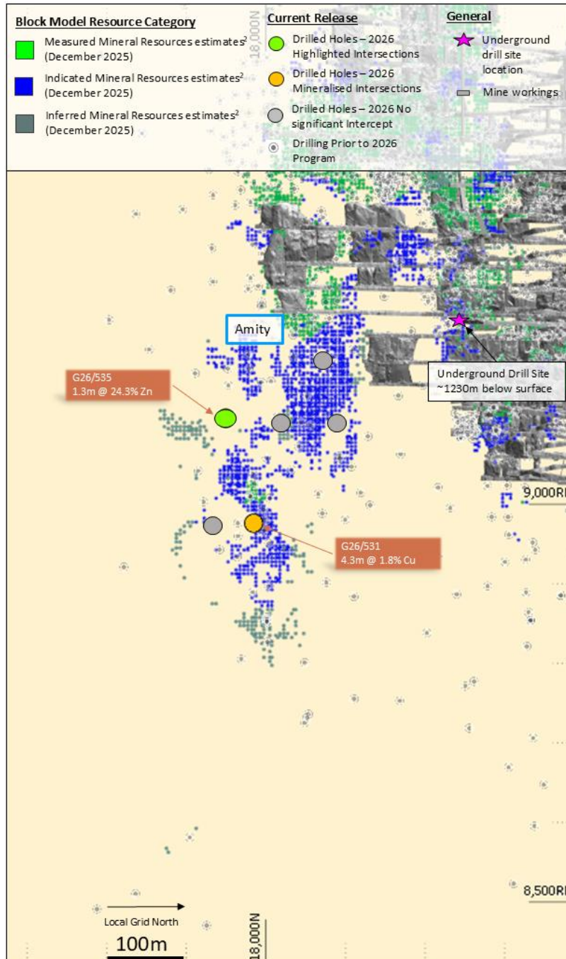
Figure 4: Long-section of Amity showing pierce points of assay results from holes reported in this release as well as the pierce points locations of historic drilling in relation to existing Mineral Resources estimates 2 and mining voids. Image is orientated to look mine grid west.
