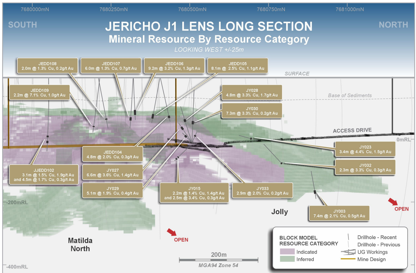
Figure 2. Jericho J1 lens long section showing Mineral Resource category (as at 31 December 2025) and recent 2026 significant intercepts reported within.
