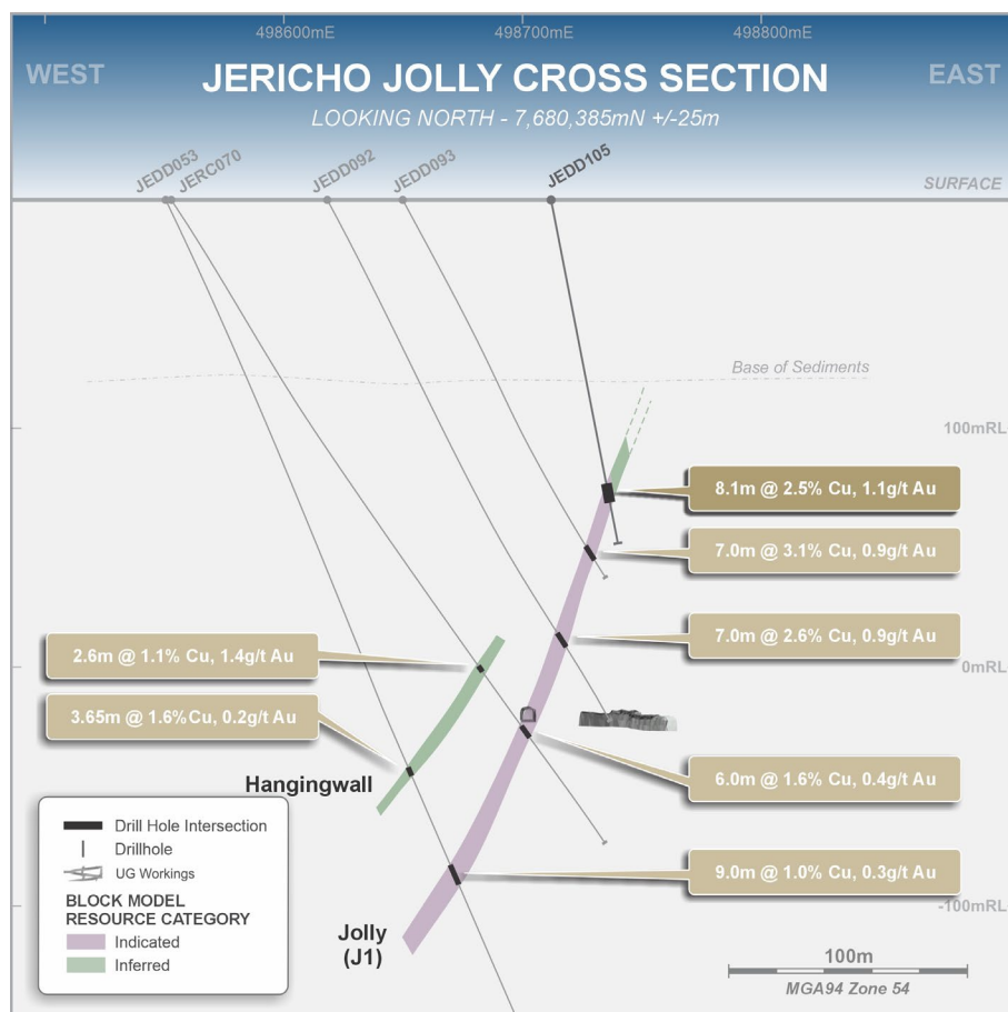
Figure 3. Jolly cross section through 7,680,385mN showing JEDD105 results.
