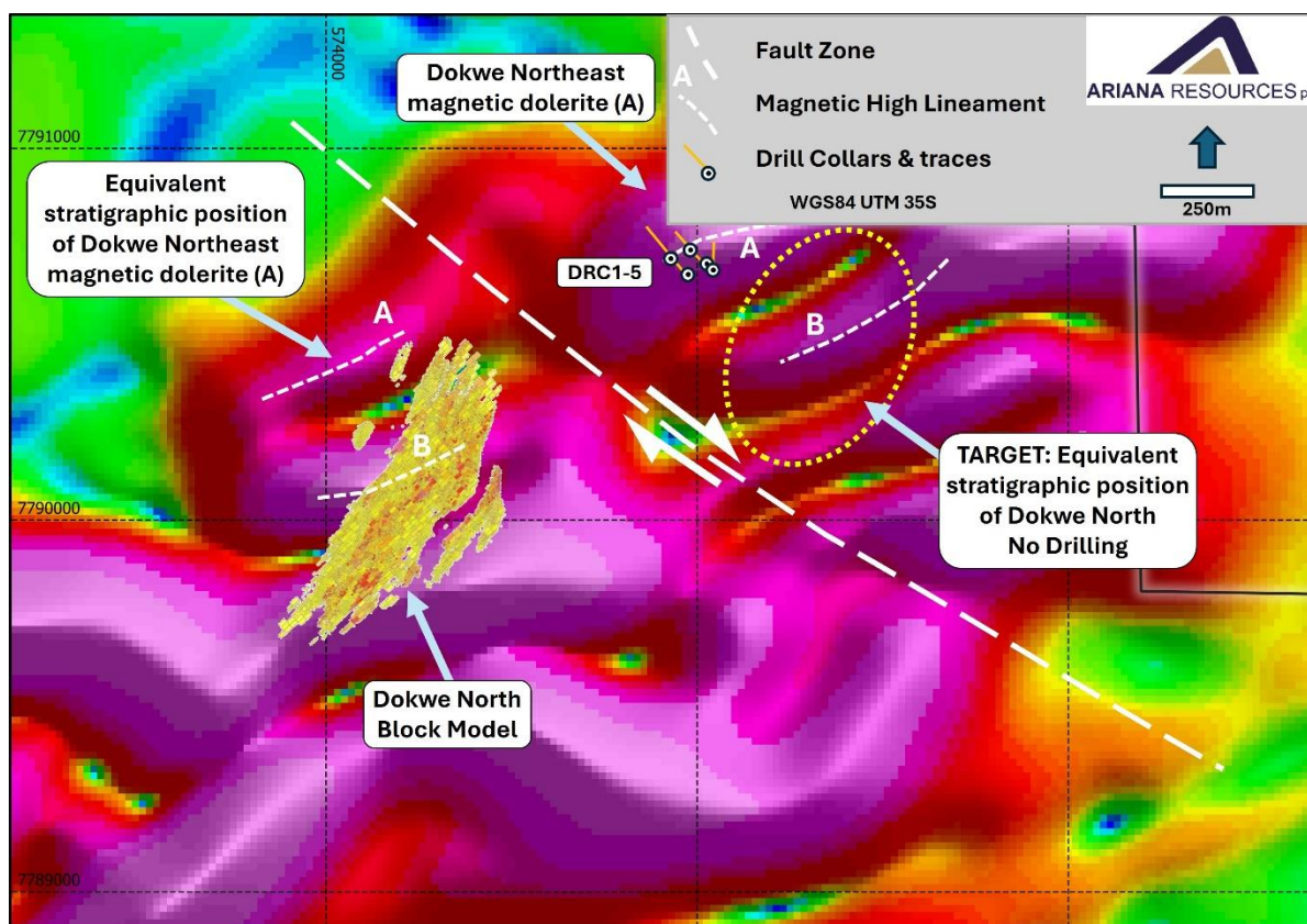
Figure 7: Aeromagnetic image showing the trace of the magnetic high (A) at Dokwe Northeast and its equivalent on the other side of the dextral fault to the north of Dokwe Central. The implication of this is that the geology hosting the Dokwe North deposit is situated just to the southeast of the original target.
