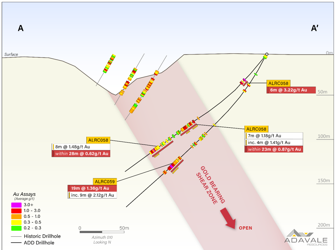
Figure 2: Cross Section Displaying position and gold results for ALRC058 and ALRC059 relative to the historic London-Victoria Open Pit (Section Line A-A' displayed in Figure 1)
