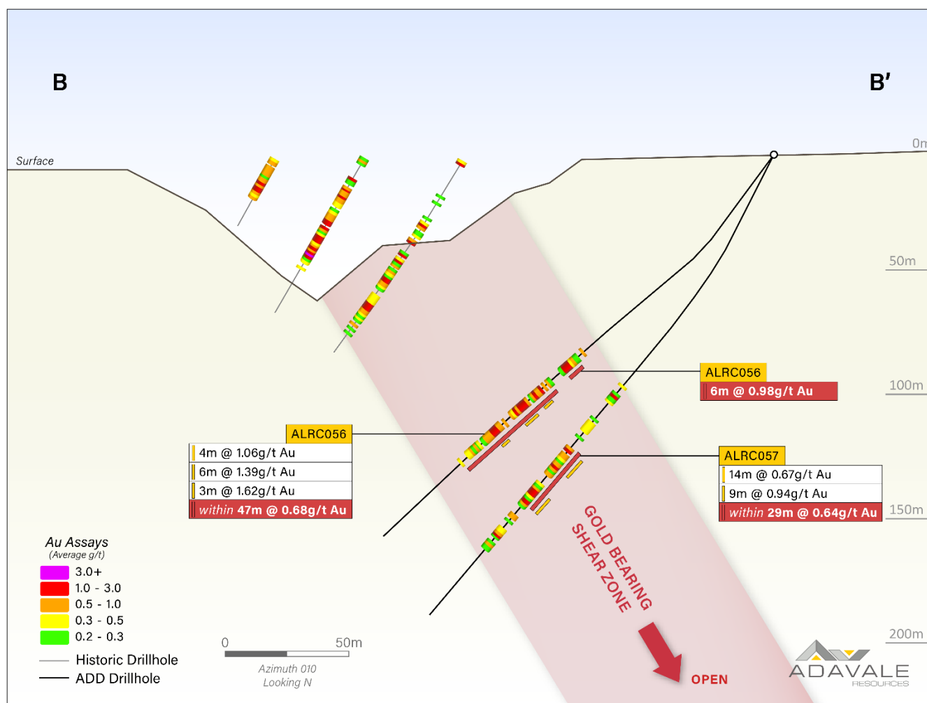
Figure 3: Cross Section Displaying position and gold results for ALRC056 and ALRC057 relative to the historic London-Victoria Open Pit (Section Line B-B' displayed in Figure 1)
