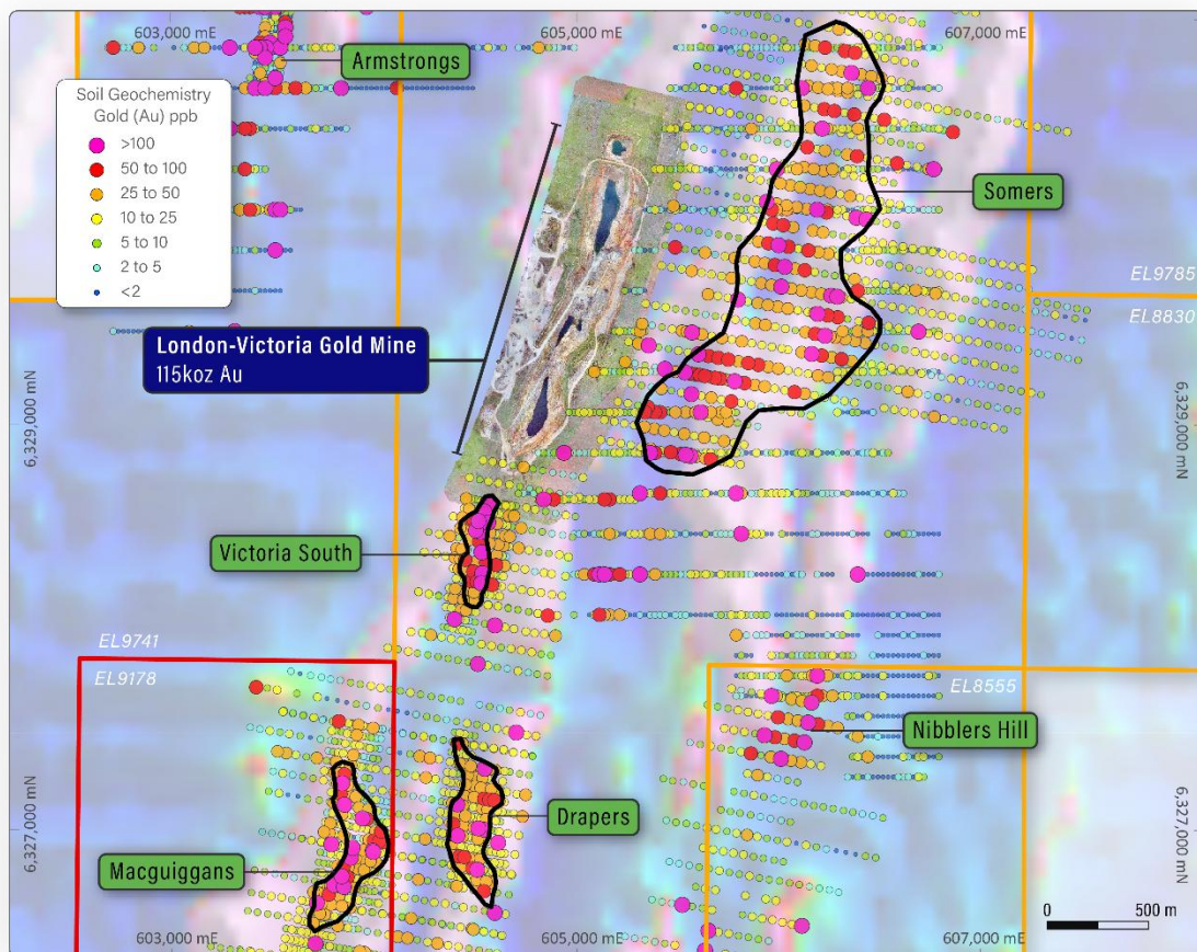
Figure 3: EL9178 On Regional Magnetics (RTP 1VD) highlighting Strike Extent of the London-Victoria Shear Zone Insert: Near Mine Gold Surface Geochemistry and Prospect Footprints
