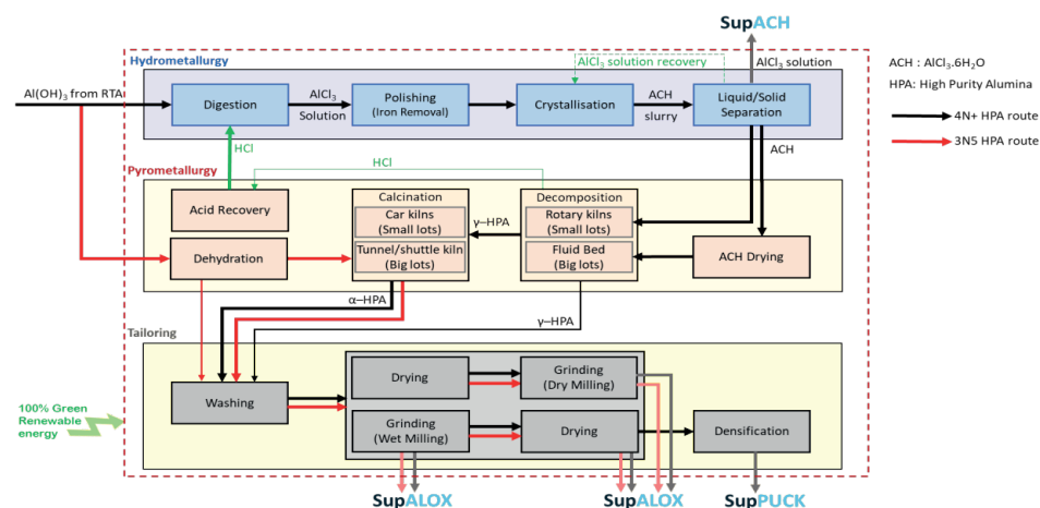
Figure 10. AEM Block Flow Diagram. (Source: AEM)
