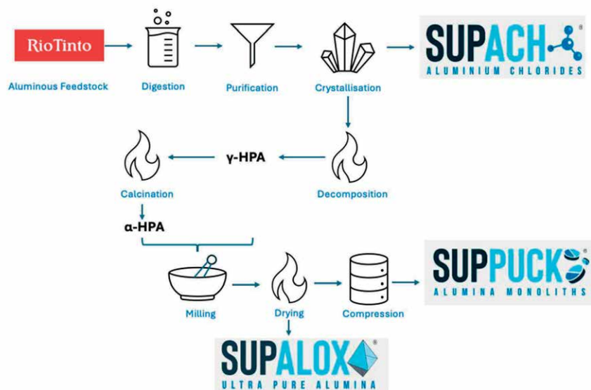
Figure 8 Chlorine Leach-CLCP
