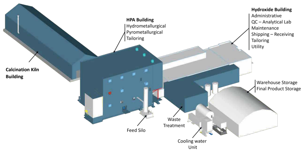
Figure 4. Building Schematic. (Source: AEM)
