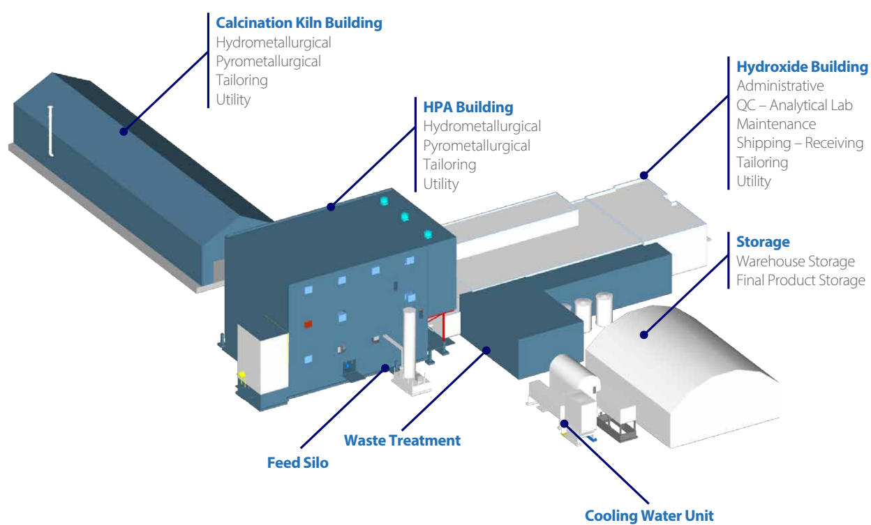
Figure 2.4: Schematic of the Cap-Chat Plant
