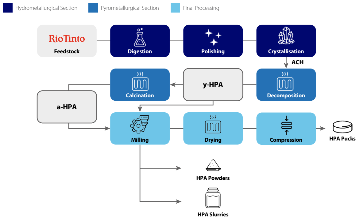
Figure 2.8: Overview of the CLCP Process
