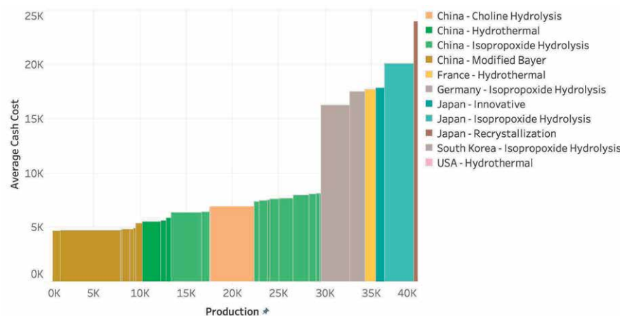
Figure 10 Global HPA Commercial Scale Production Cost Curve by Technology 2024, US$/t
