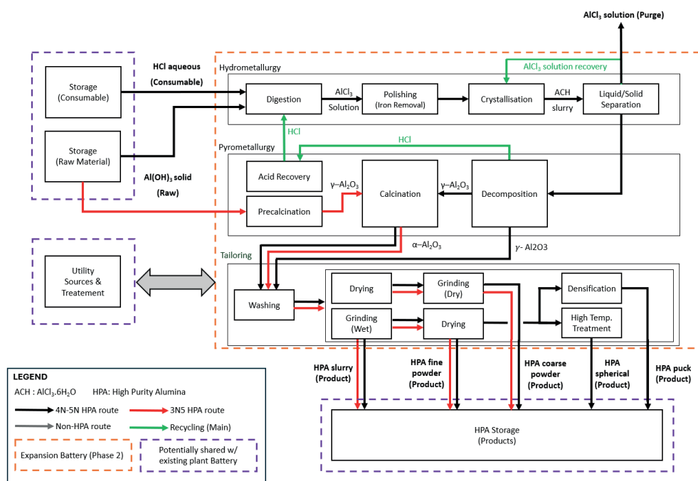
Figure 6 Project's Block Flow Diagram. (Source: AEM)
