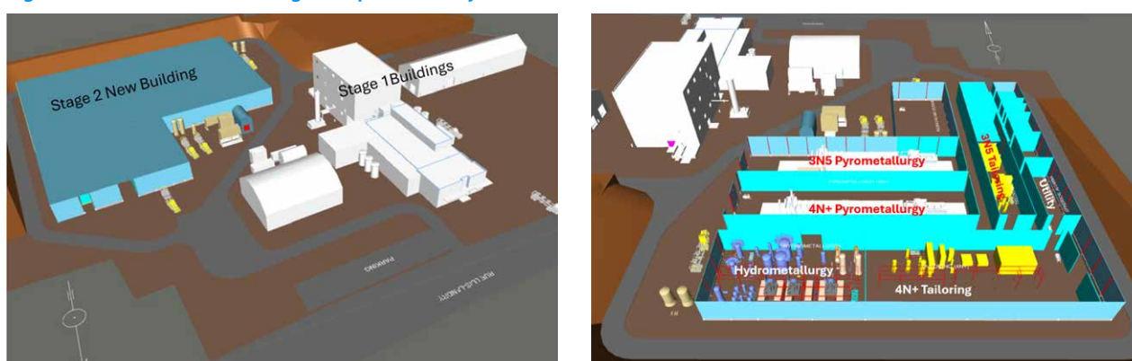
Figure 2.10: Renders of the Stage 2 Expansion Project
