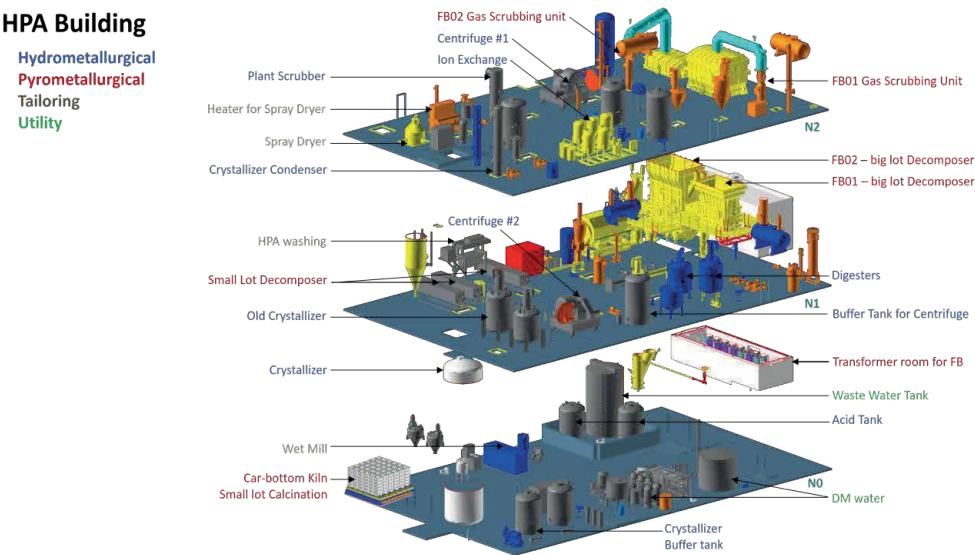
Figure 11. Exploded schematic of the unit operations in the HPA Building. (Source: AEM)
