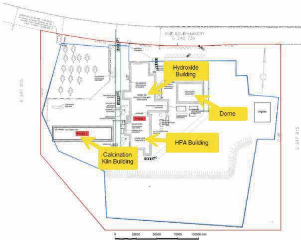
Figure 2. Layout Stage 1. (Source: AEM)
