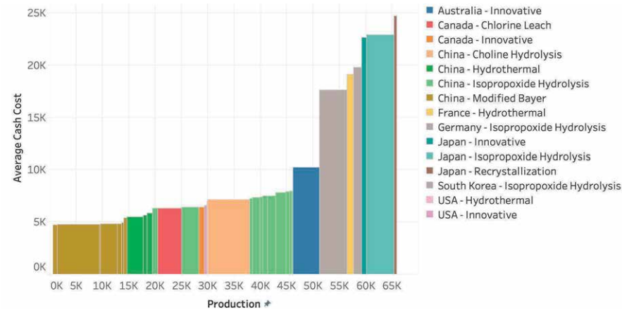
Figure 11 Forecast Global HPA Commercial Scale Production Cost Curve by Technology 2030, US$/t
