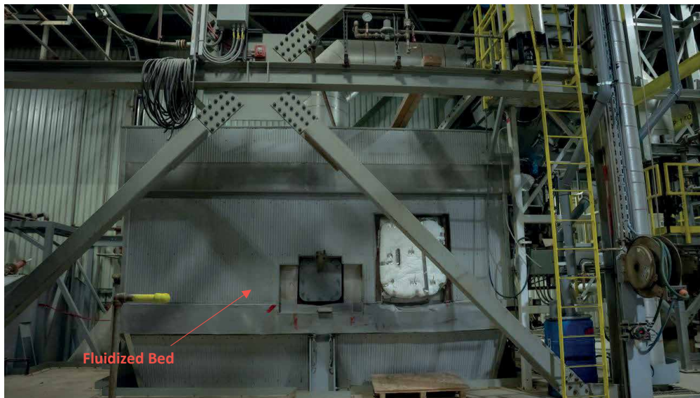
Figure 16. Decomposer #1 (FB01). (Source: AEM)
