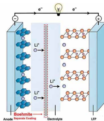
Figure 2 Application of Boehmite in LFP Batteries
