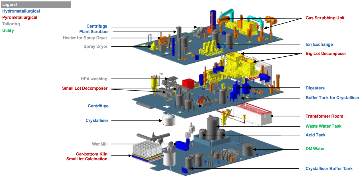
Figure 2.5: Overview of equipment currently installed in HPA Building
