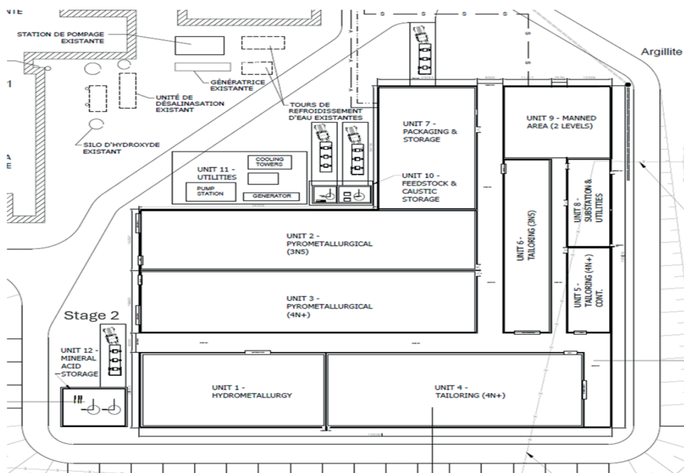
Figure 3 Layout of Functional Units. (Source: AEM)
