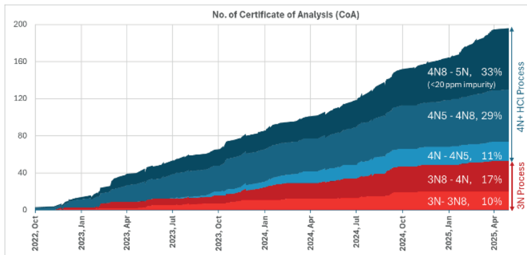
Figure 27: Purities recorded on Certificate of Analysis (CoA) since Q4 2022. (Source: AEM)
