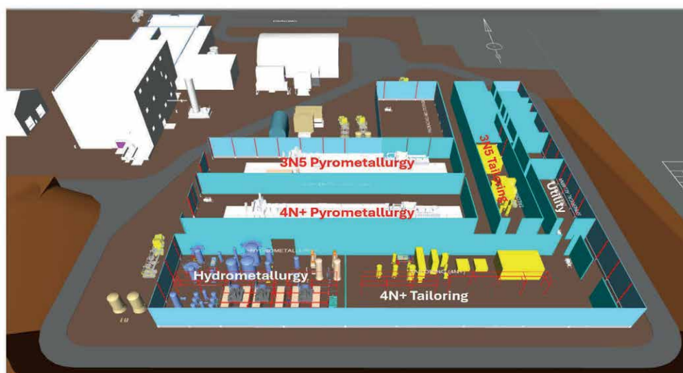
Figure 4 Equipment Layout. (Source: AEM)
