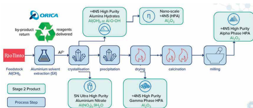
Figure 7 Solvent Extraction
