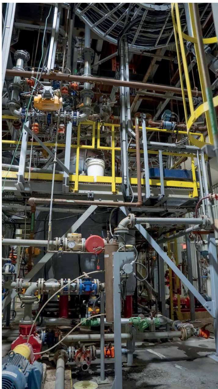
Figure 9. Digester #2 in operation. (Source: AEM)
