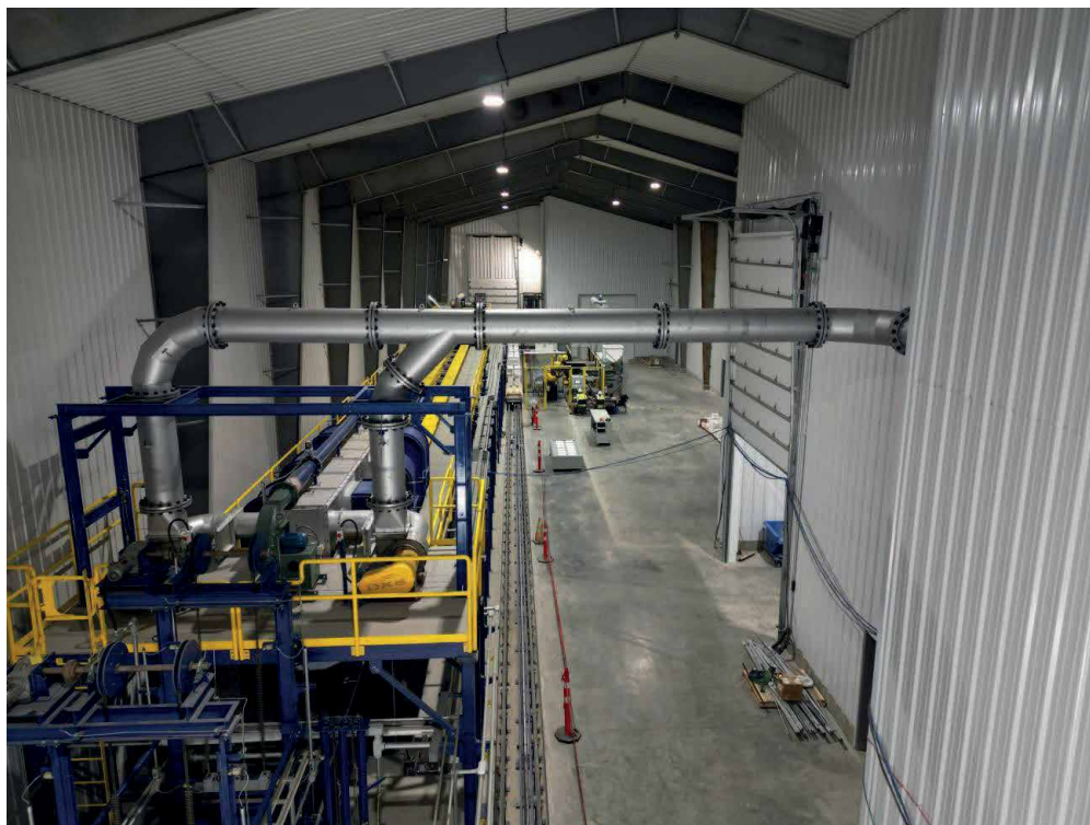
Figure 8. New Building - Tunnel Kiln. (Source: AEM)
