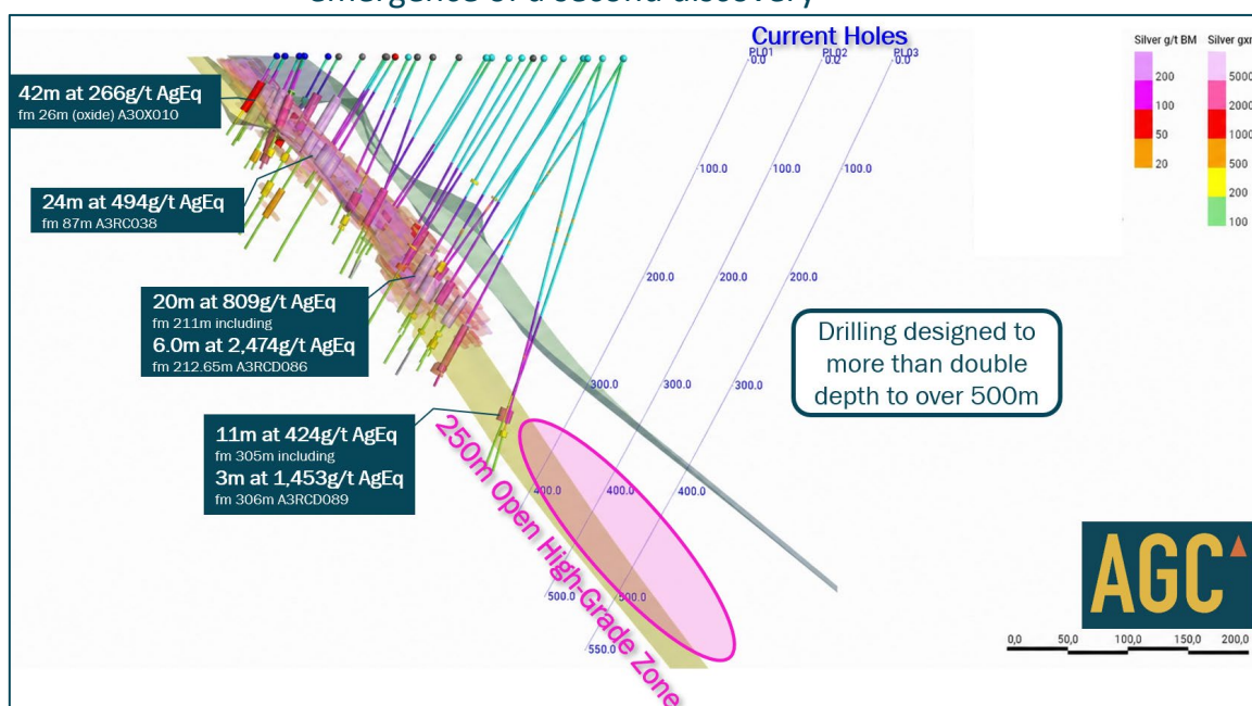
Figure 1: Achilles northern zone cross section looking north through 6,329,030N showing high grade mineralisation from surface to 250m depth.
