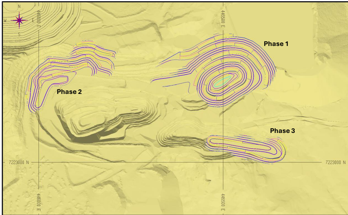
Figure 16.4: Perseverancia Operational Pits – Phases 1, 2 and 3
