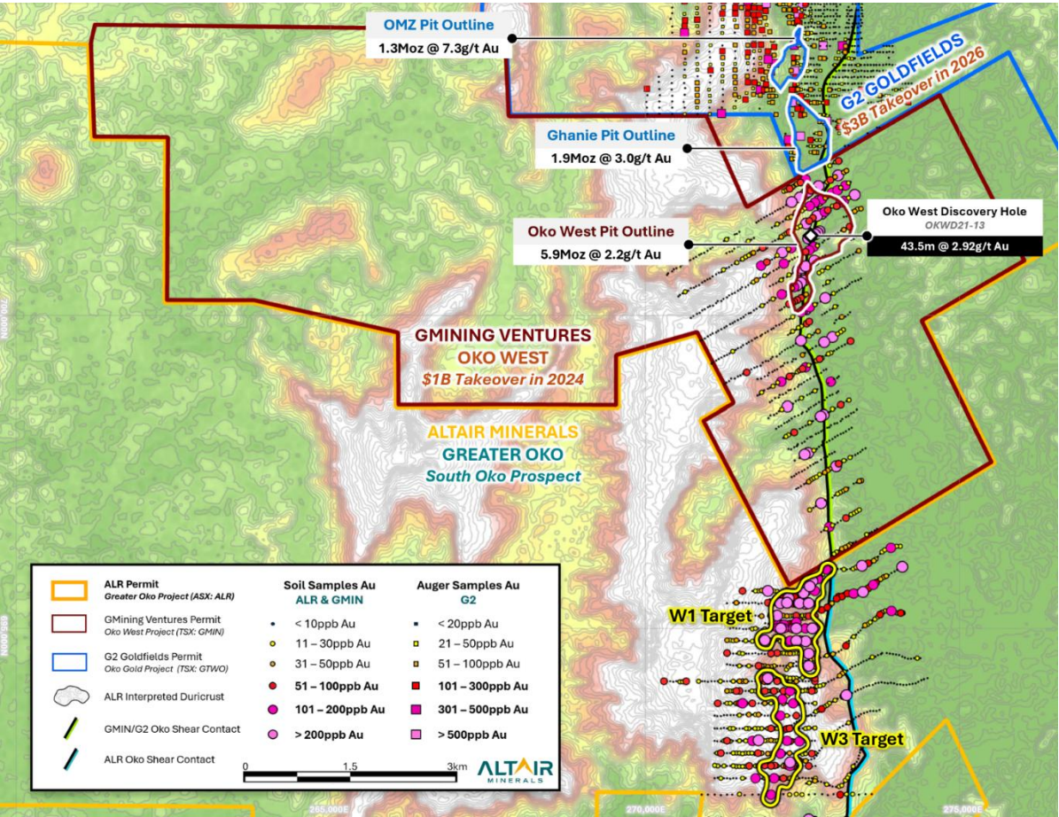
Figure 2: Plan view of Altair South Oko area, overlaid with soil sampling data for South Oko & Okos West projects and auger geochemistry at G2 Goldfields. Includes results subsequent to end of quarter. WGS84 UTM Zone 21N. 1,2,3,24,25
