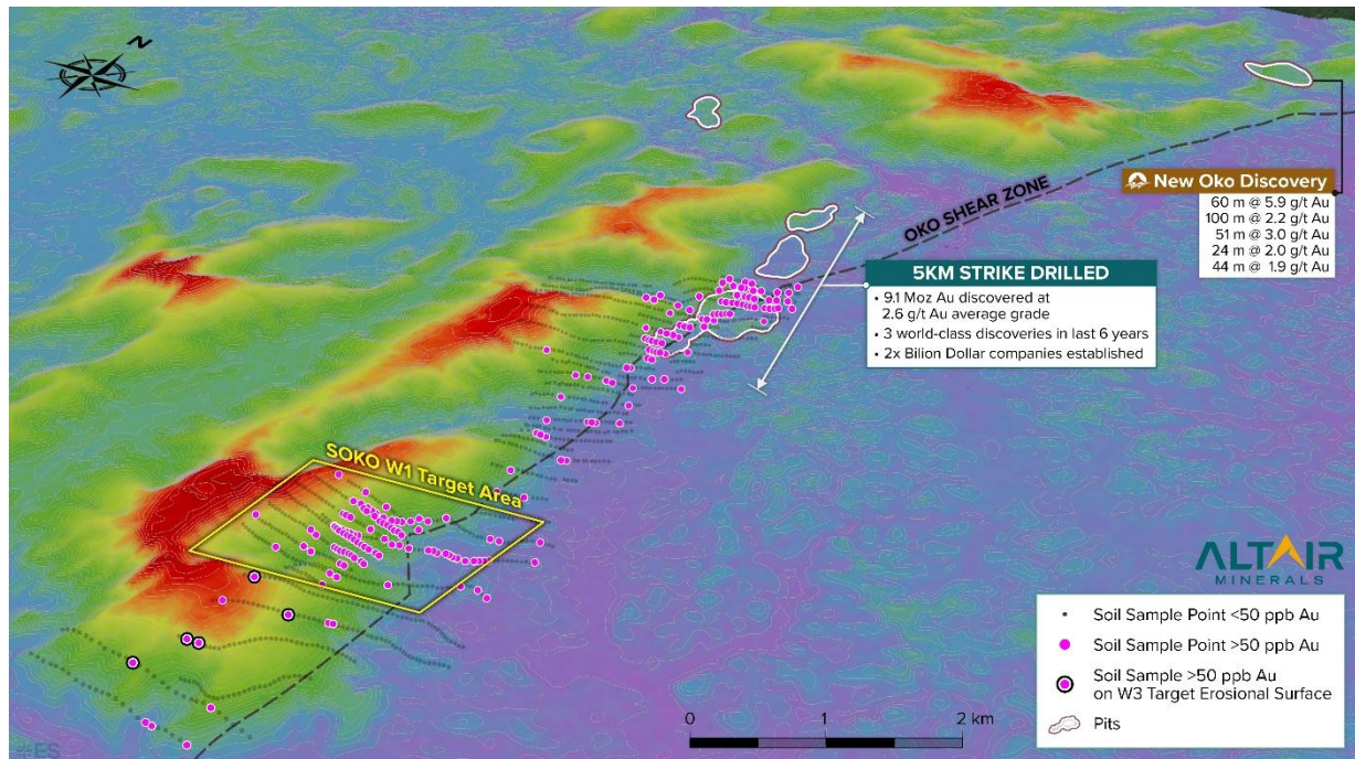
Figure 5: Topographic perspective view across the Oko region with ALR soil sample results to date alongside previously reported soil sampling program within the B-Horizon completed by GMIN. Key structural control of Oko Shear Contact shown alongside pit outlines for deposits and discoveries made across this distinct structural control. East of Oko Shear = Granitoid Oko Pluton. West of Oko Shear = Greenstone belt, seen by distinct change in topographical character. “Pits” refer to MRE Pit design outlines from PEA/FS studies conducted by neighbouring assets. Note due to 3D perspective view, scale only applies in the NE direction its orientated in. 1,2,3,4,5,9,10,11,12
