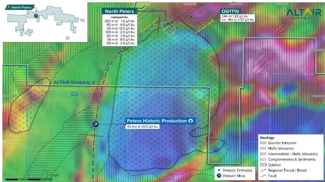
Figure 5: Geological map overlaid with aeromagnetic RTP survey of Puruni District with NP historic drilling. WGS84 UTM Zone 21N. 19,20,26
