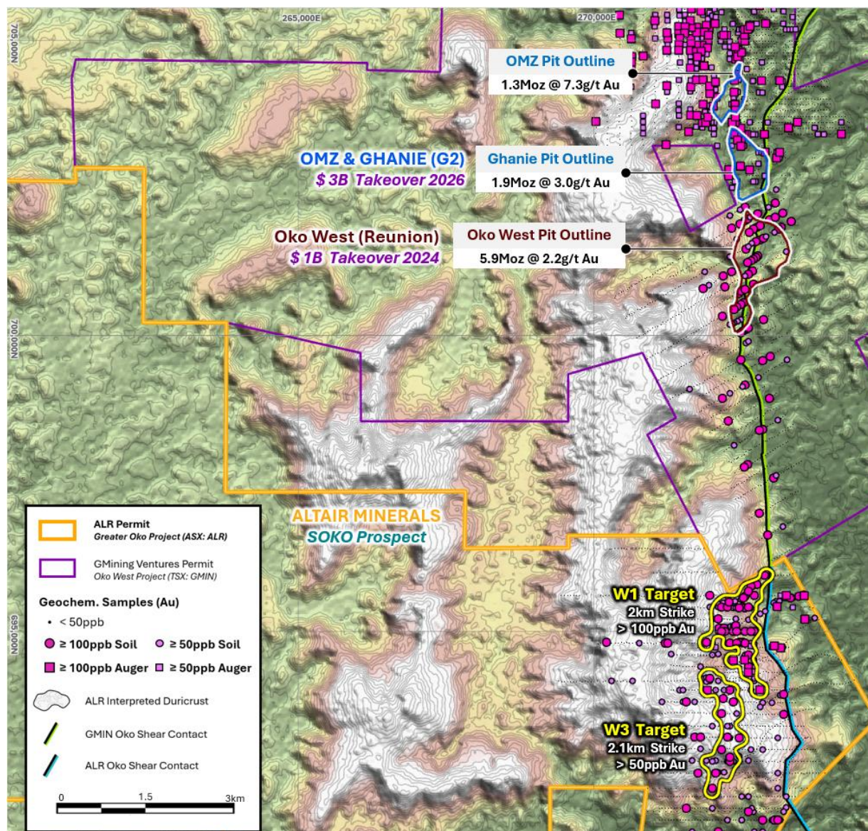
Figure 11: Plan view of Altair South Oko area in proximity to neighbouring deposits, overlaid with soil sampling data for South Oko & Okos West projects and auger geochemistry at OMZ and Ghanie. WGS84 UTM Zone 21N. 1,2,3,4,25
