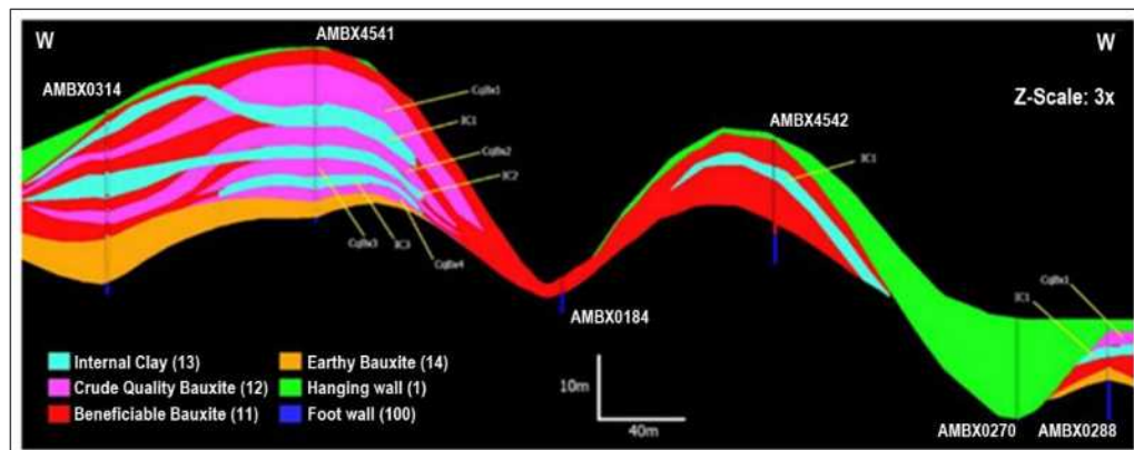
Figure 4-3: Example cross section of bauxite-bearing laterite profile at the Amargosa Project
