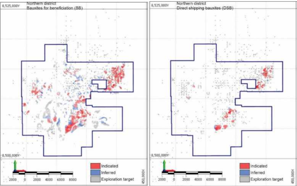
Figure 6-10: Mineral Resource classification for Northern District (source: based on SLR initial data, 2026) Source: ERM based on SLR data 2026
