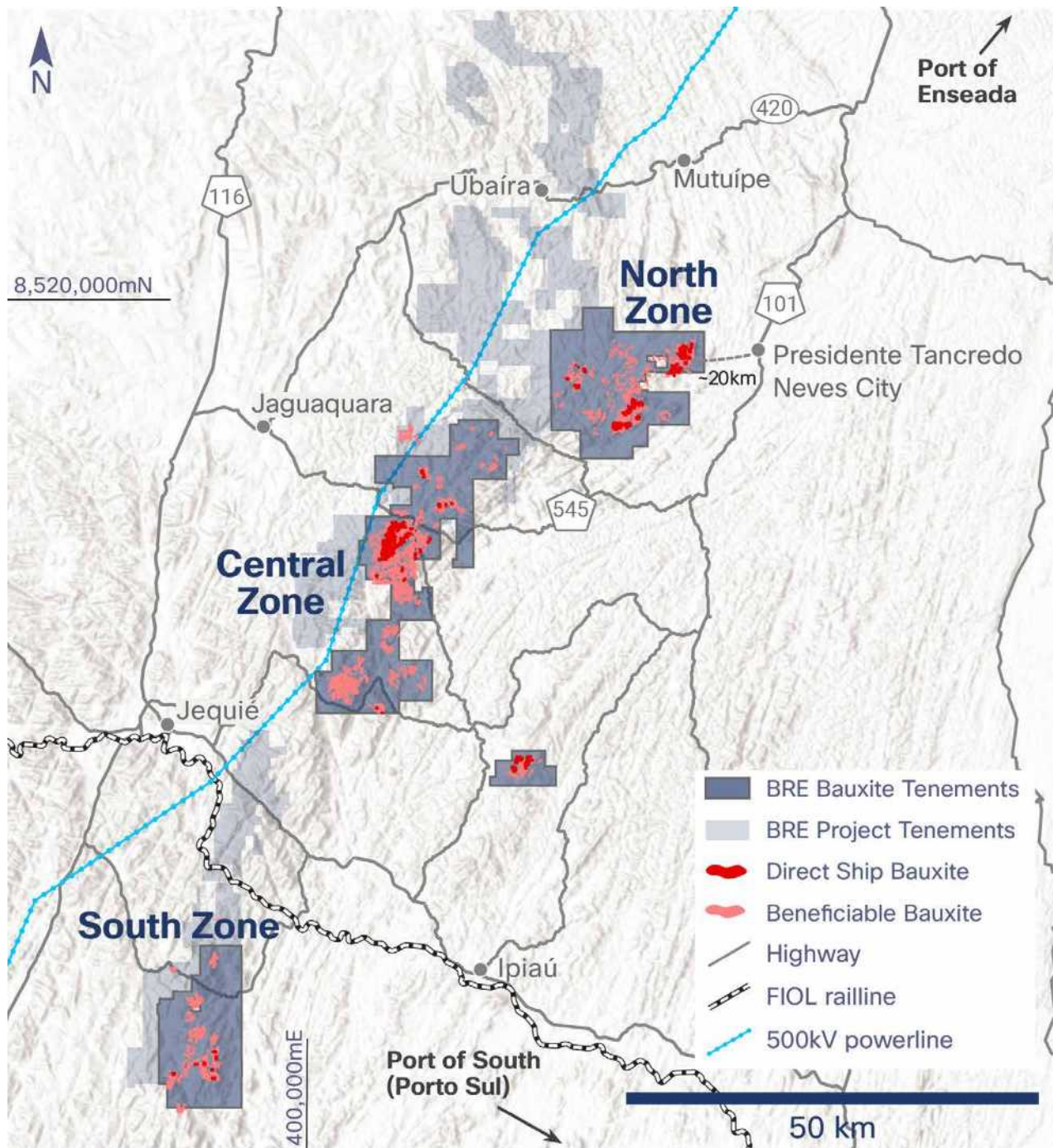
Figure 9: Distribution of DSB and BB Bauxite at the Amargosa Project
