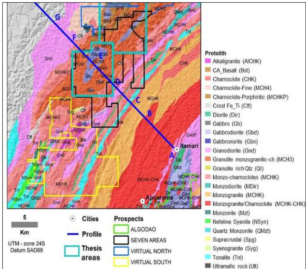
Figure 4-7: Central District Geology Map
