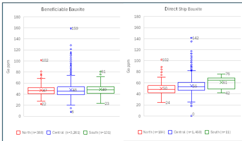
Figure 5-13: Gallium ppm boxplot by mineralised domain
