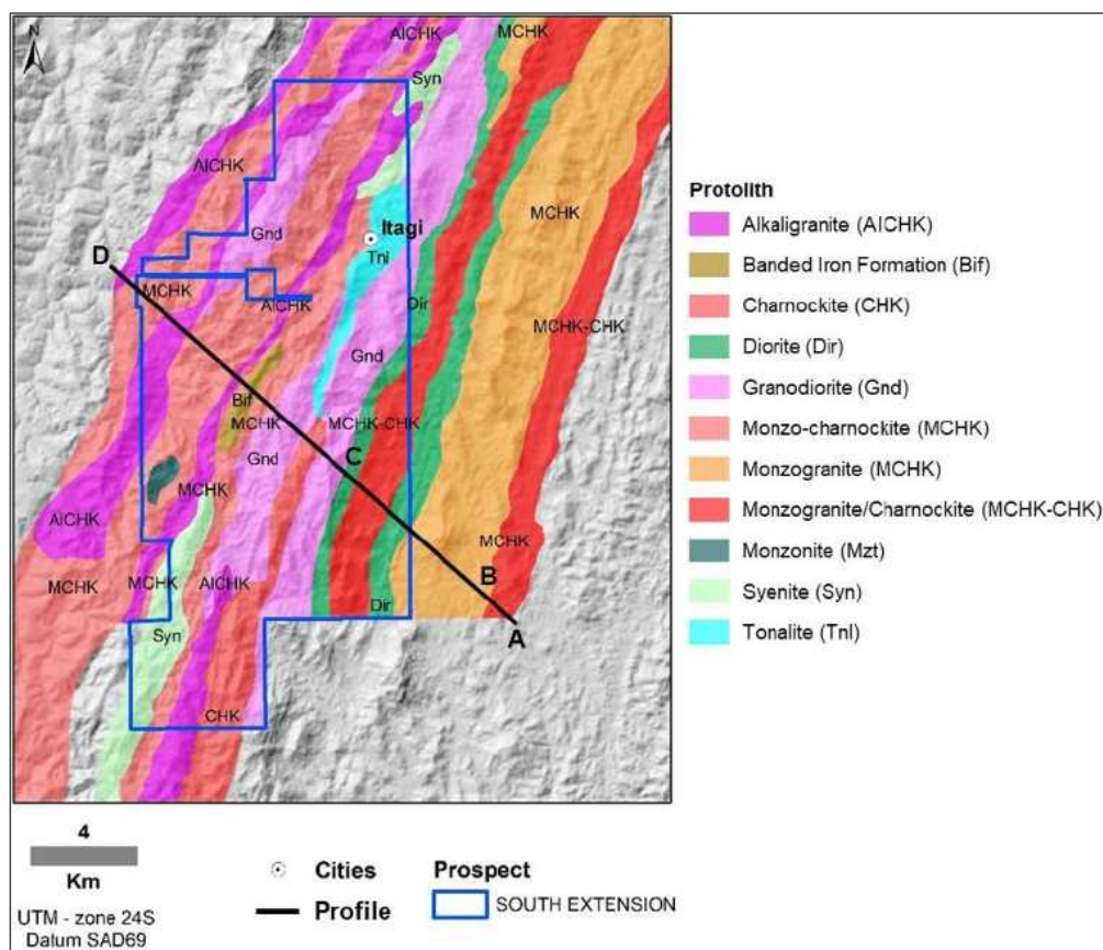
Figure 4-8: South District Geology Map
