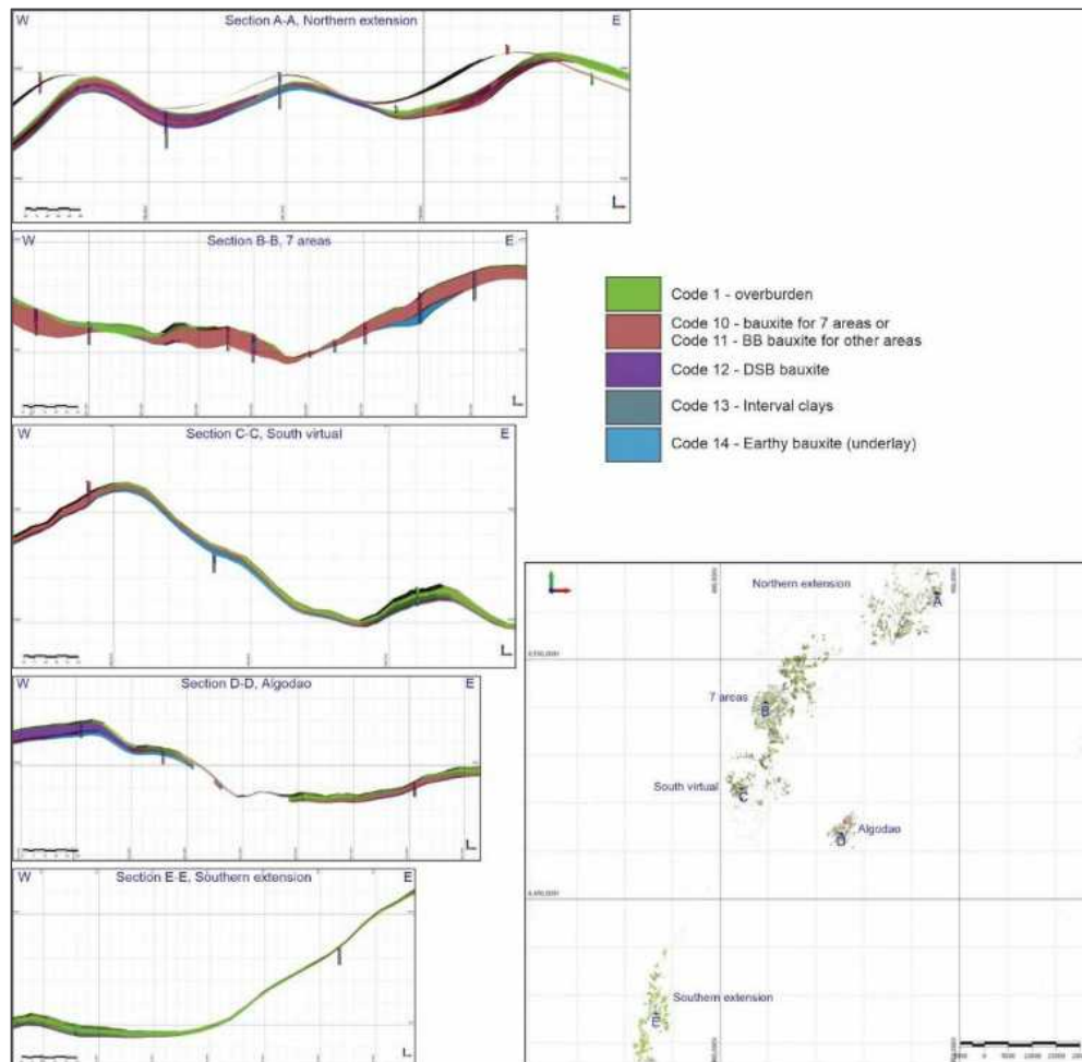
Figure 6-4: Example of cross-sections through the bauxite-bearing laterite profiles
