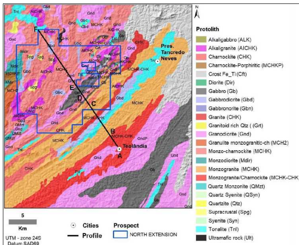
Figure 4-6: North District Geology Map
