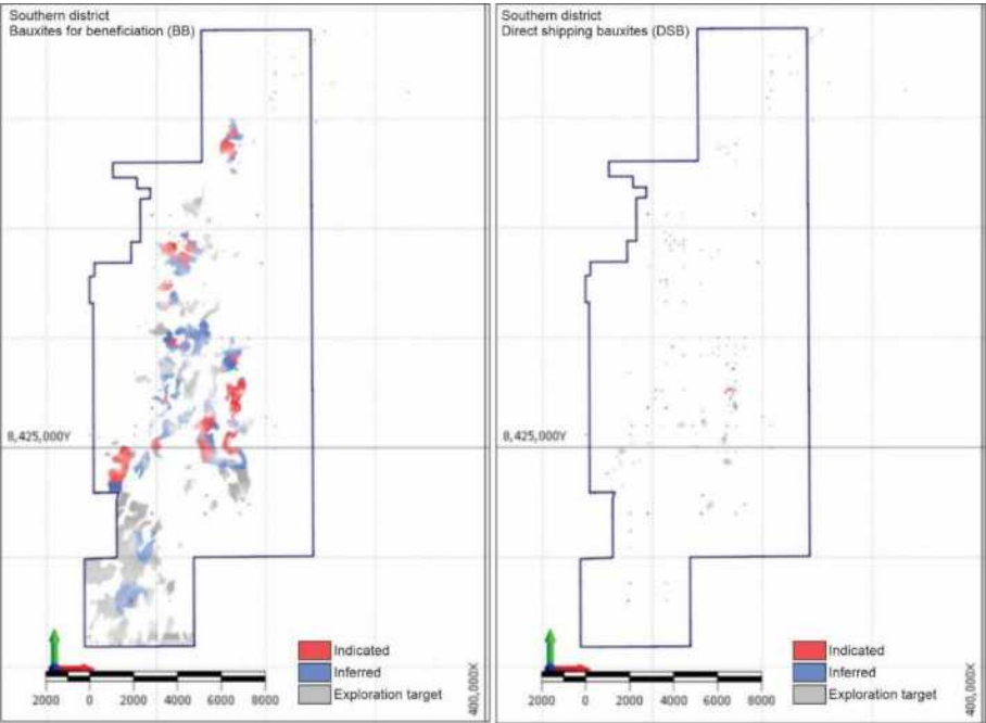
Figure 6-11: Mineral Resource classification for Southern District (source: based on SLR initial data, 2026) Source: ERM based on SLR data 2026
