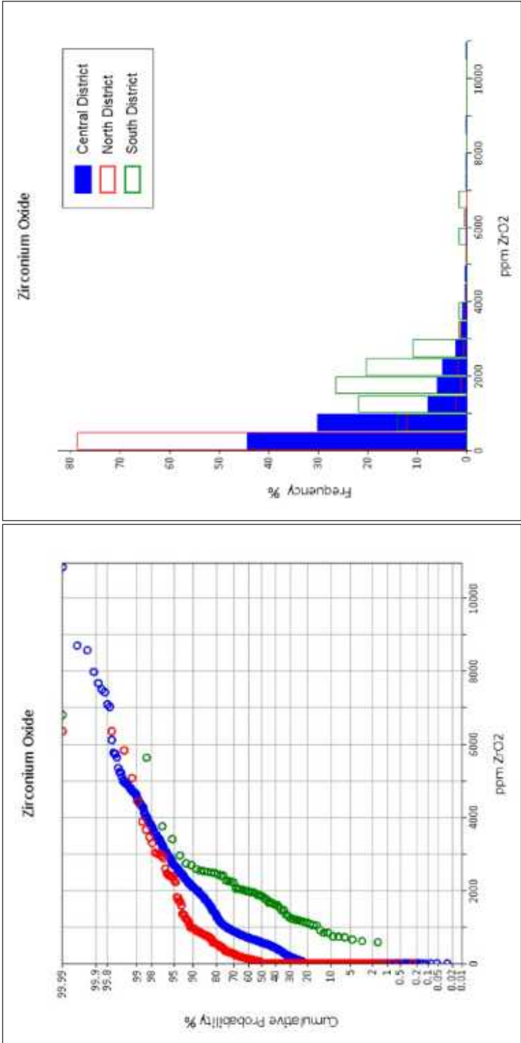
Figure 8-3: Histogram and Probability Plot of ZrO 2 (ppm) Assay Grades in Beneficiable Bauxite, 2025 MRE Source: BRE, 2026
