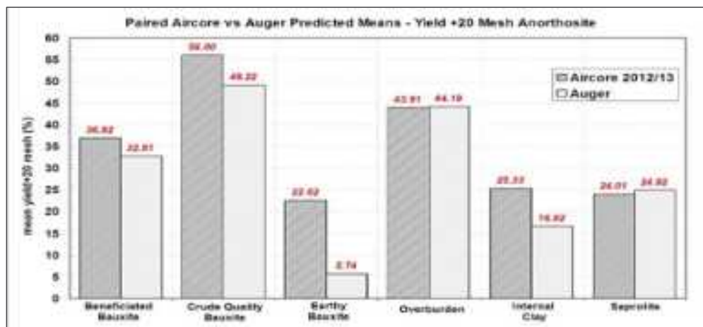
Figure 5-10: Predicted +20 mesh Minzone mean yields from regression model in twin holes
