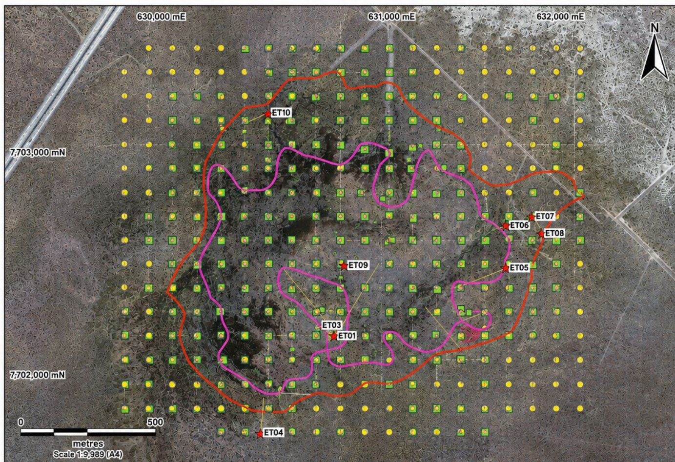
Figure 4-2 | SURFACE SAMPLING (TREO) CARBONATITE – 100 m GRID
