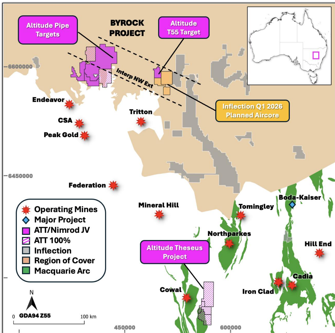
Figure 2 Location map showing Altitudes Pipe Targets, T55 Target and tenements relative to Inflection Resources Boorara, Colossal and Bugwah prospects for planned aircore drilling in Q1, 2026, in northern New South Wales and Inflections AngloGold partnered projects. The location of the Macquarie Arc and Post Mineral cover has been outlined with reference to operating mines and major exploration projects from NSW Government websites.
