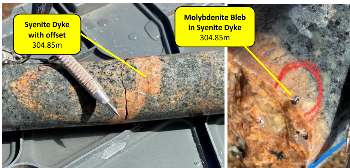
Figure 3 Molybdenite-bearing syenite dyke (with structural offset), crosscutting monzodiorite intrusion at the T55 Target, Byrock Project at a depth of 304.85m. Molybdenite is suitable for Re-Os age dating.
