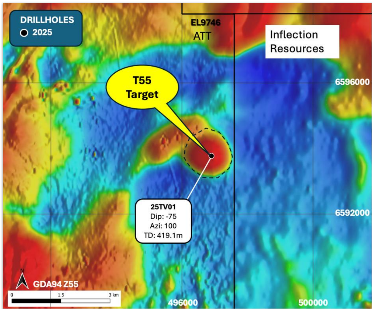
Figure 1 The T55 Target, Byrock Project - drill tested with mud rotary and diamond core drilling in December 2025 - prospectively a porphyry system. Background image Company 0.5VD RTP magnetics (ASX 7/5/2025). No previous historical drilling is recorded on this tenement.
