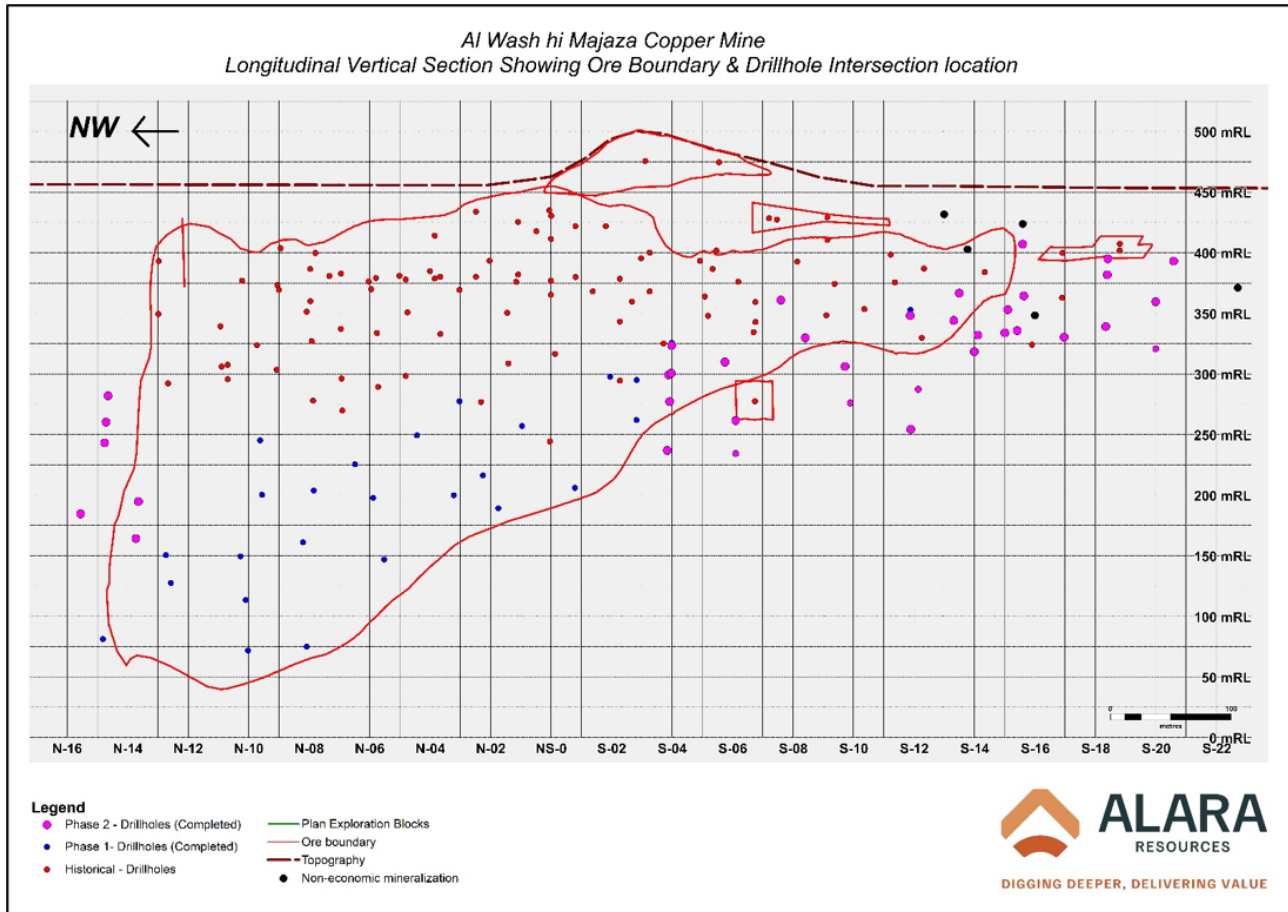
Figure 21 - Diamond Drill Holes completed in Phase 1 and 2
