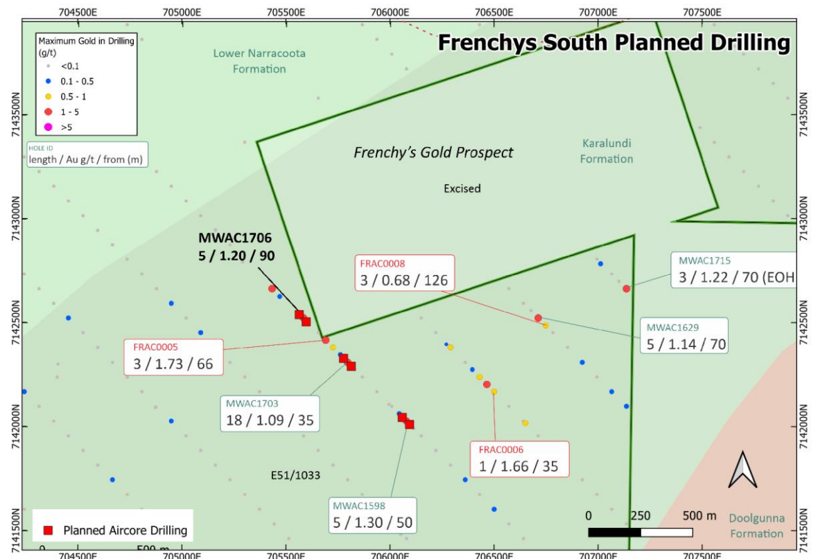
Figure 3: Frenchy's South Prospect Drilling Plan (ASX Announcement 8 August 2023 for previous results)
