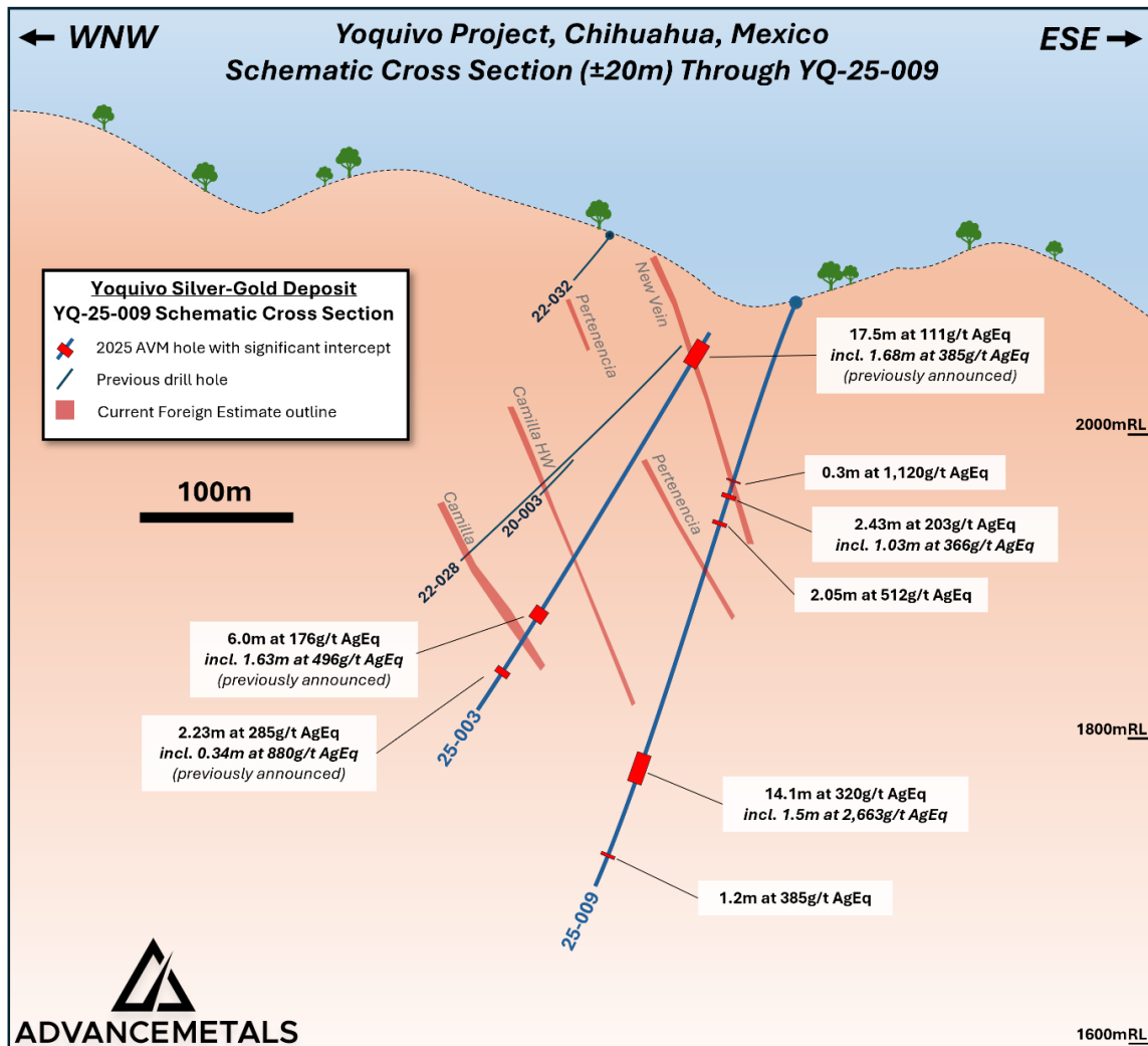
Figure 4. Schematic cross section (±20m, looking north-northeast) showing previous drilling and the approximate outline of the existing Foreign Estimate 4 , along with significant down hole intersections for YQ-25-009 (see Table 1 & 2 for full details).
