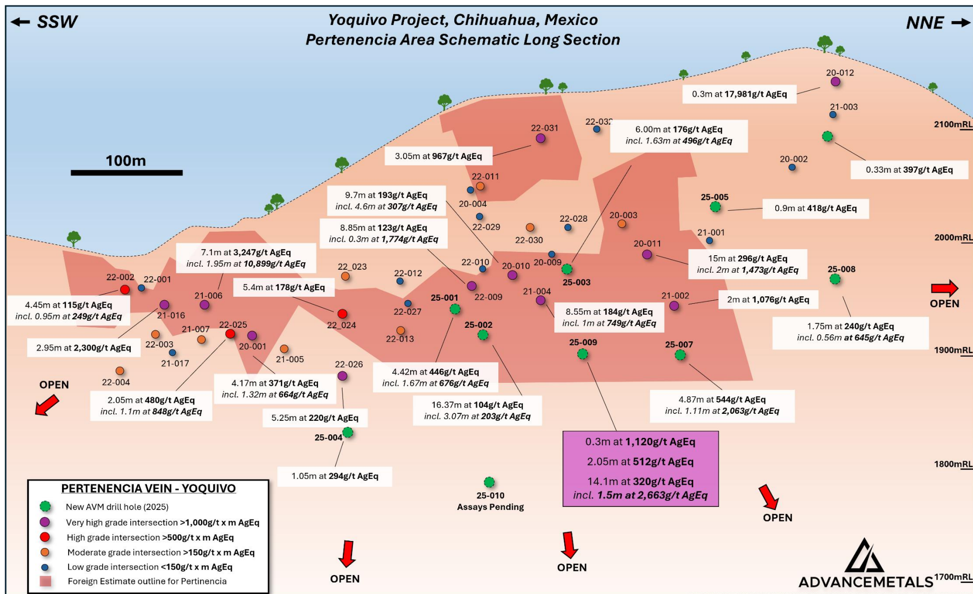
Figure 3. Schematic long section showing previous drill intersections at Pertenencia 2 , colour-coded by silver-equivalent 1 multiplied by down hole interval (g/t x m AgEq 1 ). Selected intersections are also highlighted on the long section, as is the current Foreign Estimate outline 1,4 . Drill holes YQ-25-009 and YQ-25-010 were recently completed at Pertenencia, with the later having assays pending.
