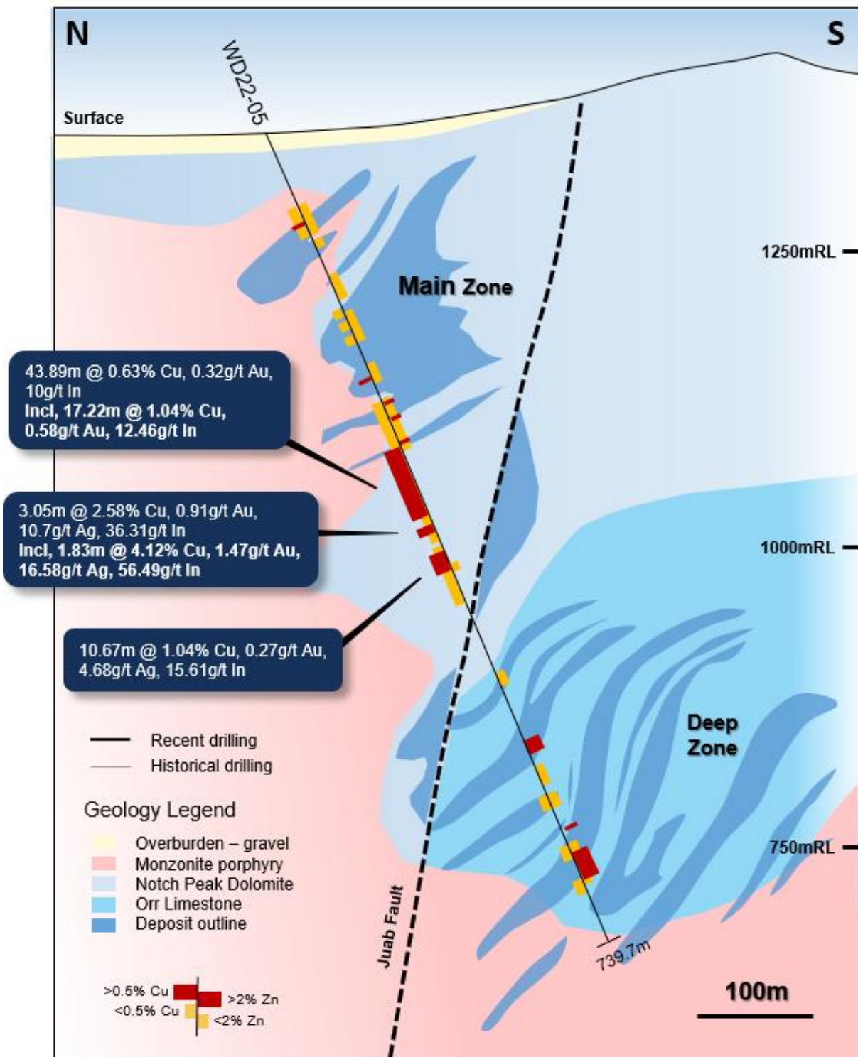
Figure 5: Schematic geological section of the West Desert Deposit at 288810E looking east showing an example of the intersections of copper-gold dominant mineralisation located outside of the current resource envelope (darker blue).
