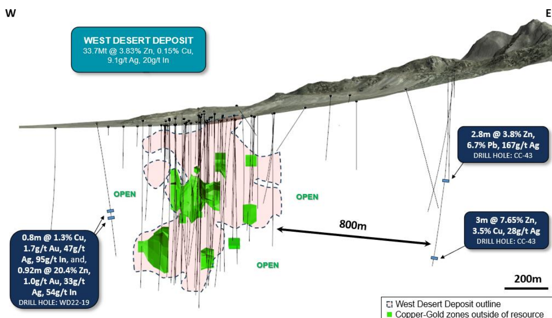
Figure 3: Schematic Long section of the West Desert Deposit area looking north, showing the Cu-Au-Ag-In-Ga zones identified by drilling (green), superimposed on current resource outline (off-section and black dotted).
