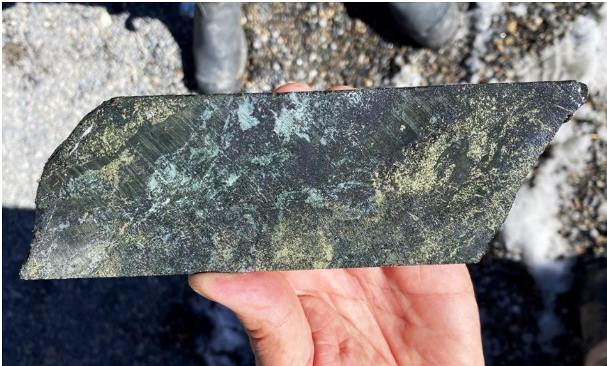
Figure 1: Cu-Au-Ag-In-Ga rich mineralisation in drill core from approximately 422m (1,385ft) downhole in WD22-01c (see Table 8 for interval details).
