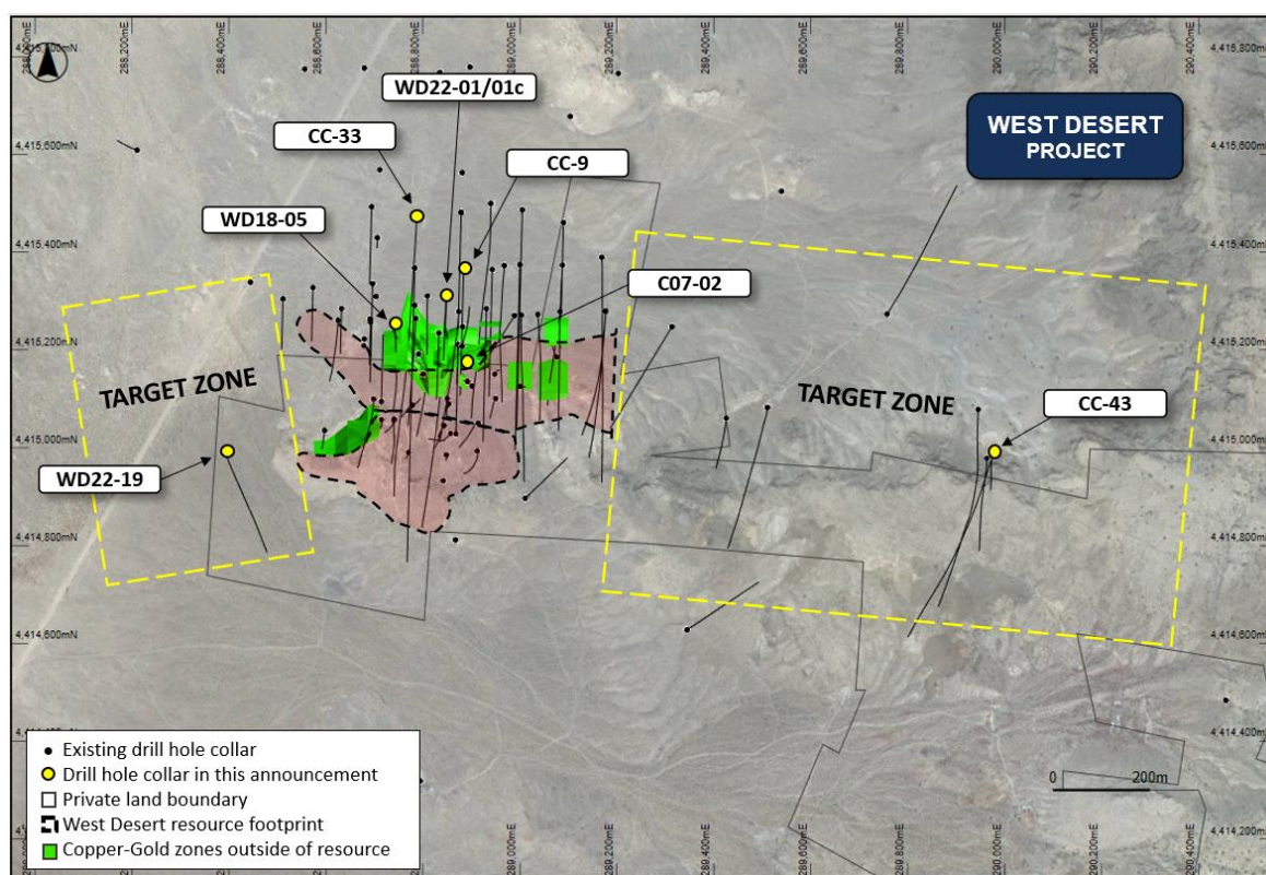
Figure 4: Plan view of the West Desert Deposit area overlaying topography.
