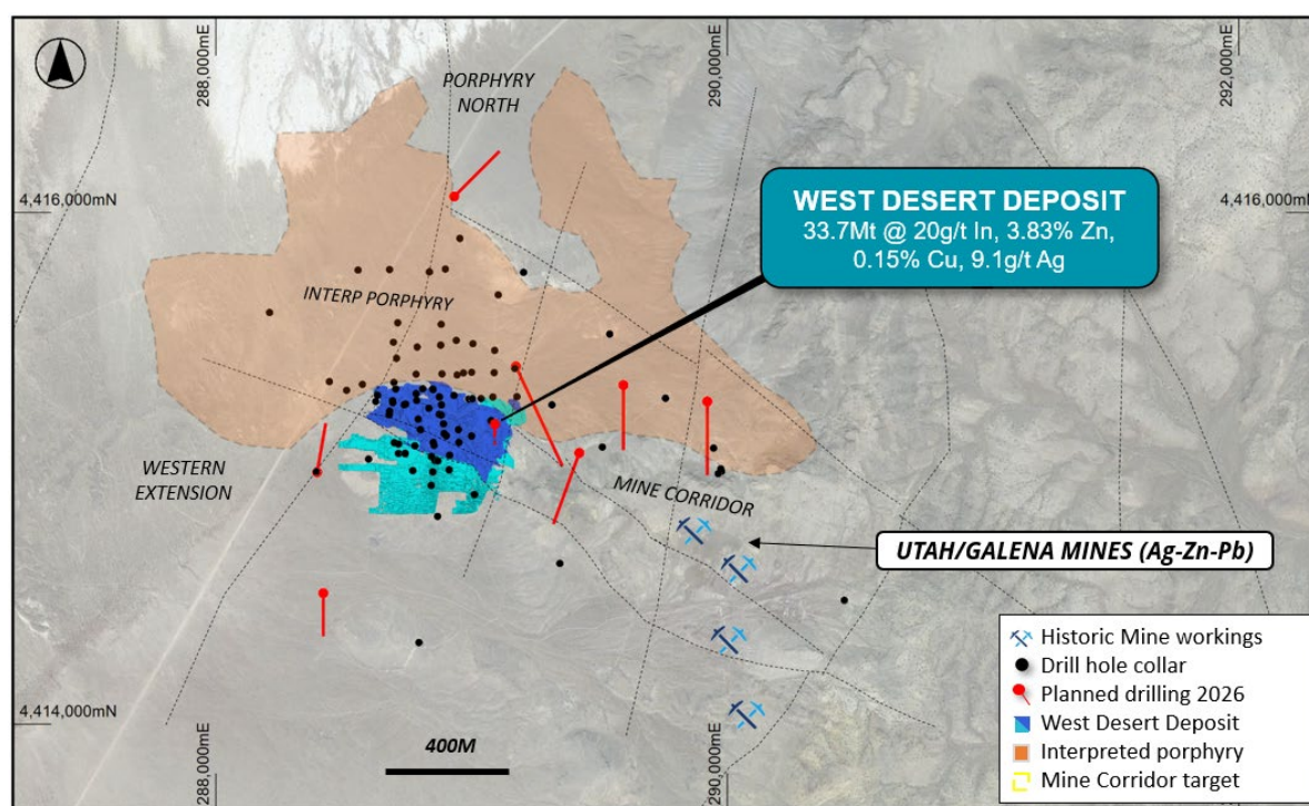
Figure 3: Plan view of the West Desert Deposit area overlaying topography.
