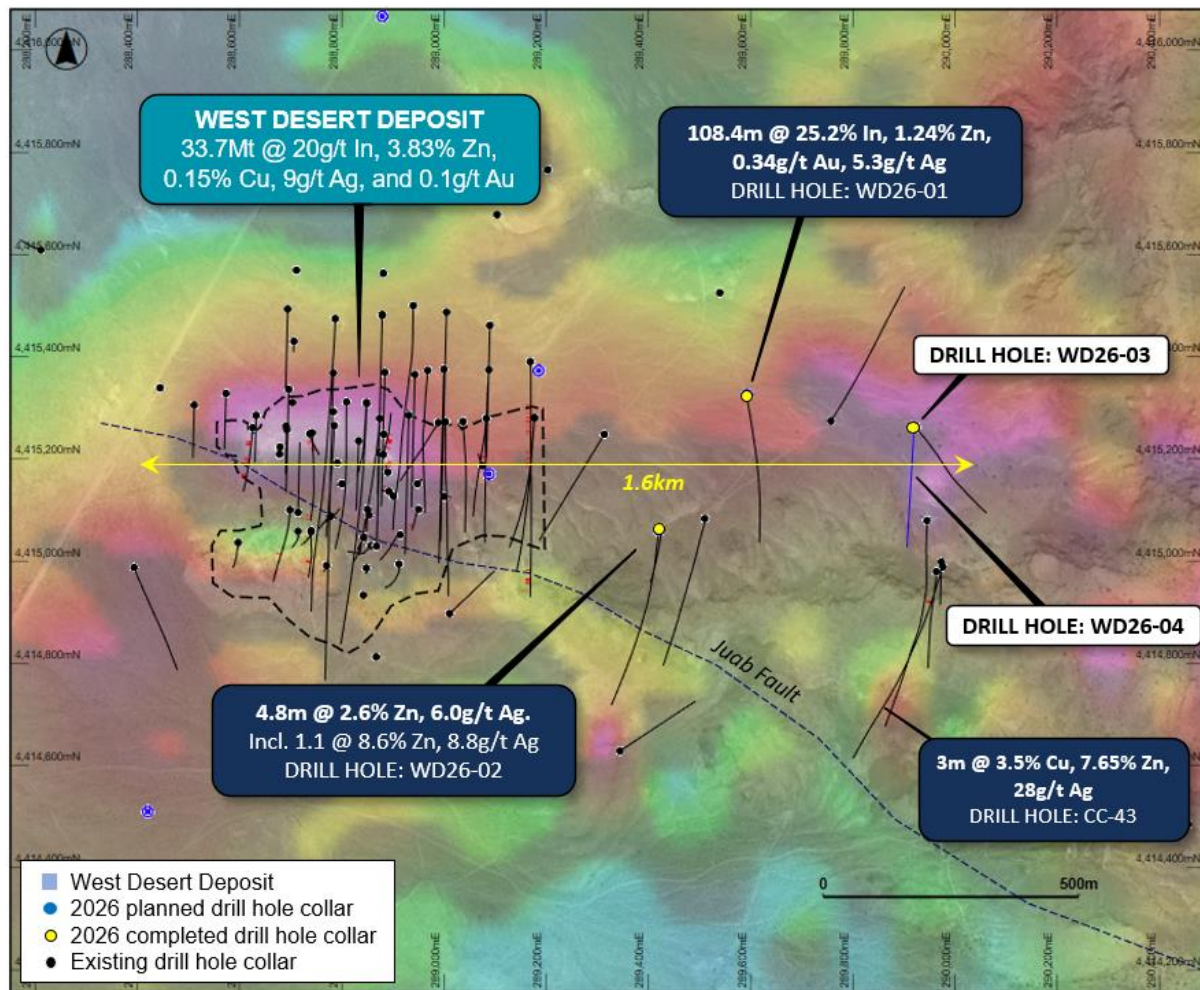
Figure 5: Plan view of the West Desert Project area, existing drilling and deposit outline overlaying magnetic imagery (1VD RTP Tilt- hotter colours represent higher magnetic intensity).
