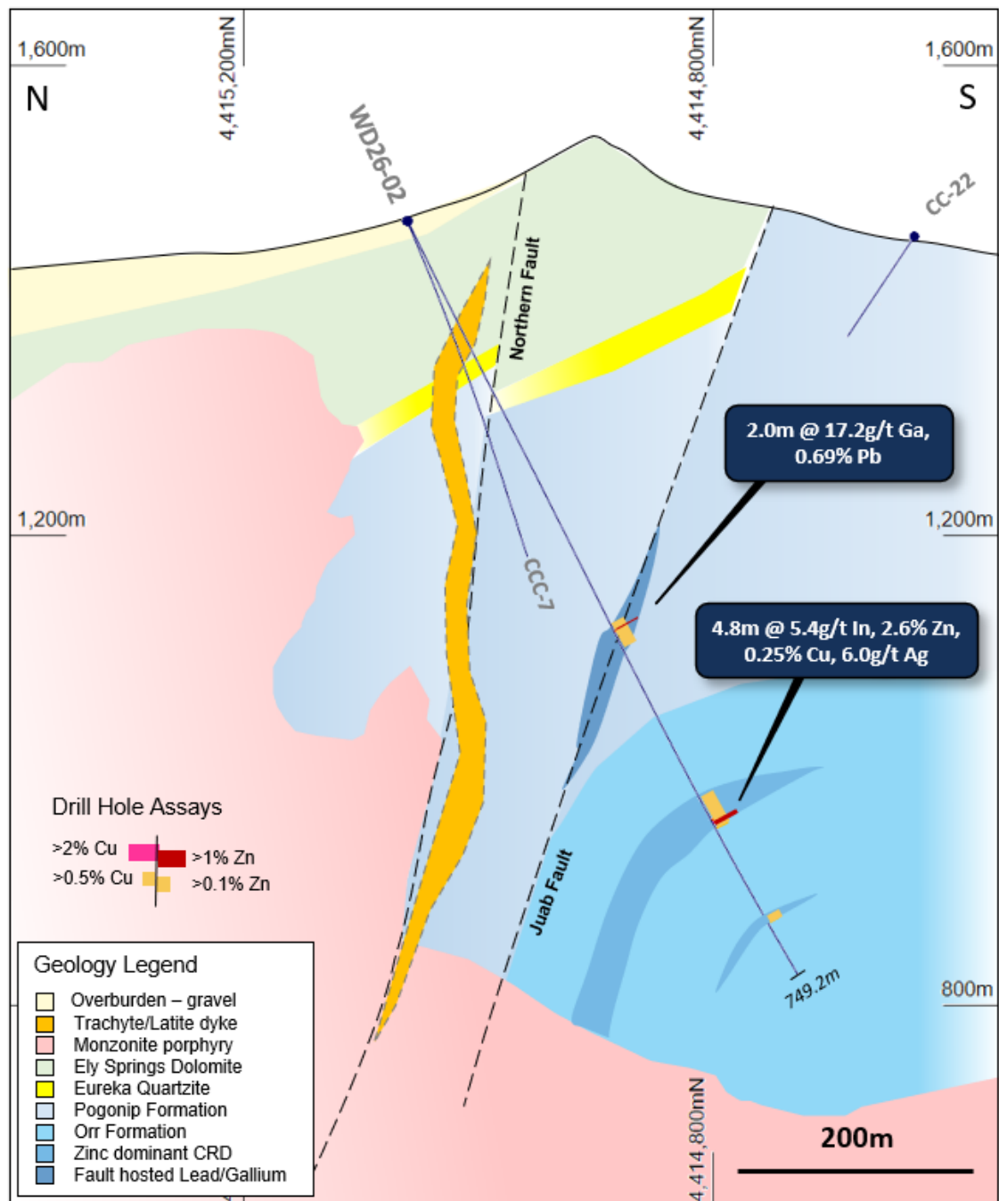
Figure 6: Schematic geological section at 289,380E (+/-50m) showing main geological units and WD26-02 drill trace.
