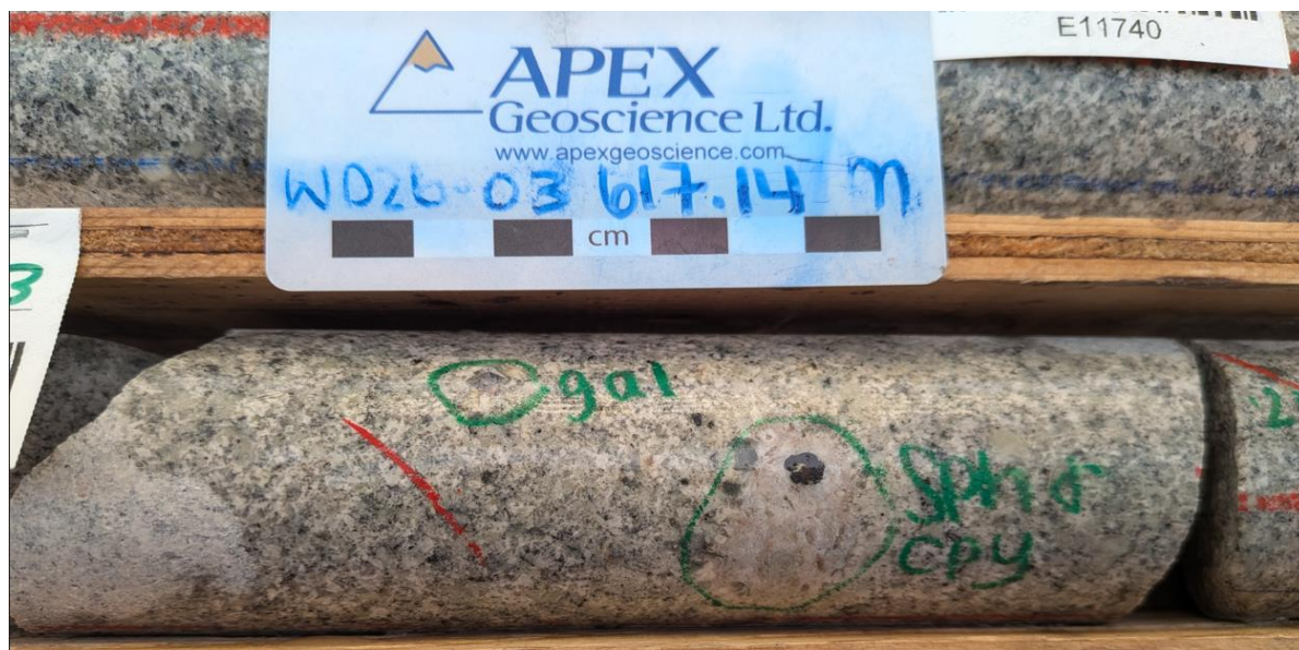
Figure 3: Weakly altered endo-skarn with visual sphalerite, chalcopyrite, and galena in NQ drill core from approximately 617.14m downhole in drill hole WD26-03. Laboratory assays for this interval are pending.
