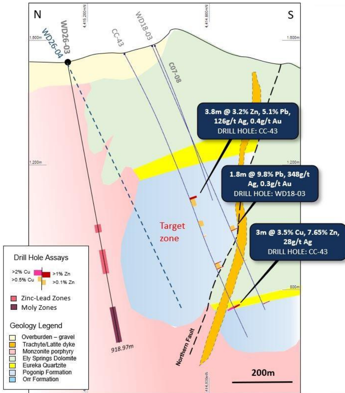
Figure 4: Schematic geological section at 289,940E (+/-150m) showing main geological units and drilling. A simplification of the mineralised intervals in WD26-03 is shown.
