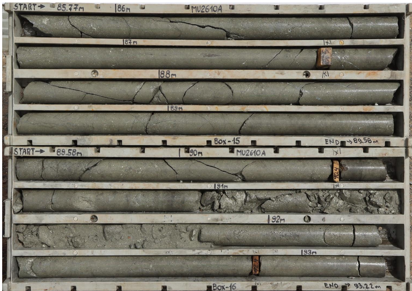
Photo 1. Massive sulphide mineralisation, drillhole MU2610A, boxes 15-16 (85.77 to 93.22 m). Visual estimates of mineral abundance are provided in Table 1.
