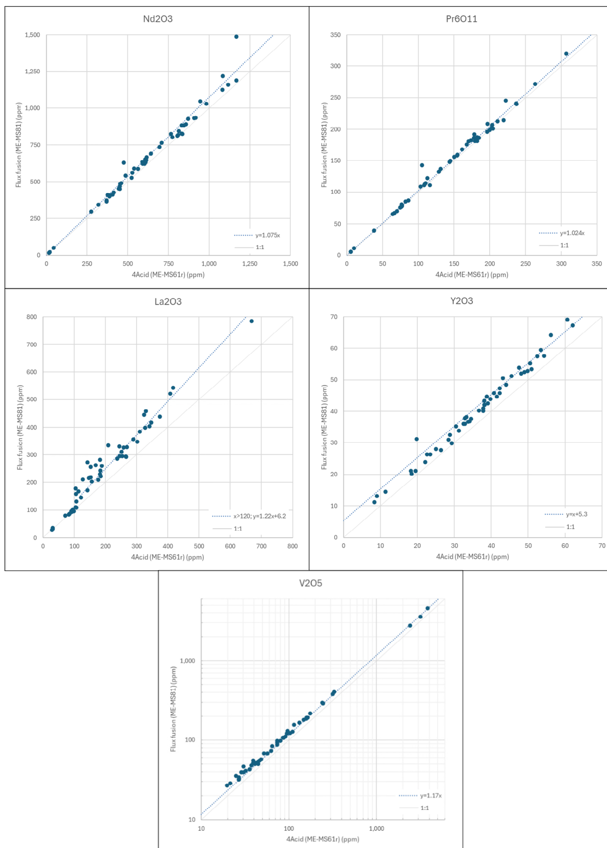
Figure 8-4: Scatter plots of Nd 2 O 3 , Pr 6 O 11 , La 2 O 3 , Y 2 O 3 and V 2 O 5 four-acid ICP-MS vs flux-fusion ICP-MS data and linear regressions used for grade adjustments (Sterk, 2024).
