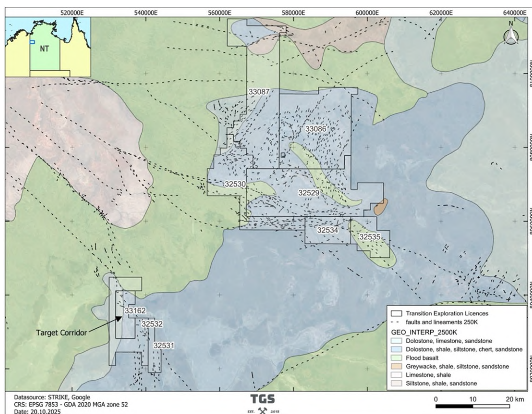
Figure 4-3: Regional geological and structural map of the Buntine Project area.
