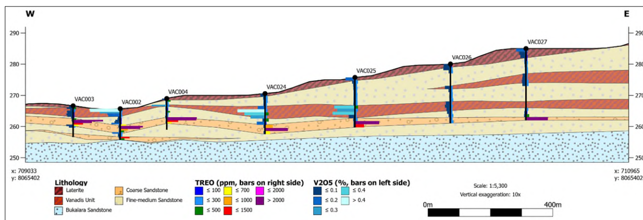
Figure 6-3: Sedimentary interpretation of an E-W section through the Vanadis Prospect, with V 2 O 5 and TREO grades (10 x vertical exaggeration).
