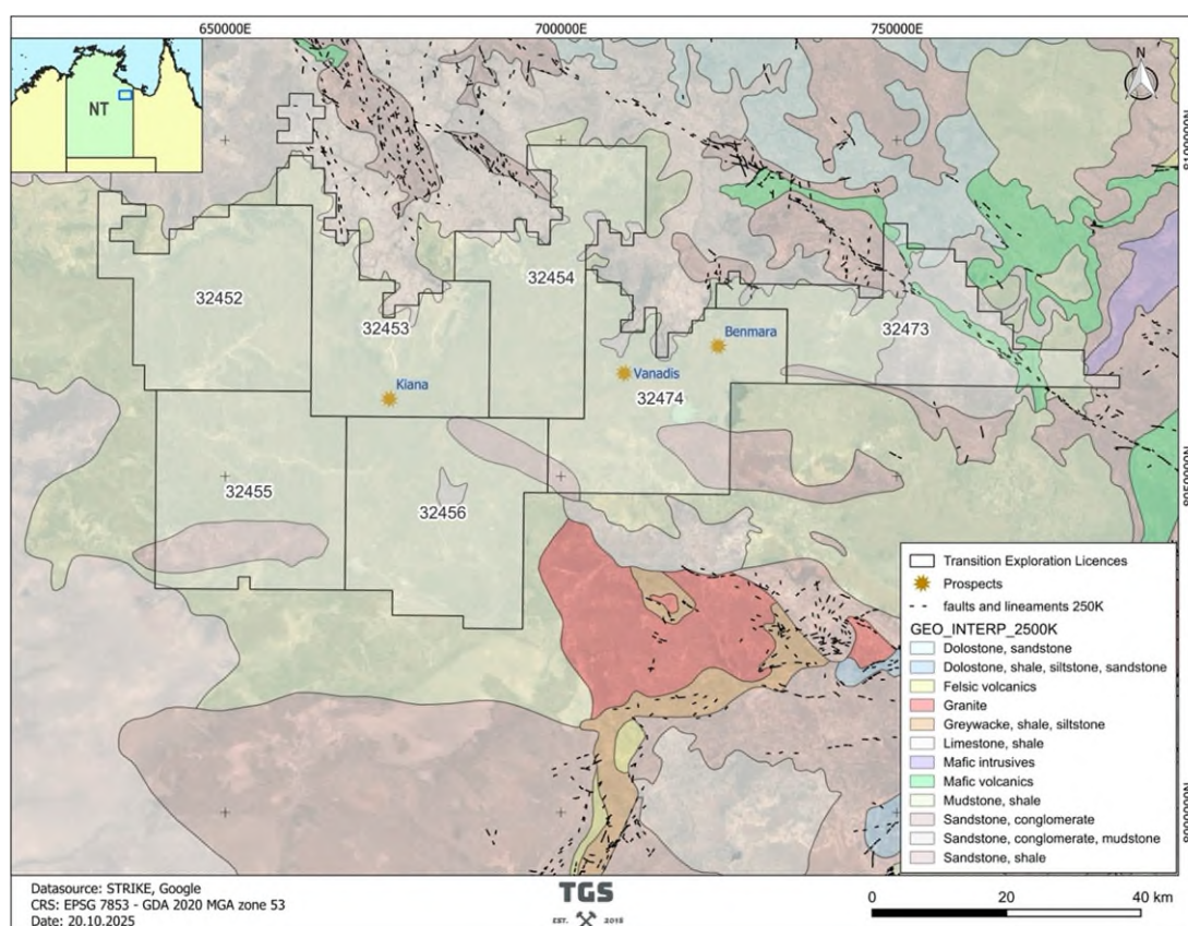
Figure 4-2: Regional geological and structural map of the Barkly Project area.
