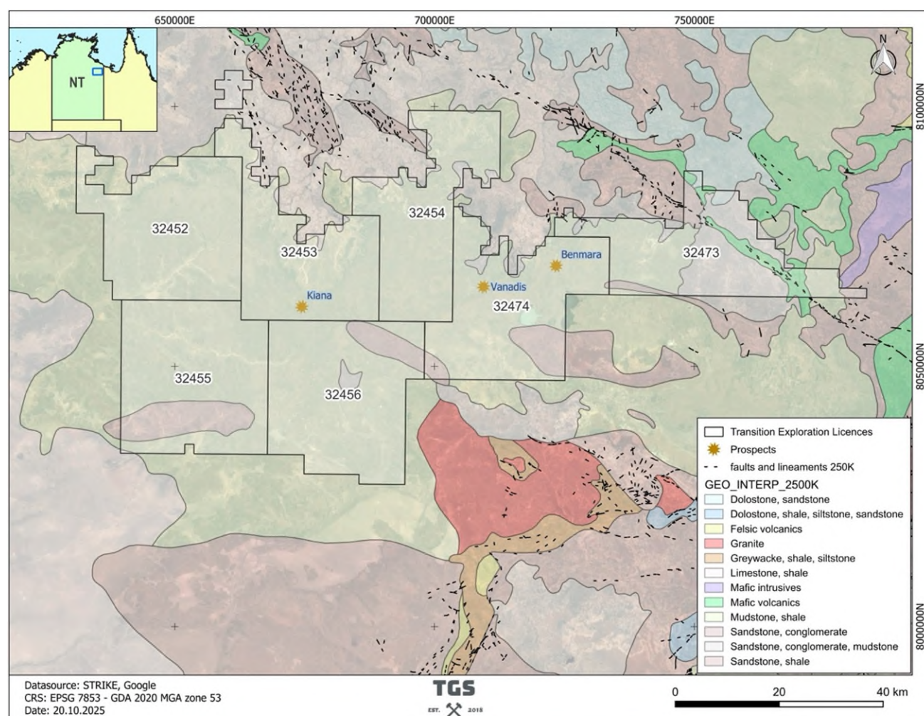
Figure 2: Regional geological and structural map of the Barkly Project area.
