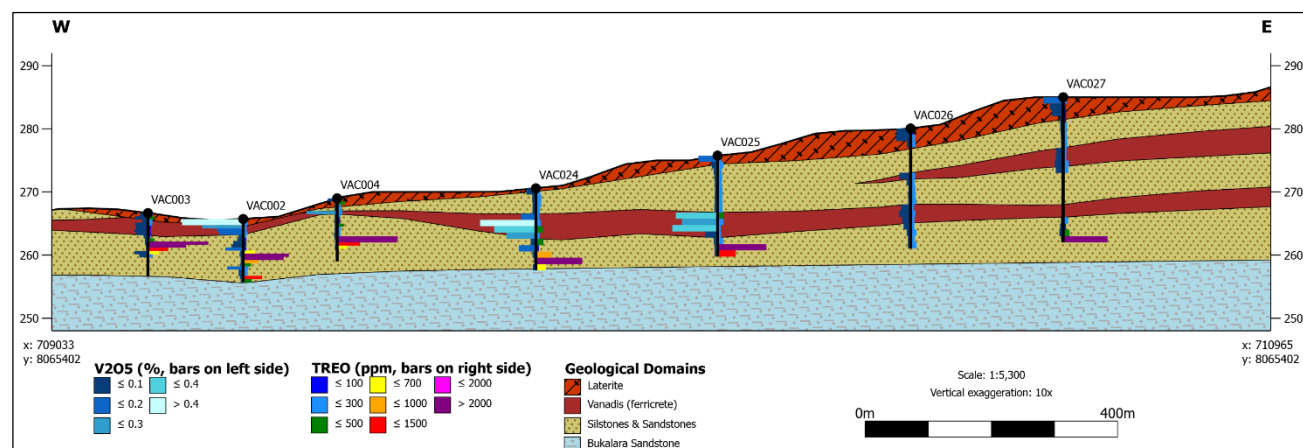
Figure 9-1: West to east cross-section (8,065,402 mN), looking north of the modelled geological domains
