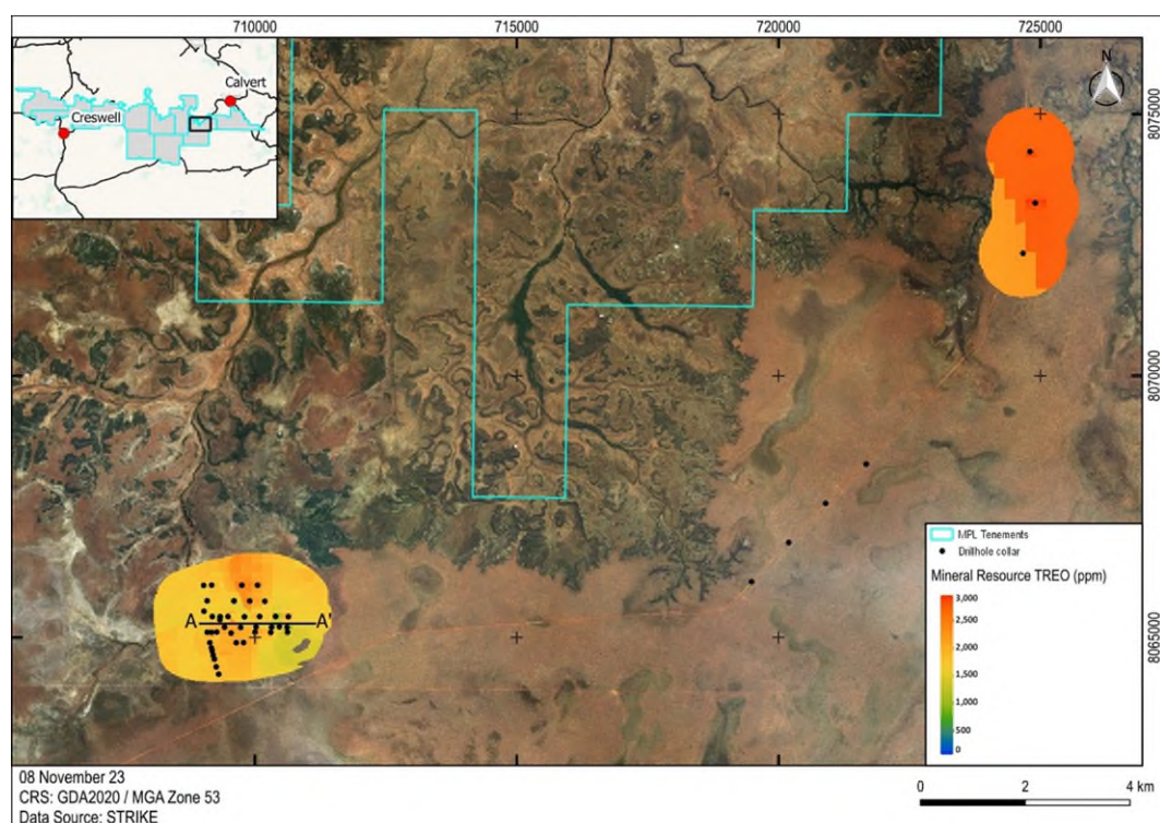
Figure 9-7: Plan view of the Barkly REE Inferred Mineral Resource extent and grades
