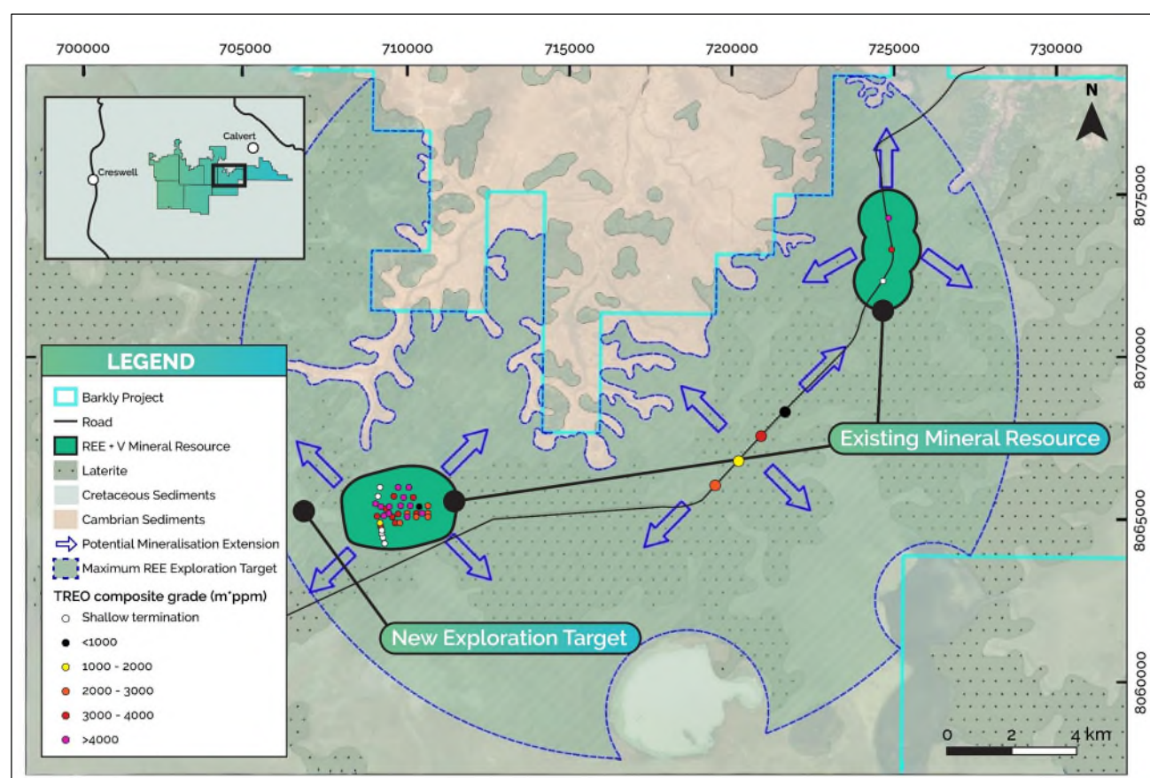
Figure 5: Barkly Project rare earth element Exploration Target.
