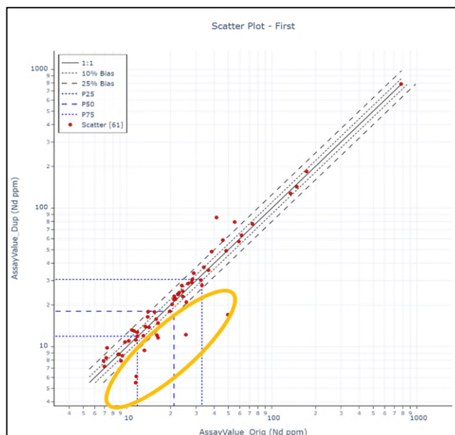
Figure 8-2: First-split RD plot for Nd (four-acid ICP-MS).
