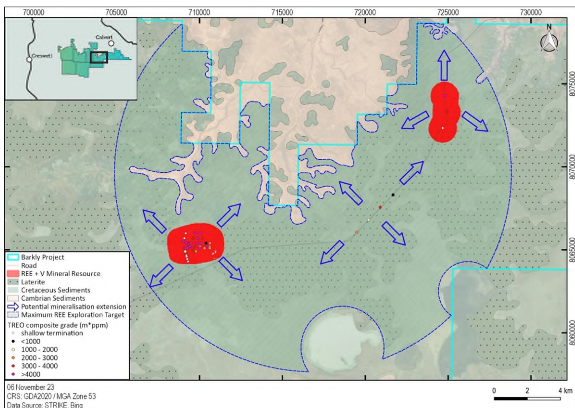
Figure 11-1: Maximum extent of estimated REE Exploration Target.
