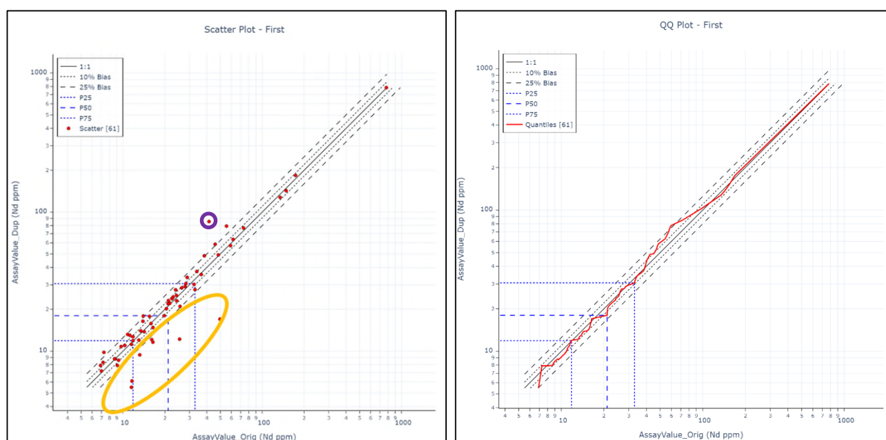
Figure 8-3: Scatter (left) and QQ (right) plot Nd (ppm, 4A ICP-MS) first-split repeats.
