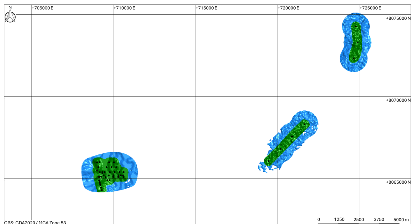
Figure 9-2: Plan view of Mineral Resources within 300 m of drill lines (green) and extrapolation beyond 300 m (blue).
