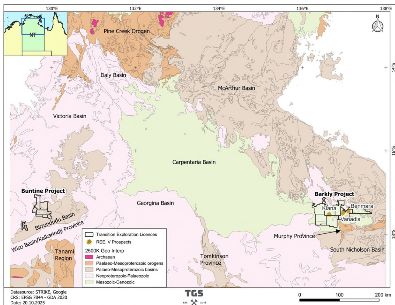
Figure 4-1: Regional geology of the project areas.
