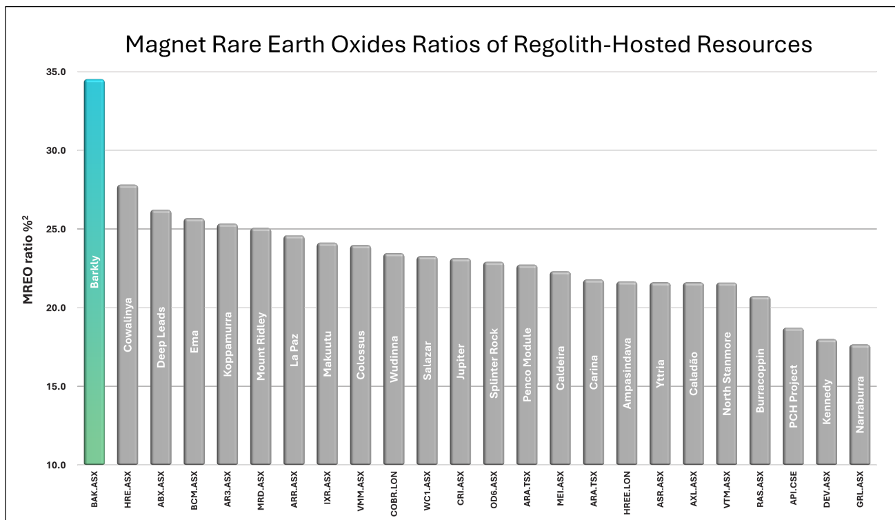
Figure 3: MREO/TREO ratio of rare earth resources of regolith-hosted reesources globally. Data citations are available in Appendix C of the Independent Technical Assessment Report.
