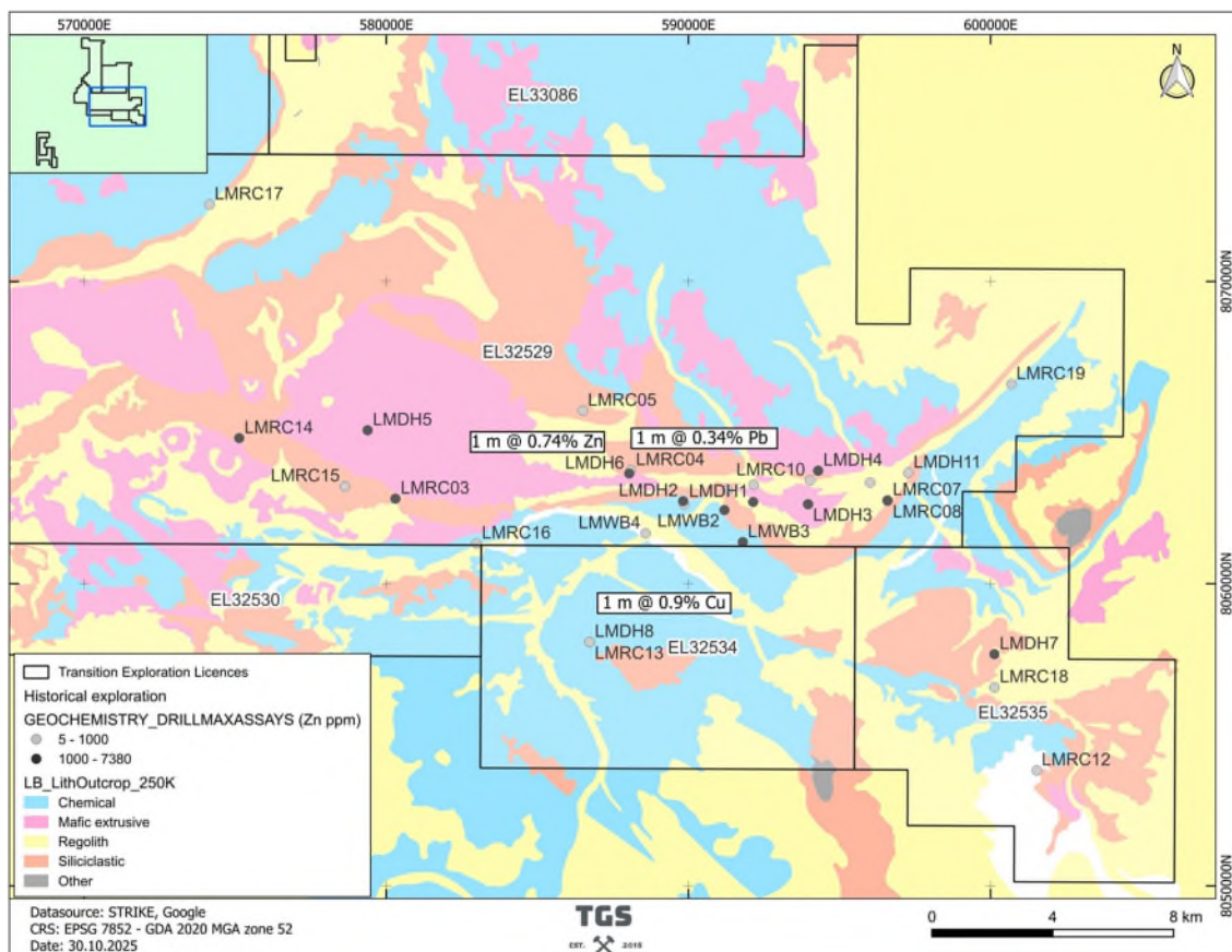
Figure 5-3: Historical drilling data at Buntine from Geopecko with significant intercepts highlighted for LMDH6, LMDH8, and LMRC04.
