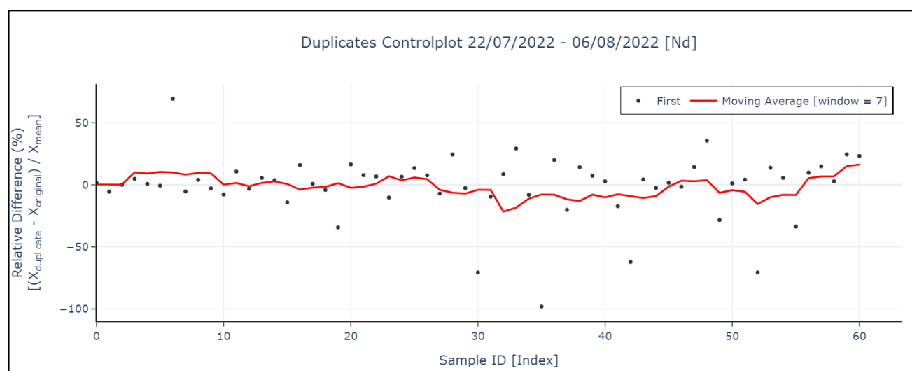
Figure 8-1: First-split repeat RD plot for Nd (four-acid ICP-MS).
