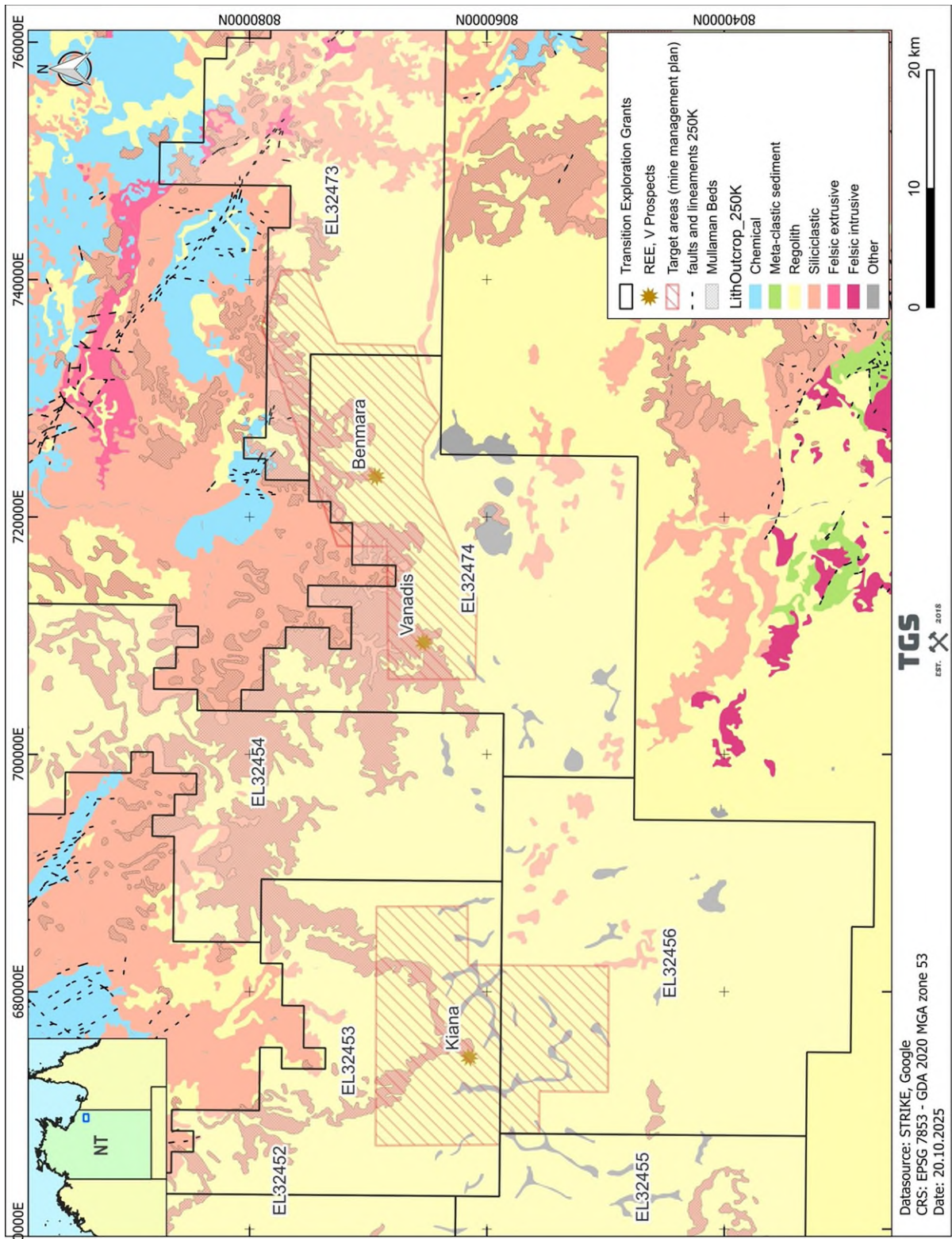
Figure 4-4: Geological map of the Barkly Project.
