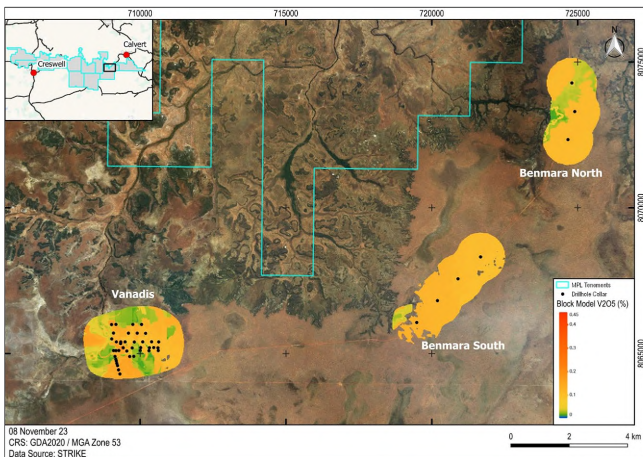
Figure 9-8: Plan view of Barkly V_2O_5 Inferred Mineral Resource extent and grades.
