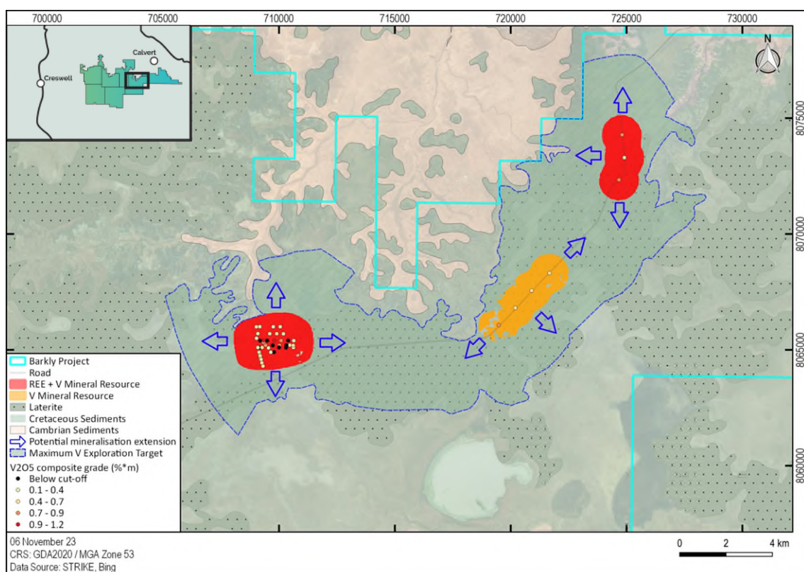
Figure 11-2: Maximum extent of estimated V 2 O 5 Exploration Target.
