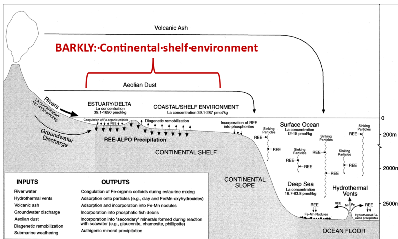
Figure 4-9: Schematic diagram of major inputs and outputs of REEs in the ocean cycle, modified from Rasmussen et al. (1998).
