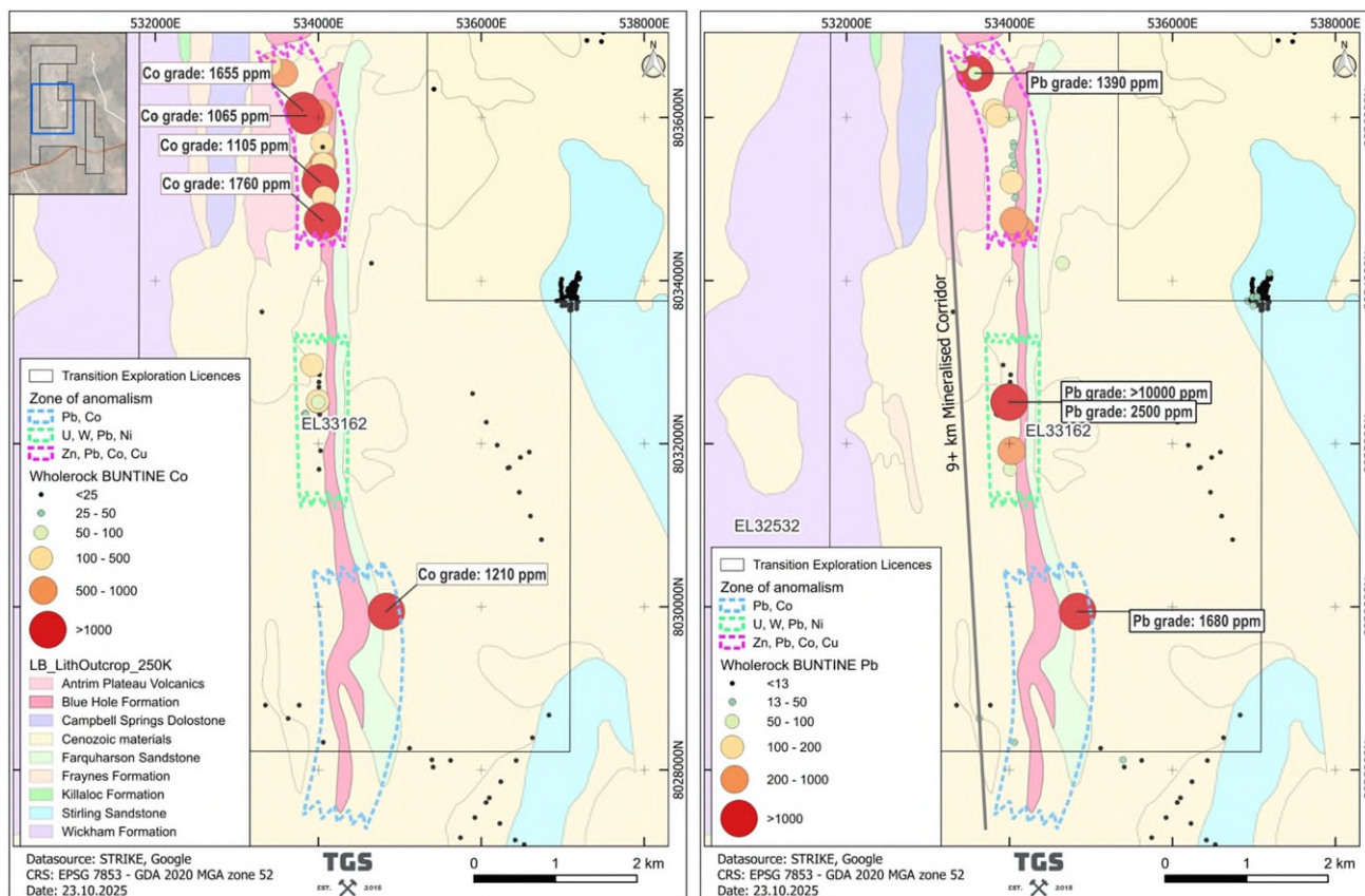
Figure 5-2: Rock-chip sampling programme at Buntine with exemplary results from Pb and Co.
