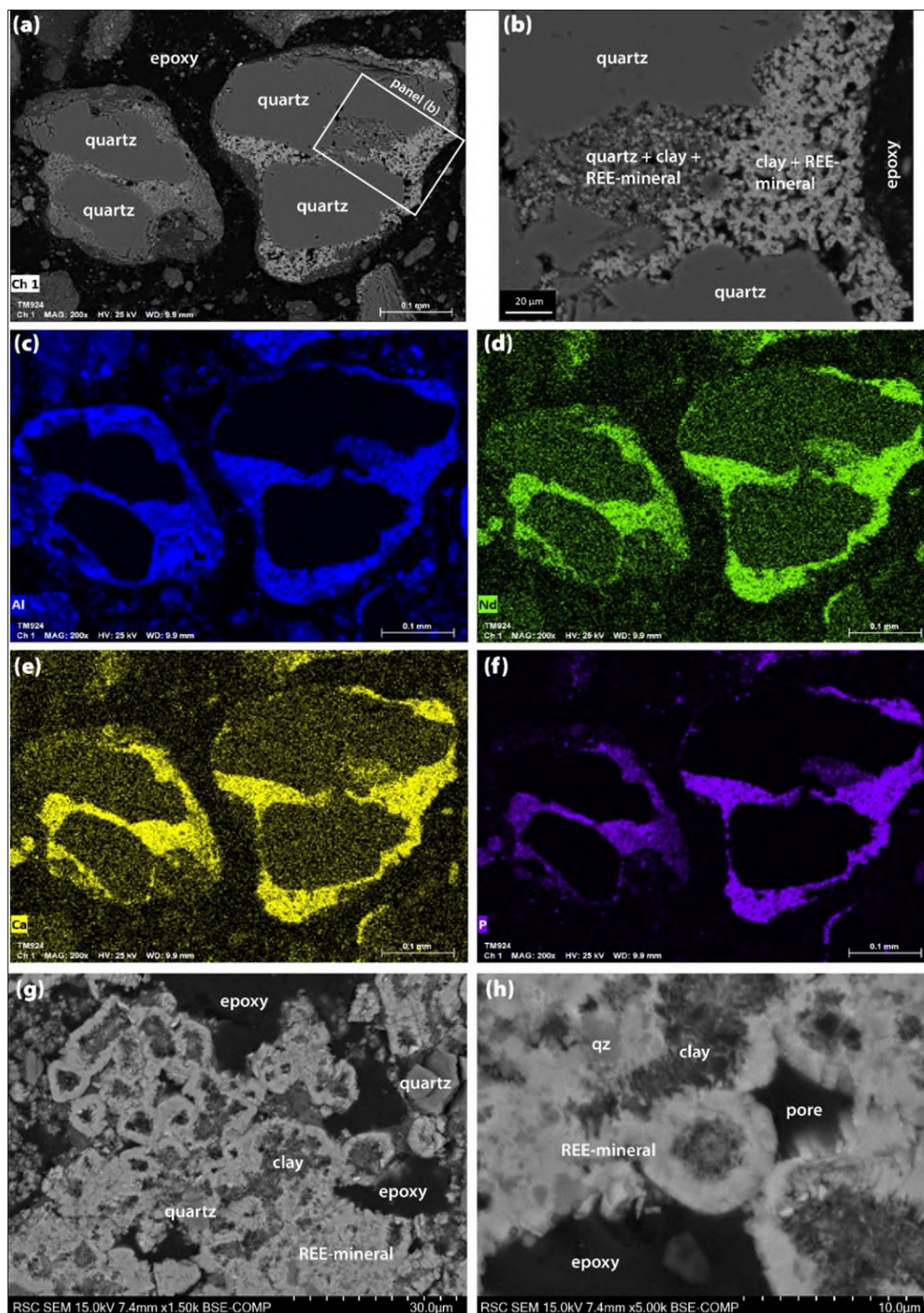
Figure 6-4: Vanadis SEM results: (a) BSE image of APS minerals (labelled as REE mineral) around quartz in sample TM00924; (b) BSE image of area indicated in (a), with intergrowths of clay and quartz; (c) EDS map of Al concentrations for panel (a); (d) EDS map of Nd concentrations for panel (a); (e) EDS map of Ca concentrations for panel (a) — considered alongside panels (a) to (c), the EDS maps indicate the presence of Al, Nd, Ca, and P almost exclusively in the APS mineral phase; (f) EDS map of P concentrations for panel (a); (g) BSE image of an REE mineral surrounding clusters of clay grains; and (h) high-resolution BSE image of an APS mineral surrounding clusters of clay grains with adjacent pore space and minor quartz.
