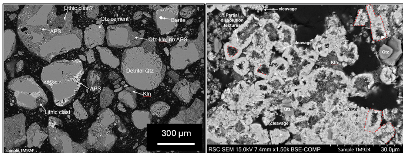
Figure 4-7: Vanadis REE sample SEM results. (Left image) Sample consists dominantly of sand-sized detrital quartz grains, less-abundant rounded kaolinite grains (most likely altered feldspar), and rare lithic clasts that are also composed of quartz-kaolinite; (Right image) APS minerals form masses of hollow, ring-shaped crystals and are typically finely intergrown with quartz (Serk, 2024).
