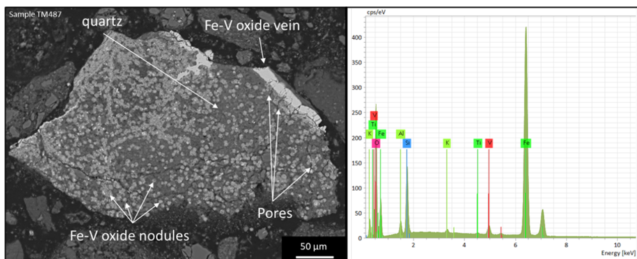
Figure 4-8: Vanadis SEM V sample results: (Left image) Back-scatter electron image of spongy nodular Fe-oxide and thin veins, (Right image) example V-enriched Fe-oxide spectrum.
