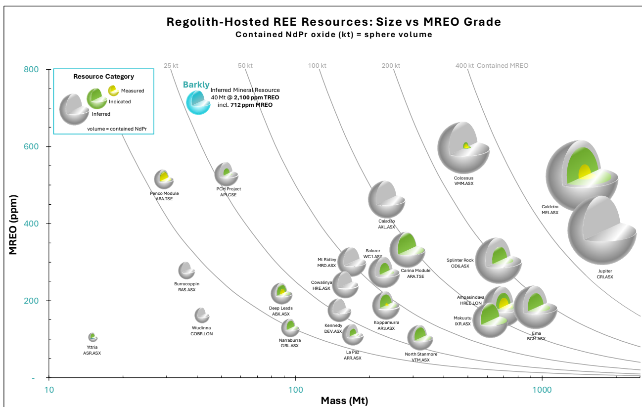
Figure 4: Size and grade of regolith-hosted REE Mineral Resources globally. Peer selection criteria and data citations are in Section 12 and Appendix C of the Independent Technical Assessment Report.
