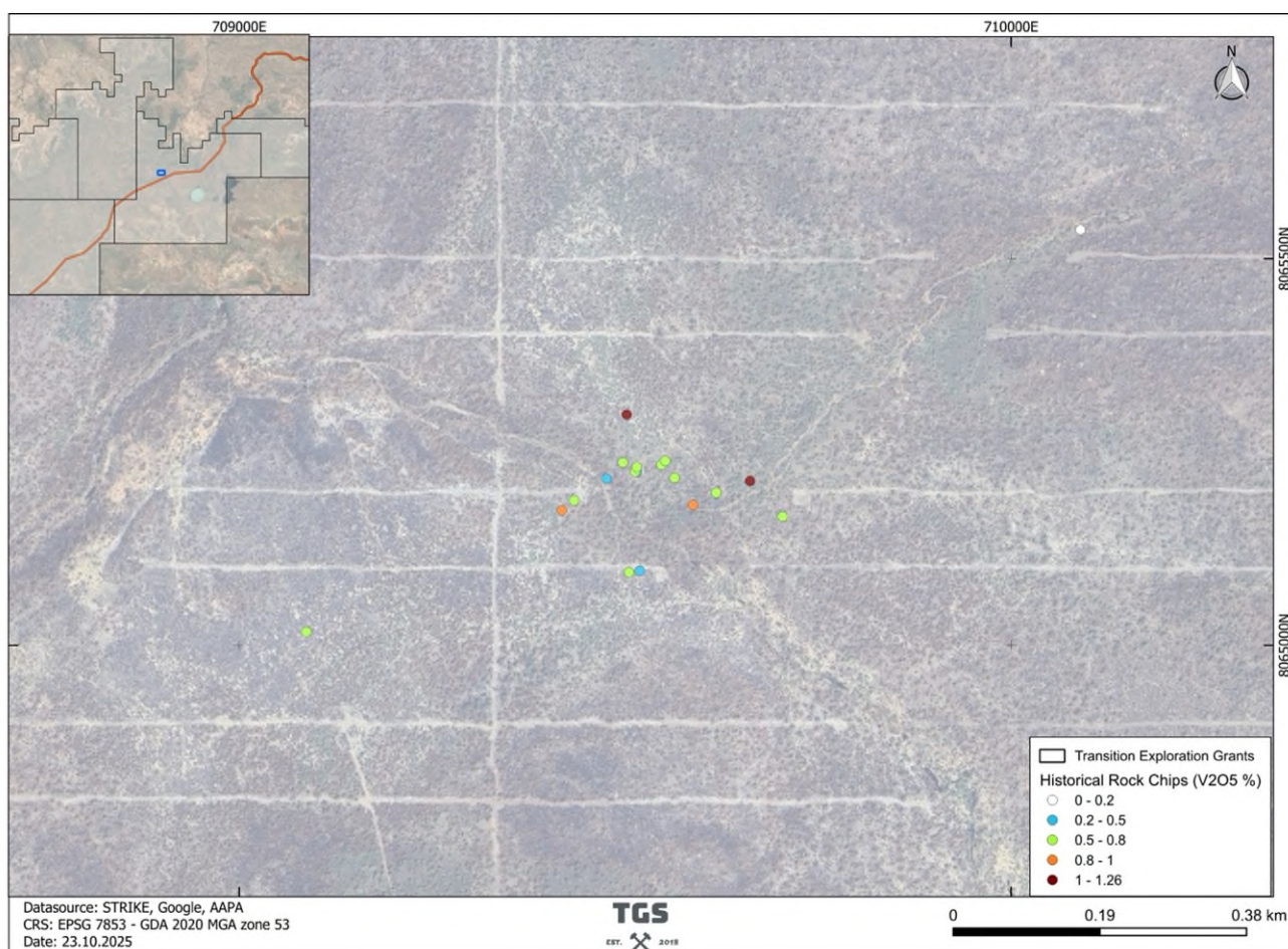
Figure 5-1: Historical rock-chip samples over Vanadis with up to 1.26% V_2O_5 .
