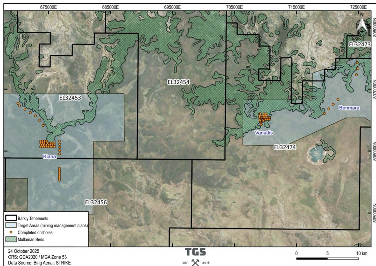
Figure 6-2: Plan view of AC drillholes completed at the Barkly Project.
