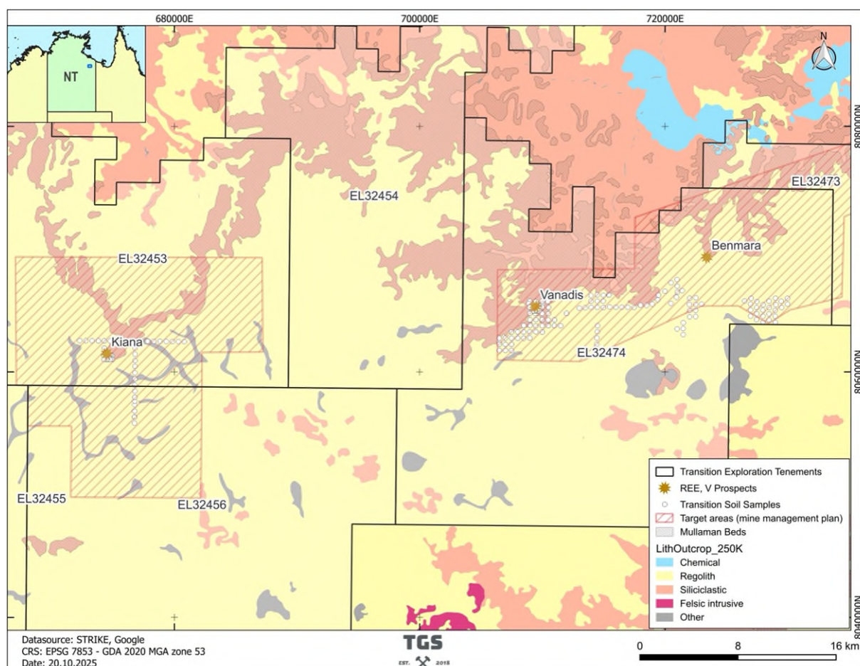
Figure 6-1: Soil samples collected by Barkly Rare Earths at surface and 0.5 m depth.
