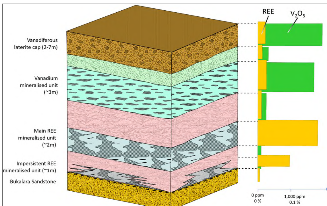
Figure 4-6. Generalised stratigraphic column and geochemical results for Barkly (Source: Barkly Rare Earths).
