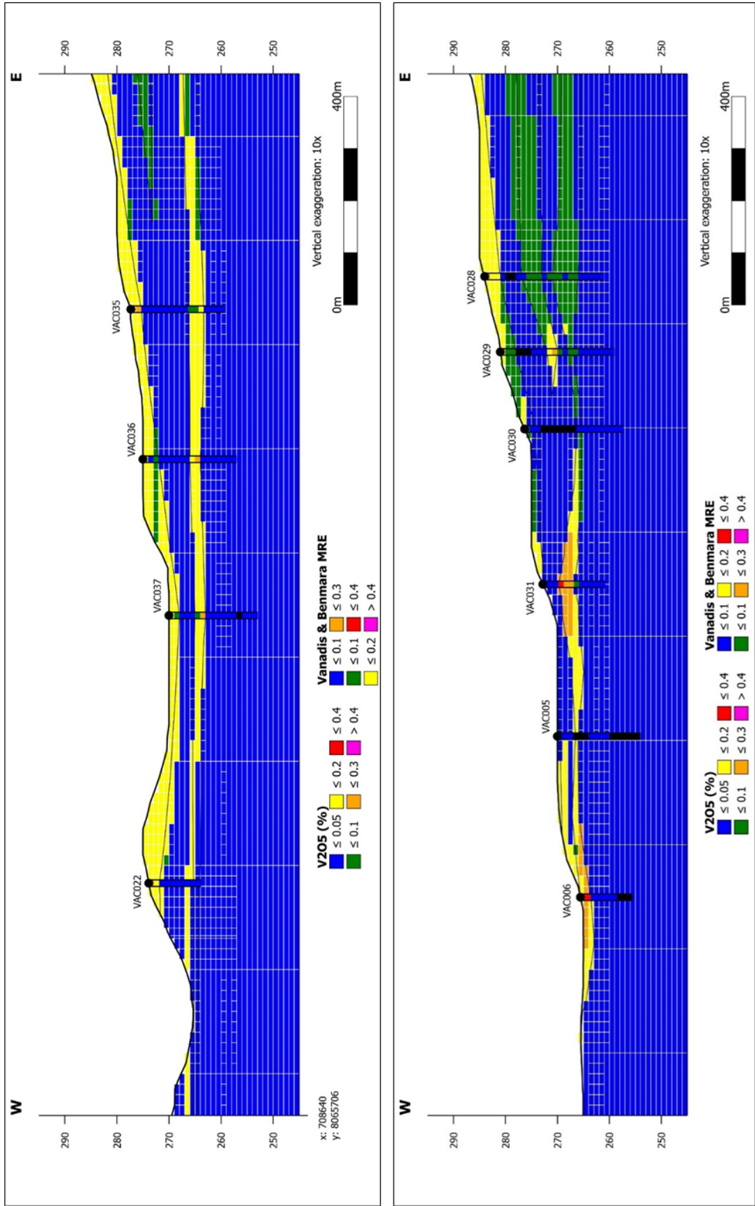
Figure 9-5: Cross-sections comparing the block model against V_2O_5 grades at Vanadis
