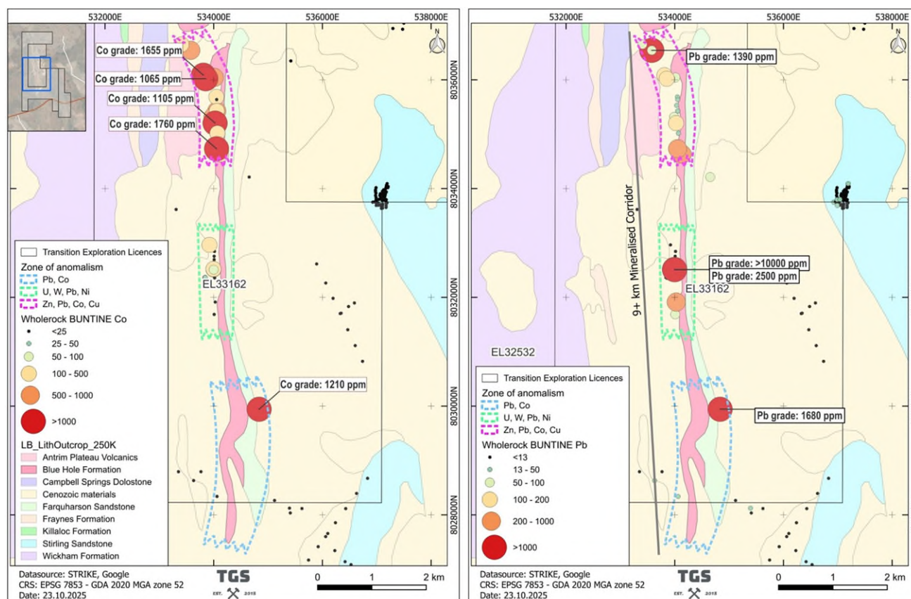
Figure 6: Rock-chip sampling programme at Buntine with exemplary results from Pb and Co.
