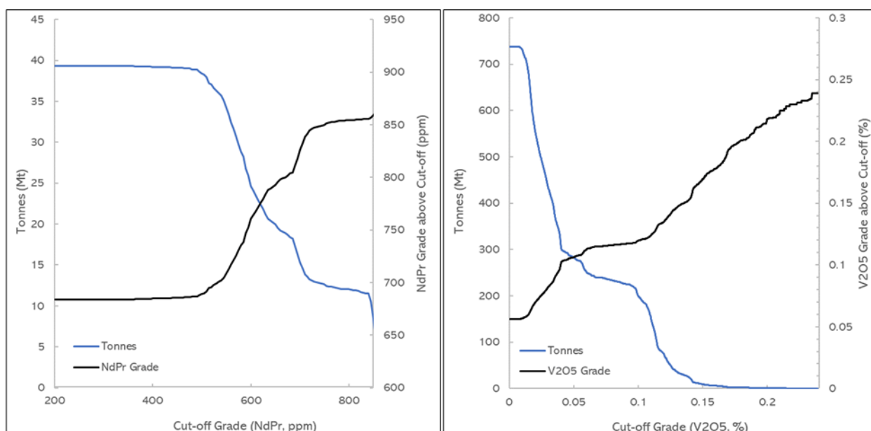
Figure 9-9: NdPr (left) and V_2O_5 (right) grade tonnage curves for the Barkly Mineral Resource (Sterk, 2024).
