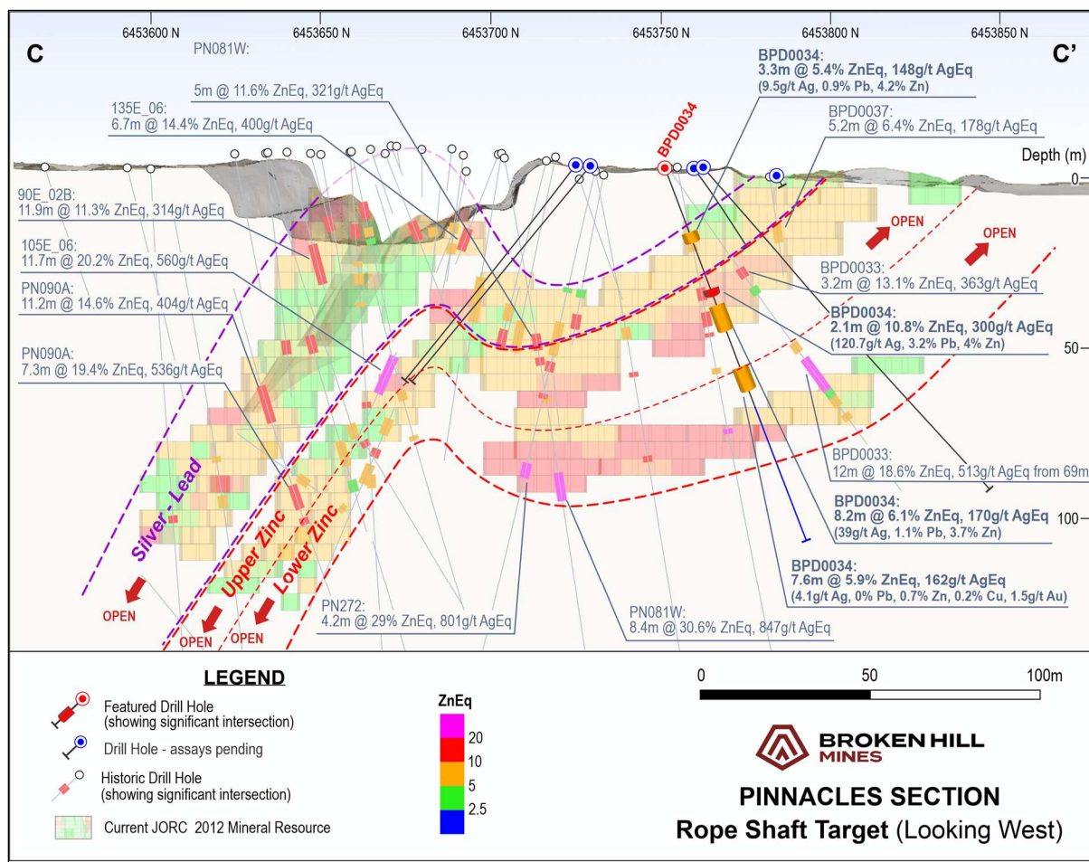
Figure 4 – Pinnacles oblique view C-C' (see Figure 1). Drilling intercepts 4.0% cutoff & 2m internal dilution
