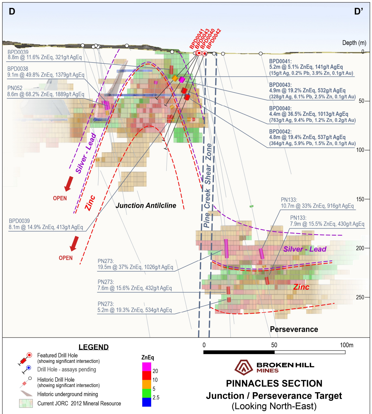
Figure 2 - Pinnacles Section view D-D' (see Figure 1). Displaying new drilling intercepts only, 4.0% cutoff and 2m internal dilution. Historic drillholes are represented in the JORC 2012 MRE Block Model colored by grade ZnEq%.
