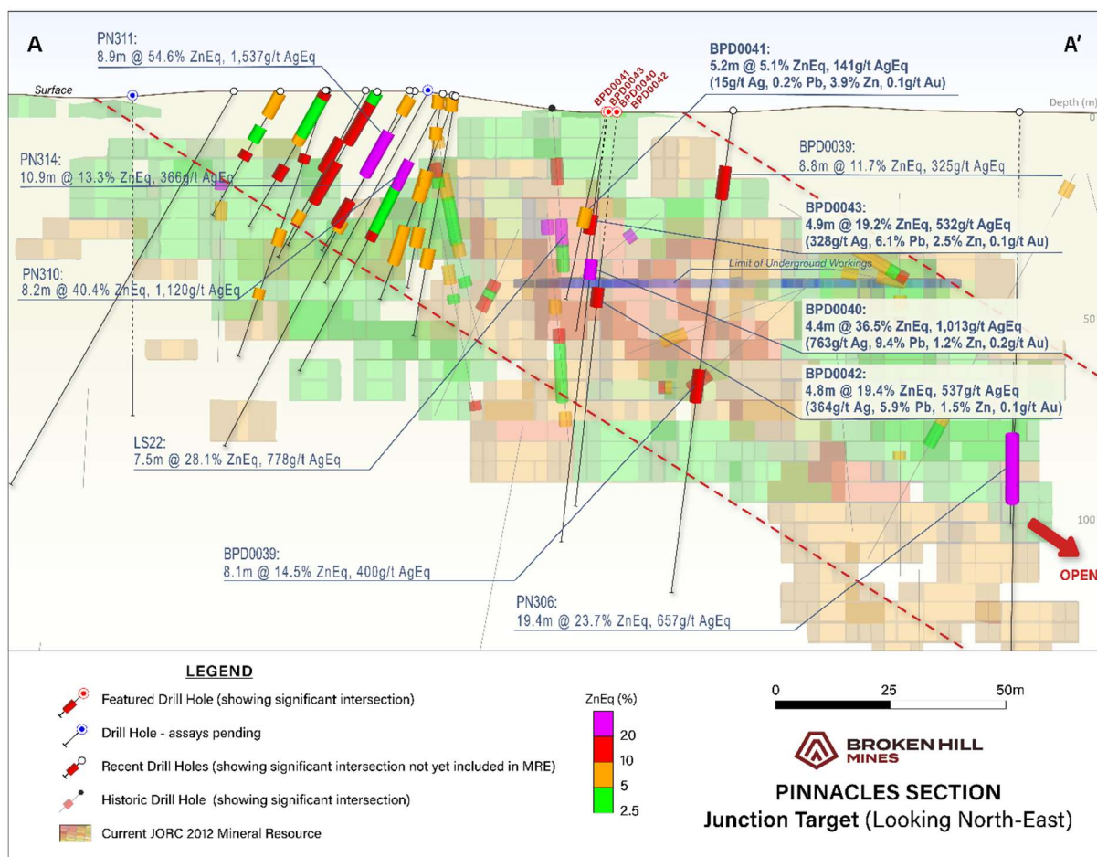
Figure 3 – Pinnacles Section view A-A' (see Figure 1). Drilling intercepts 4.0% cutoff & 2m internal dilution
