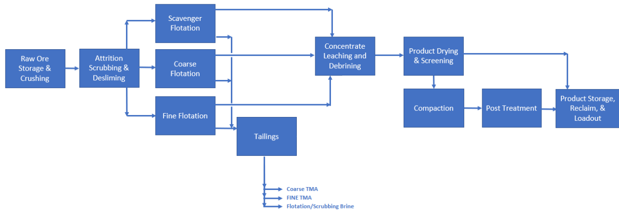
Figure 12 Jansen Process block flow diagram
