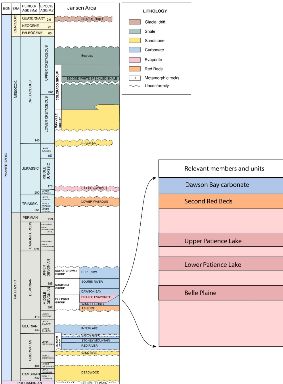
Figure 5. Stratigraphic column for Jansen area
