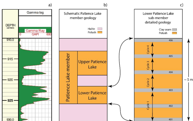
Figure 6 Detailed stratigraphy of the Patience Lake Member.
