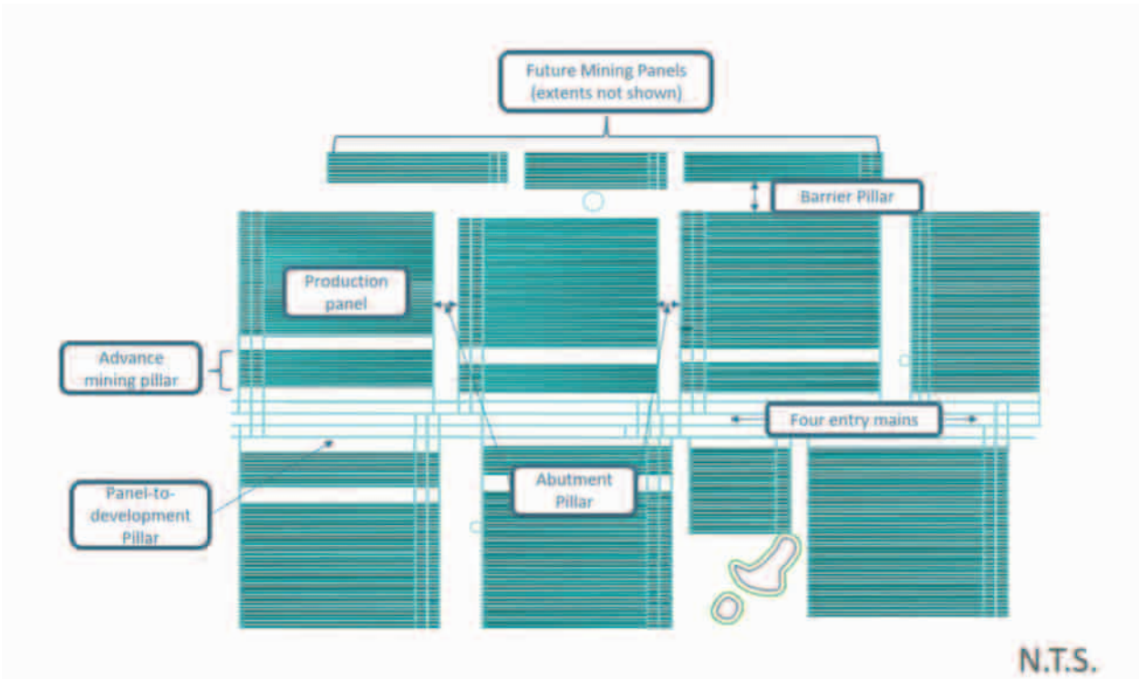
Figure 12-1: Naming convention and typical arrangement of pillars
