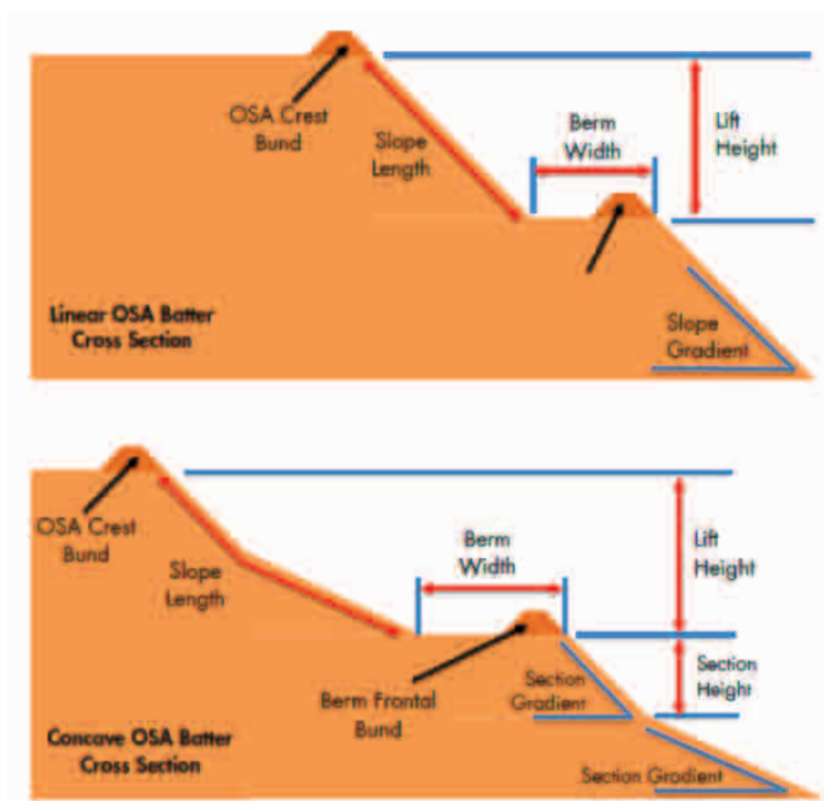
Figure 13-5: Schematic OSA Final Landform Slope Options
