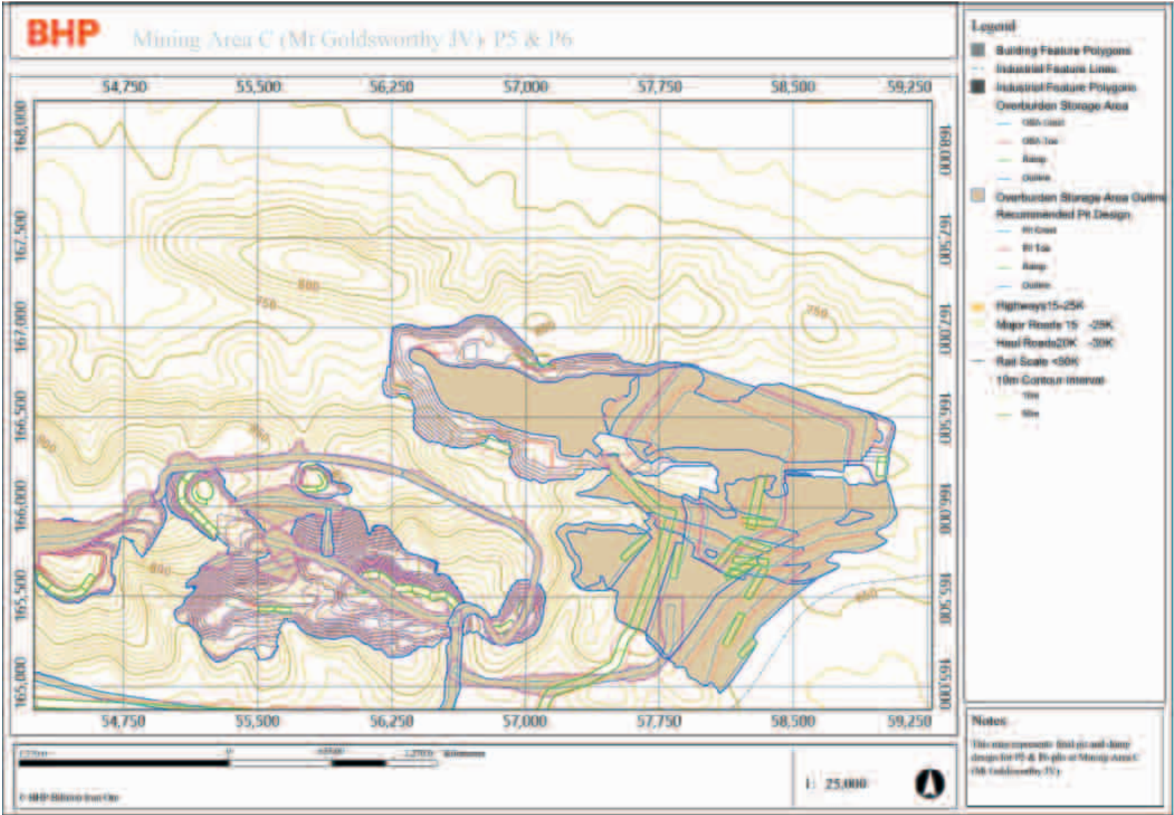
Figure 13-7: Final Pit Maps
