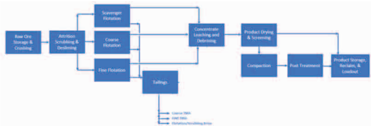
Figure 14-1: Jansen processing sheet flow
