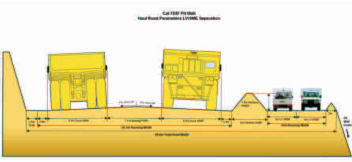
Figure 13-3: CAT 793F Pit Wall (Haul Road Parameters LV/SME Separation)
