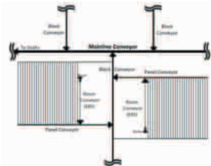
Figure 15-4: Simplified flow diagram of underground conveyor systems
