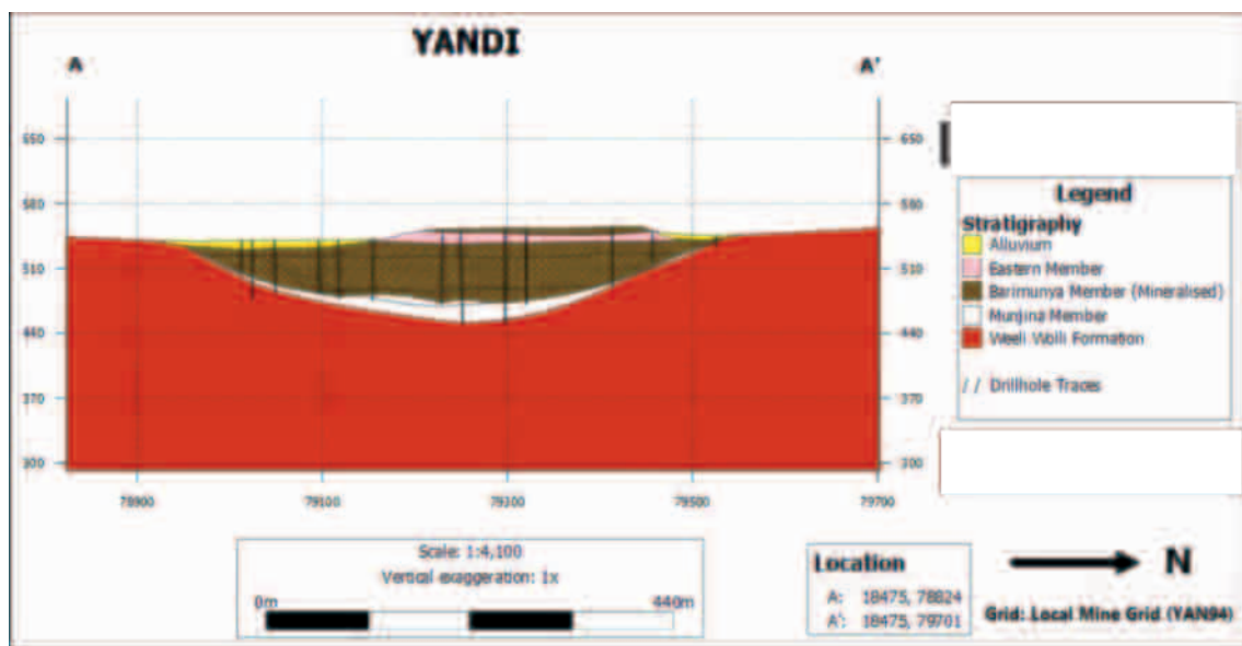
Figure 6-23: Geological cross-section A-A' through Yandi (a CID deposit)
