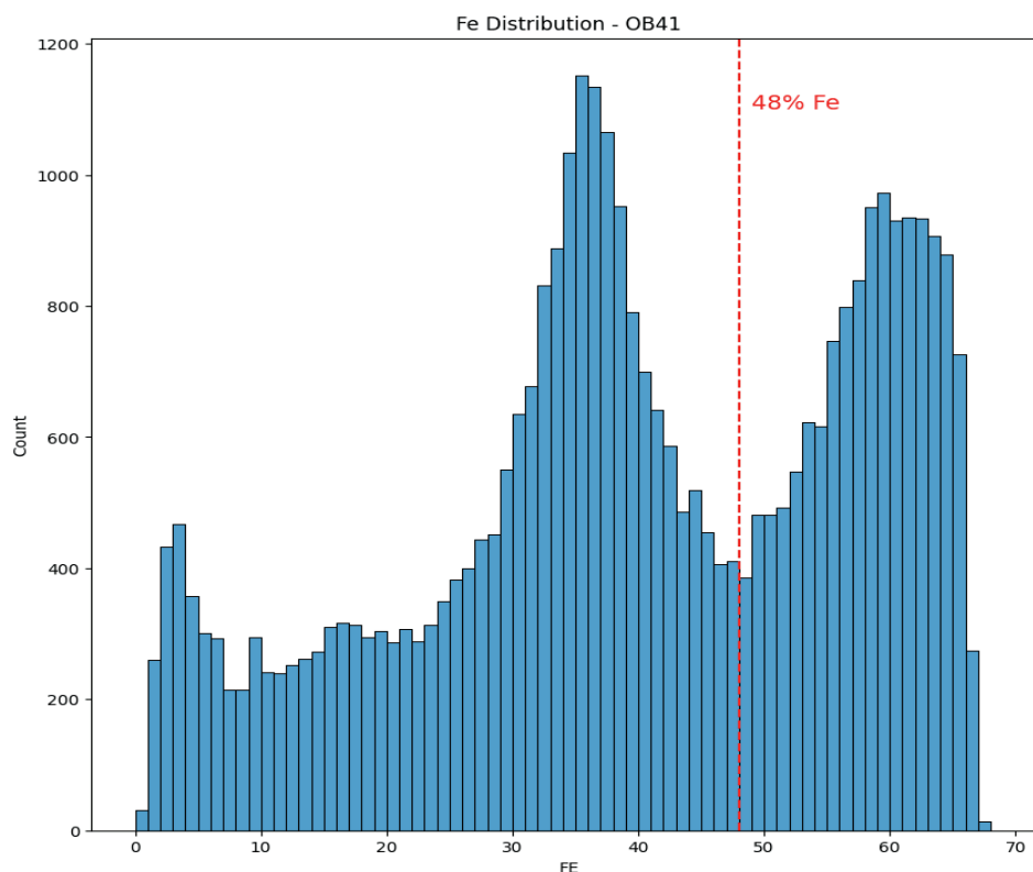
Figure 11-6: Fe Frequency Plot Demonstrating Natural Break in Mineralisation at 48% Fe
