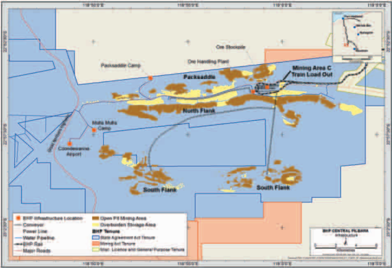
Figure 15-6: Infrastructure Layout Map – Mining Area C and South Flank Areas
