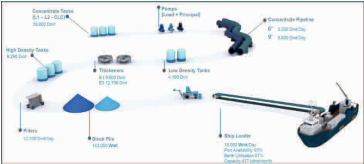
Figure 15-6: Coloso Port Process Schematic
