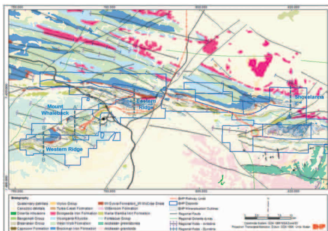
Figure 6-6: Geology Map for Eastern Pilbara Region – Newman Deposits (including approximate location of deposit cross-sections)
