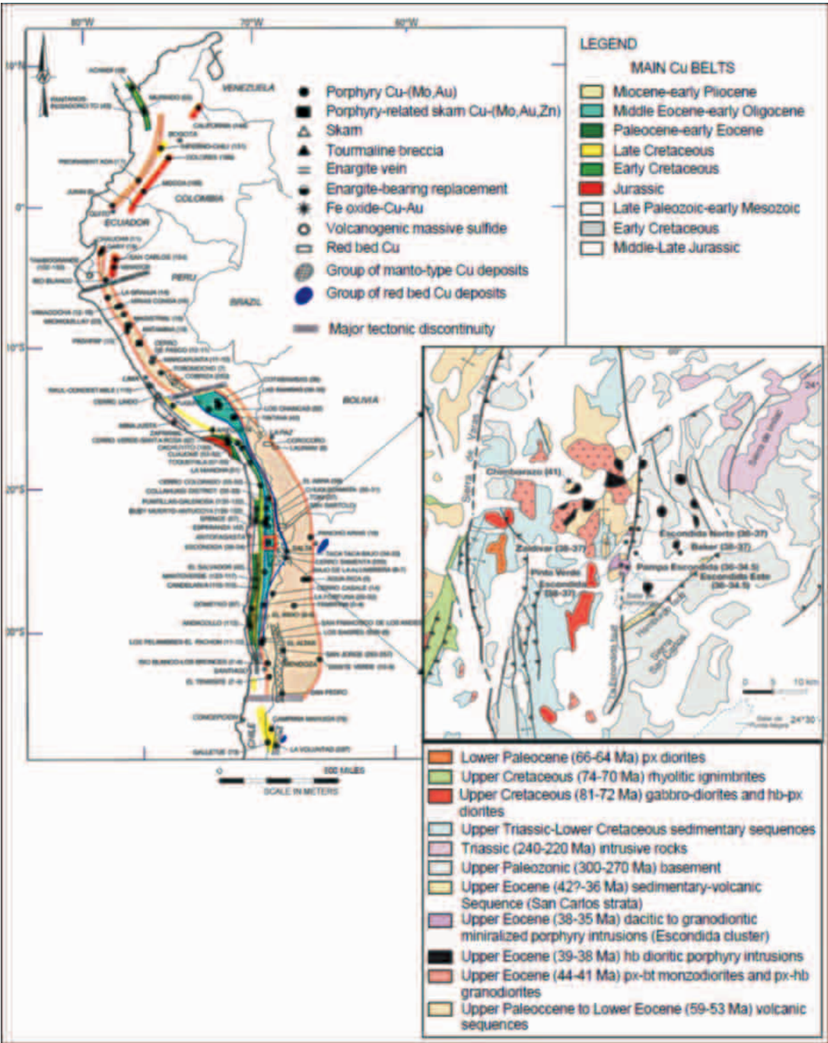
Figure 6-1: A) Metallogenic Belts of the Andes and their Main Copper-bearing Porphyries, B) Regional Geology Escondida District
