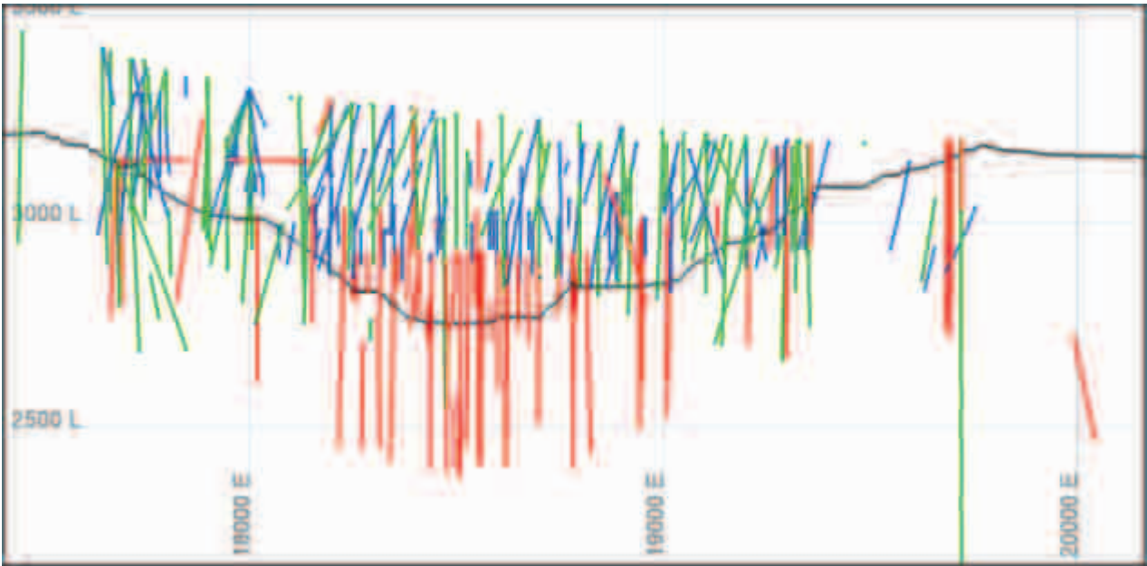
Figure 7-4: Vertical Section 108,600N with Drill Hole per Type, Escondida
