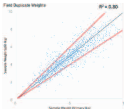
Figure 8-4: Field Duplicate Weight Data for FY2026
