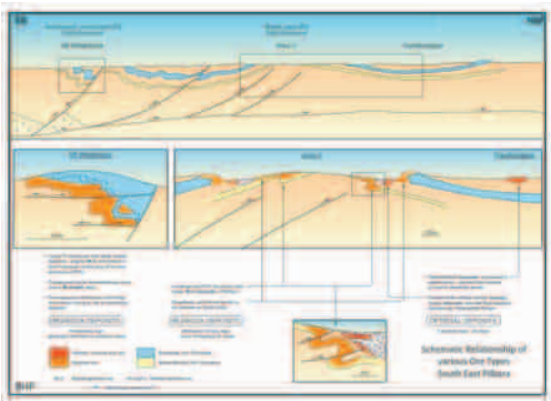
Figure 6-3: Schematic Structural Relationship of Various Material Types of South East Pilbara
