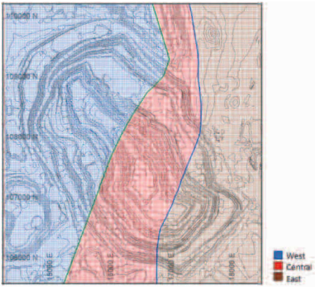
Figure 11-5: General View of the Pulse Variable, Escondida
