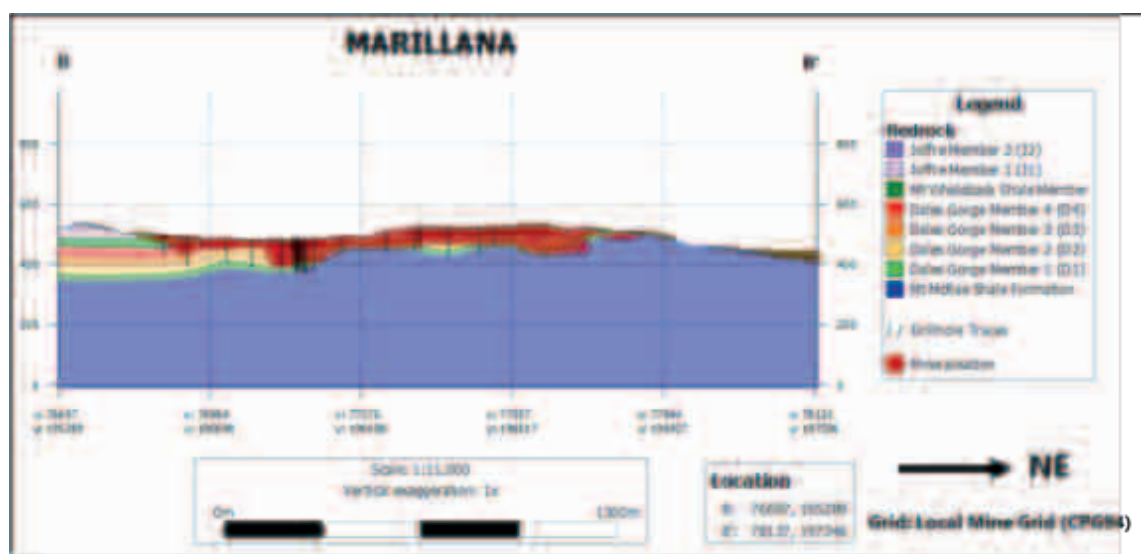
Figure 6-24: Geological cross-section B-B' through Marillana (a BKM deposit)
