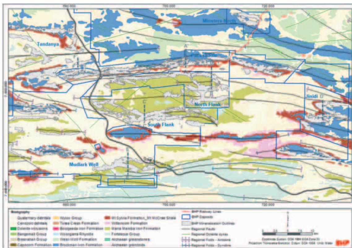
Figure 6-15: Geology Map of Central Pilbara Region (including approximate location of deposit cross-sections)
