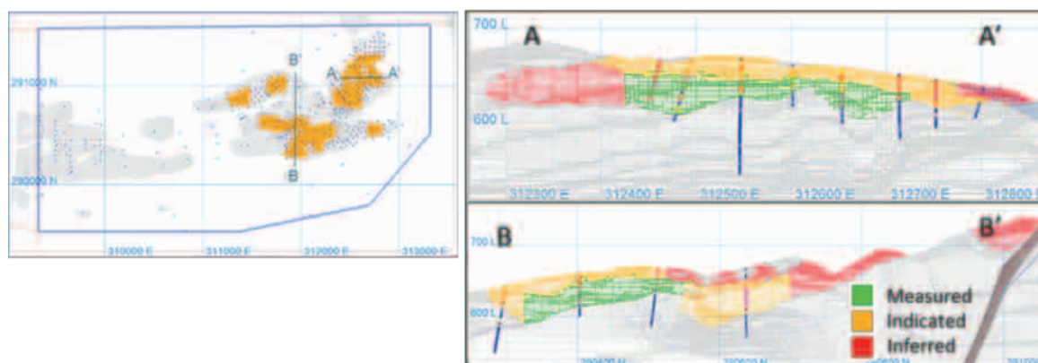
Figure 11-14: Measured Resource Classification – Plan view and cross-section
