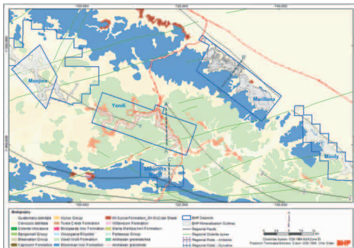
Figure 6-22: Geology Map for Yandi Region (including approximate location of deposit cross-sections)
