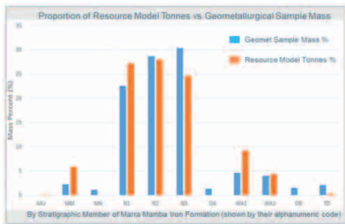
Figure 10-2: Illustration of Geometallurgical Sample Representivity by Stratigraphy
