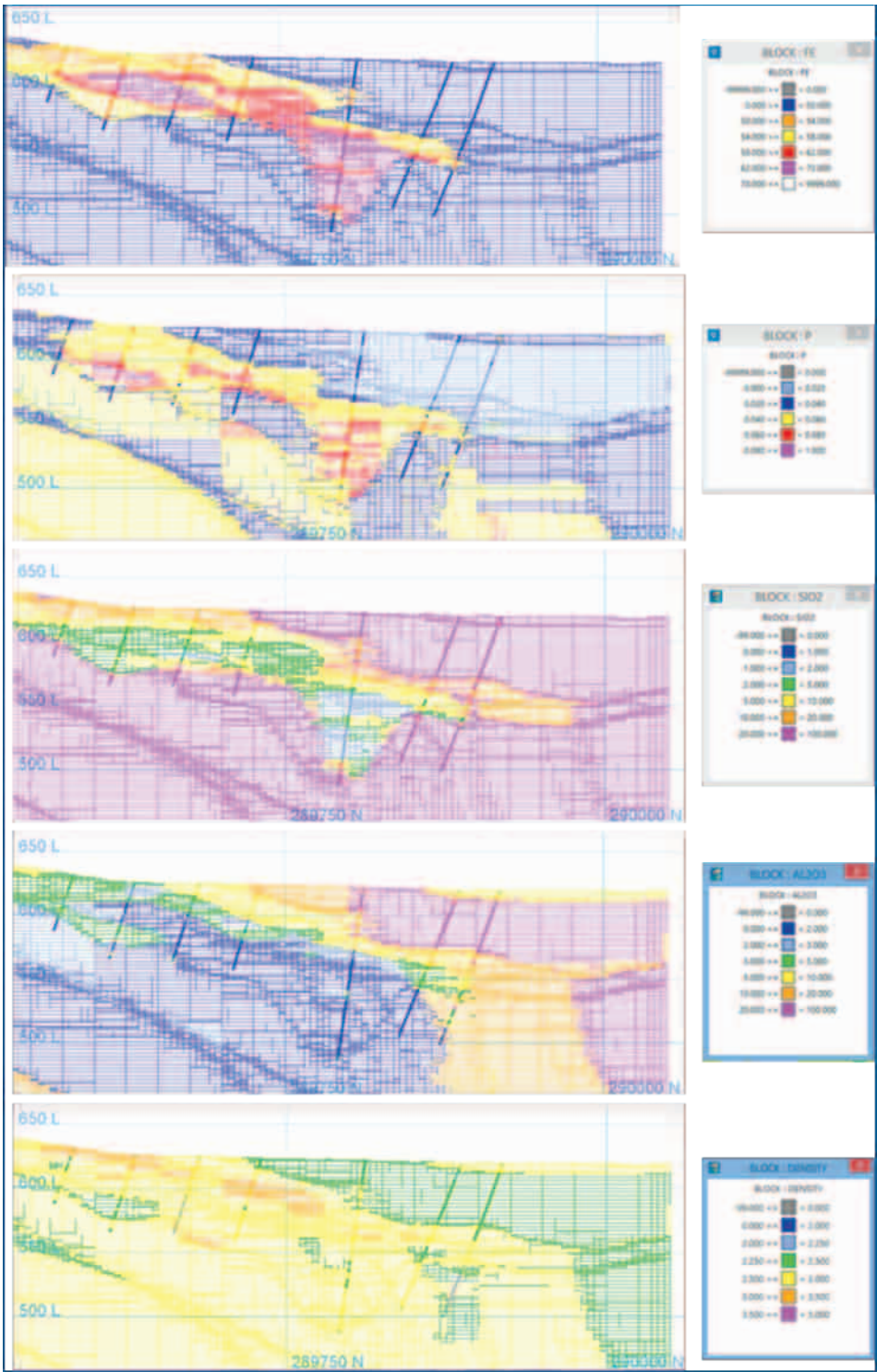
Figure 11-10: Illustration of Typical Visual Validation reviewing sections to compare drill hole grades with estimated block grades
