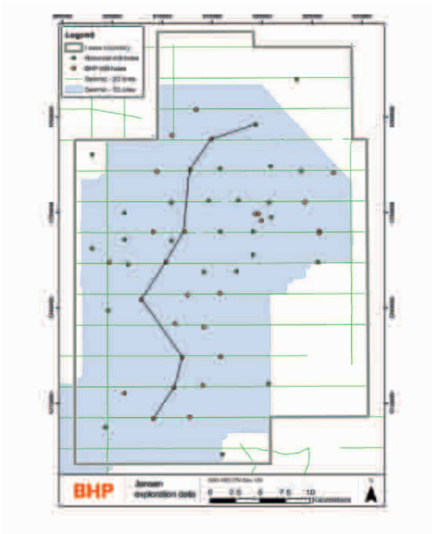
Figure 7-1: Exploration coverage. The black line shows the location of the cross section displayed in Figure 7-5.
