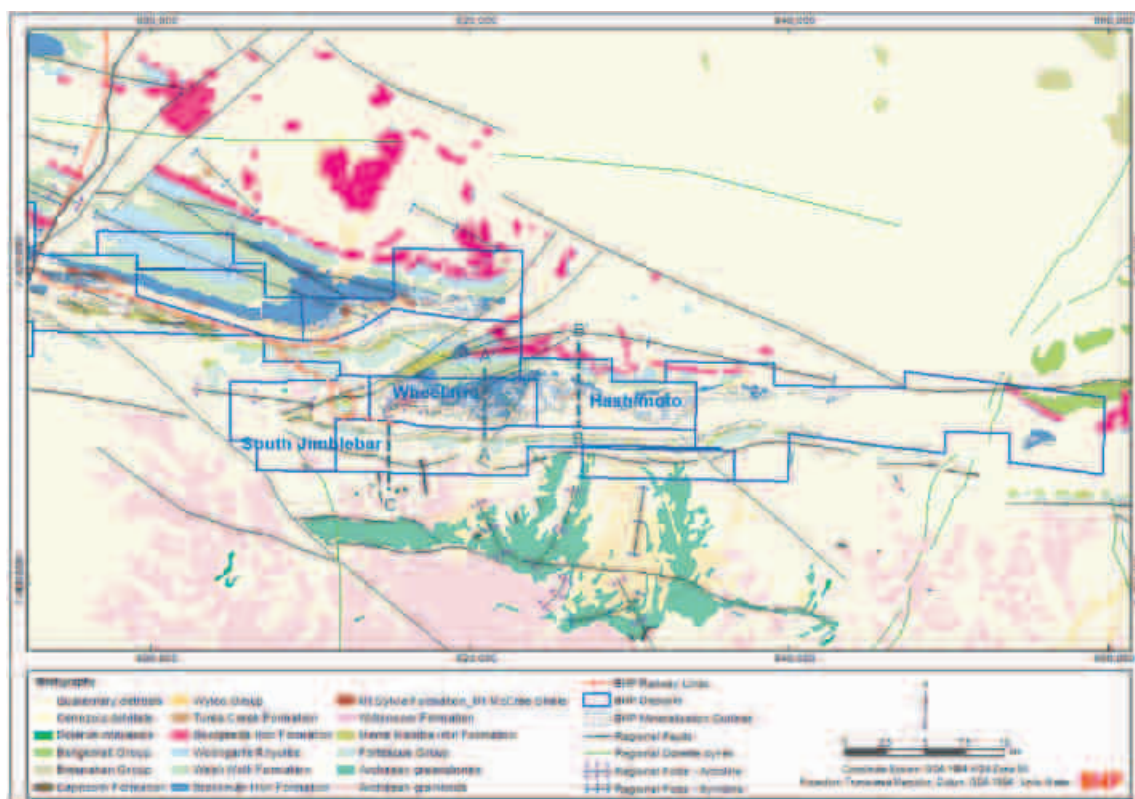
Figure 6-11: Geology Map for Eastern Pilbara Region – Jimblebar Deposits (including approximate location of deposit cross-sections)
