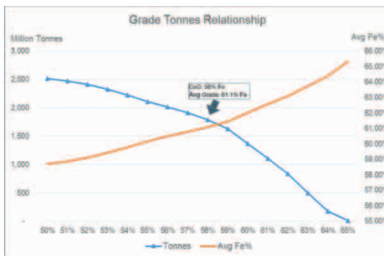
Figure 12-4: Grade Tonnage Relationship
