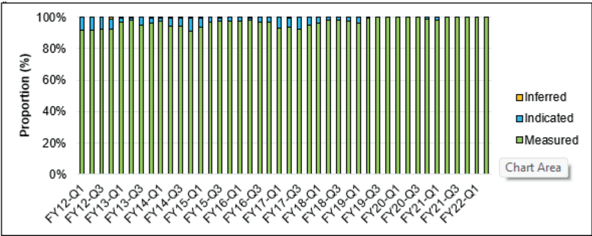
Figure 11-26: Mined Sulphide Material by Mineral Resources Category, FY12 to FY22, Escondida Norte
