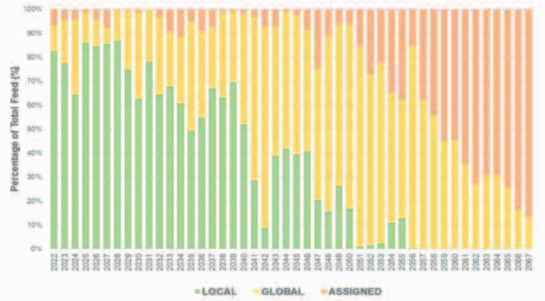
Figure 10-4: Geometallurgical Classification Profile for Copper Recovery at Concentrators on Long Term Plan 22
