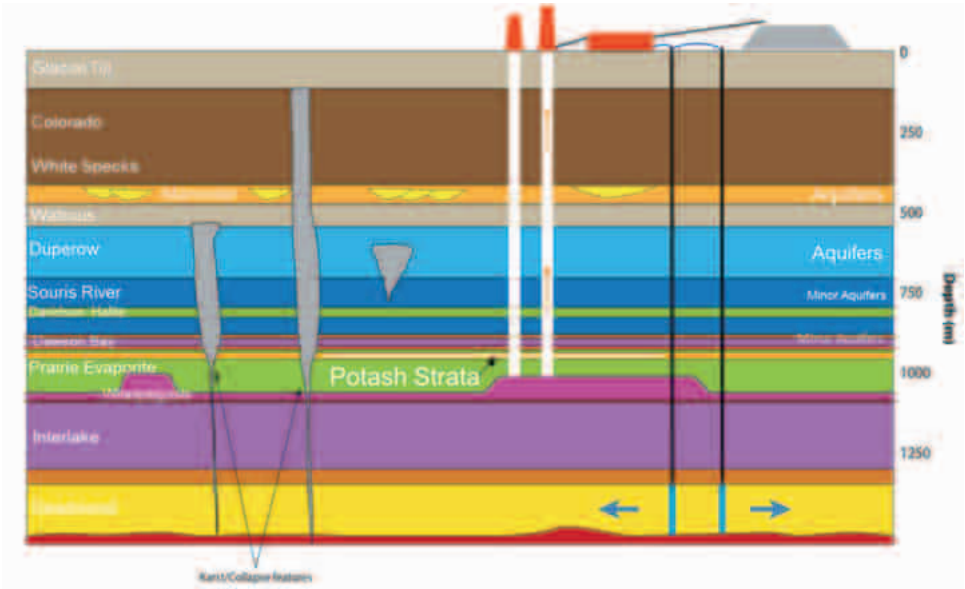
Figure 13-2: Schematic of Local Geology, Aquifer locations in relation to Potash Strata
