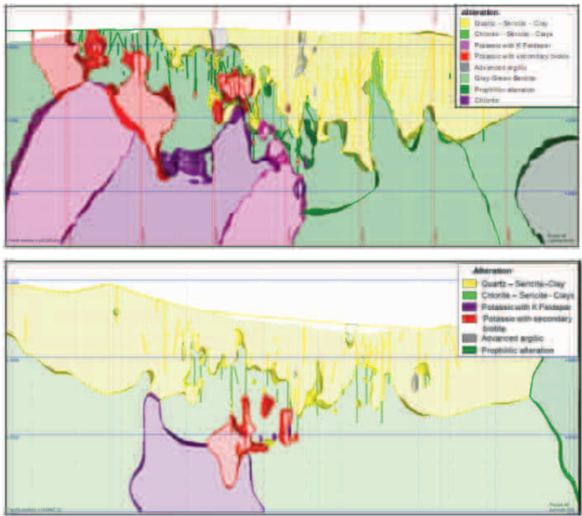
Figure11-2: Example Alteration Cross-Sections for Escondida Section 107,255N (top) and Escondida Norte Section 114,100N (bottom)
