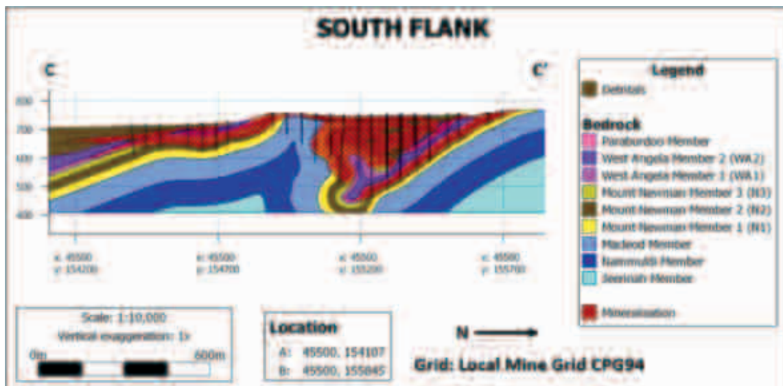
Figure 6-18: Geological Cross-section C-C' through South Flank (a MM deposit)
