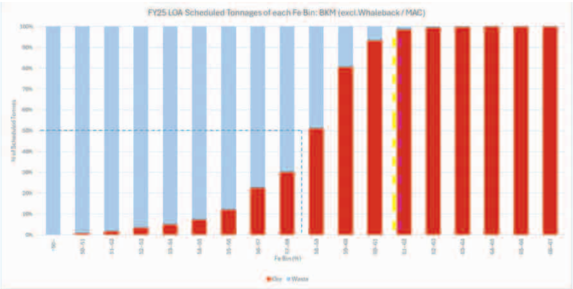
Figure 11-17: Ore vs Waste Contribution per Fe bin (normalised to 100%) for BKM material type
