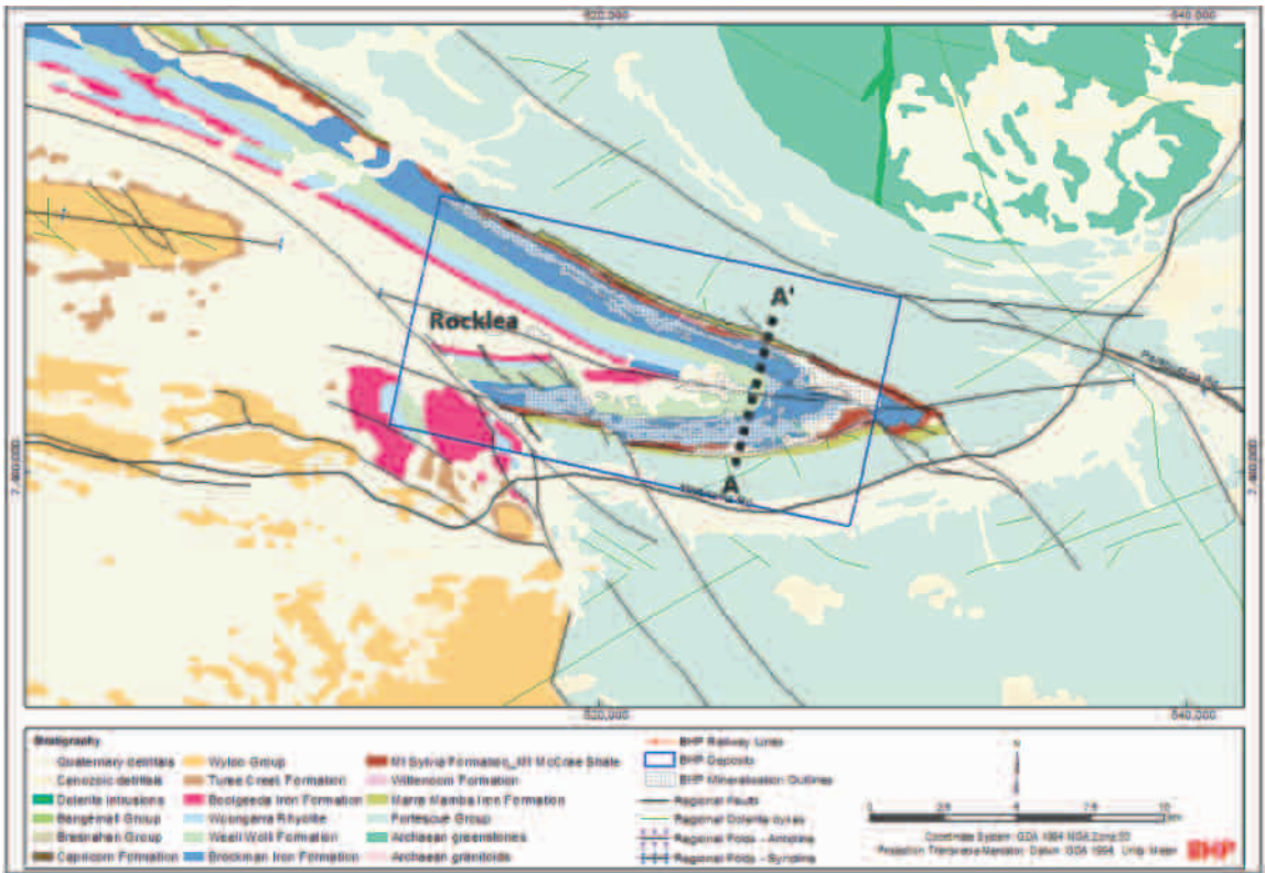
Figure 6-26: Geological Map of Rocklea (including approximate location of deposit cross-sections)
