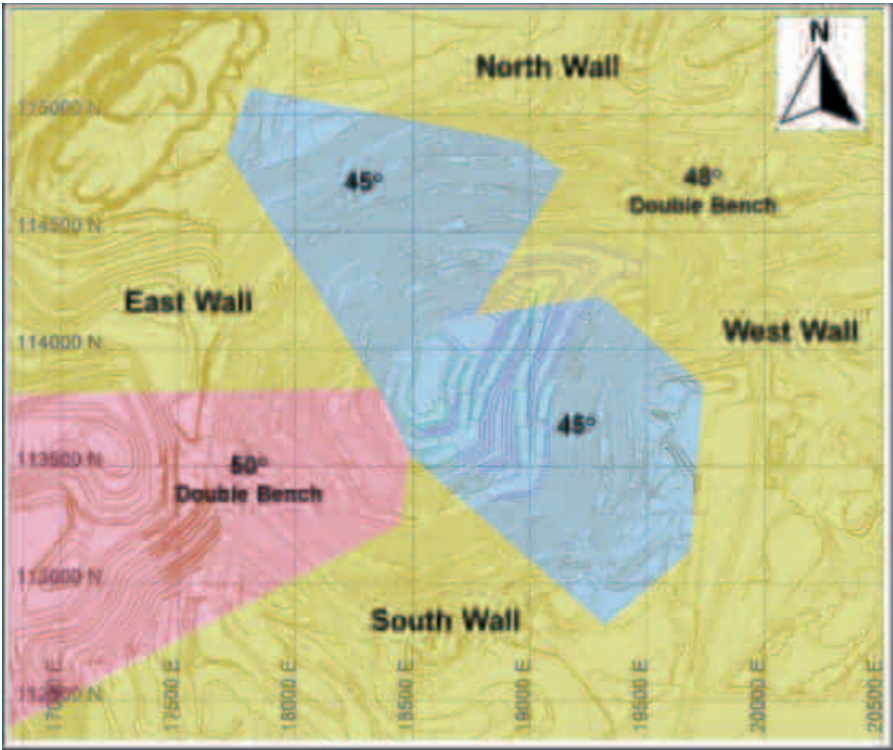
Figure 13-3: Escondida Pit Operational IRA (ToR 23)
