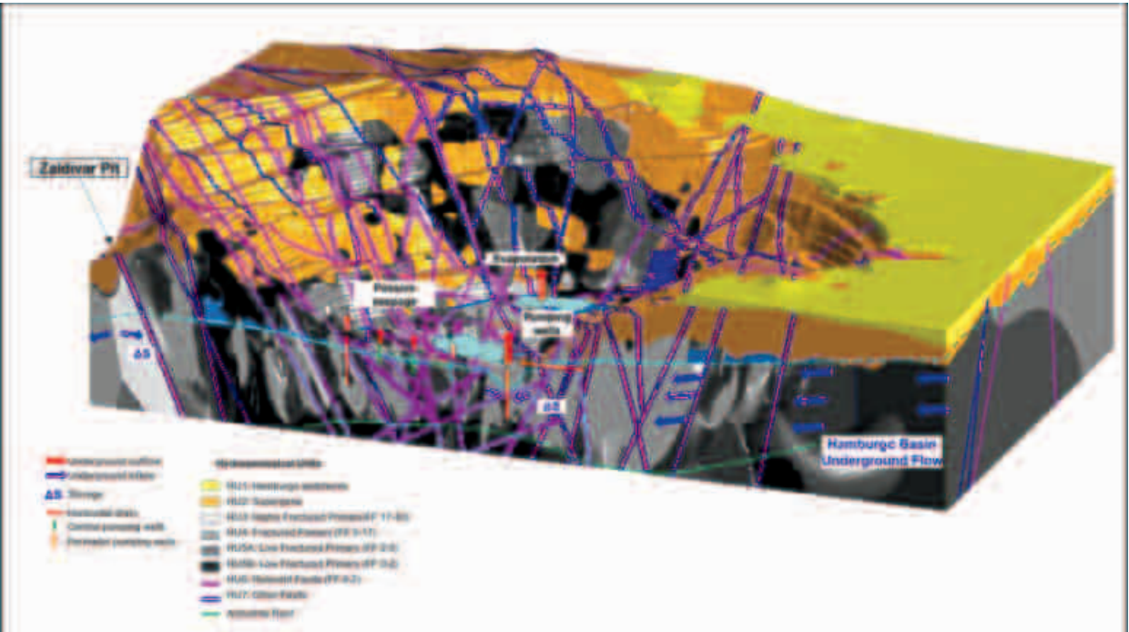
Figure 13-8: Escondida Norte Hydrogeological Model
