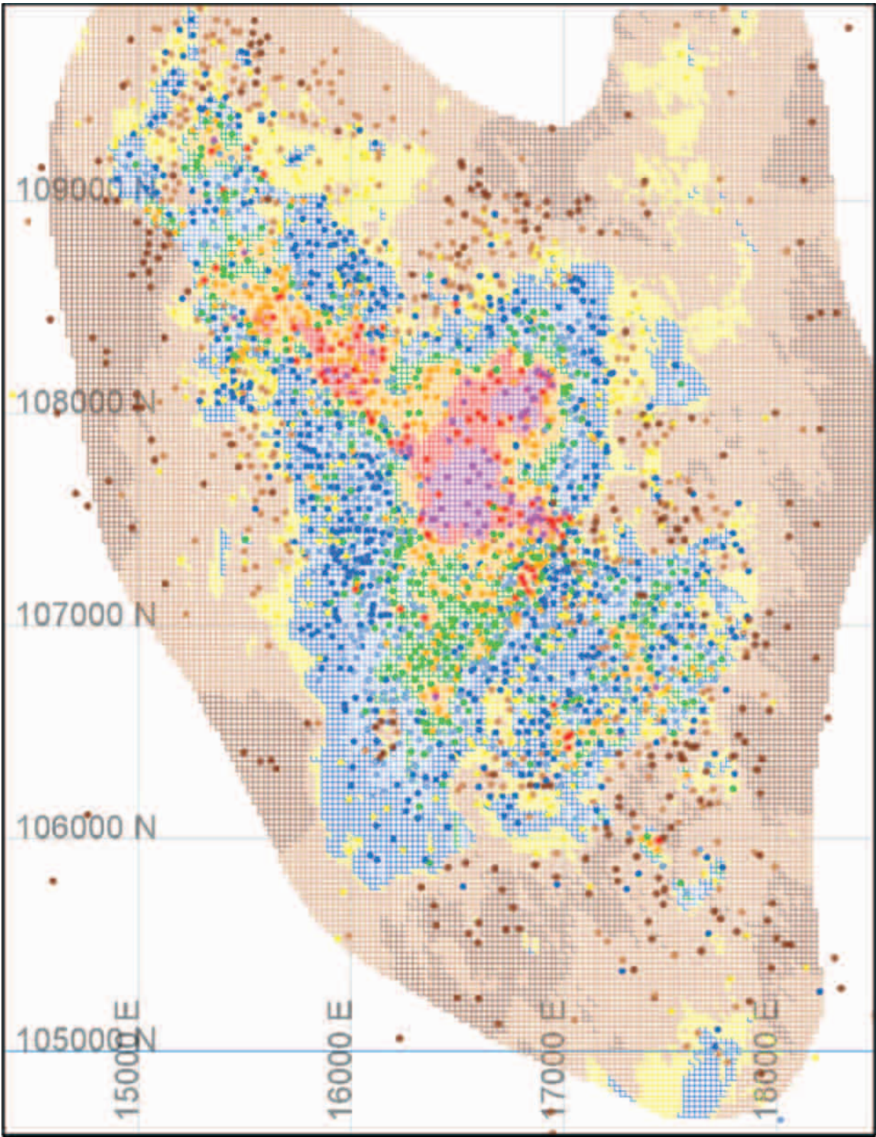
Figure 11-13: Escondida Copper at 2770 RL
