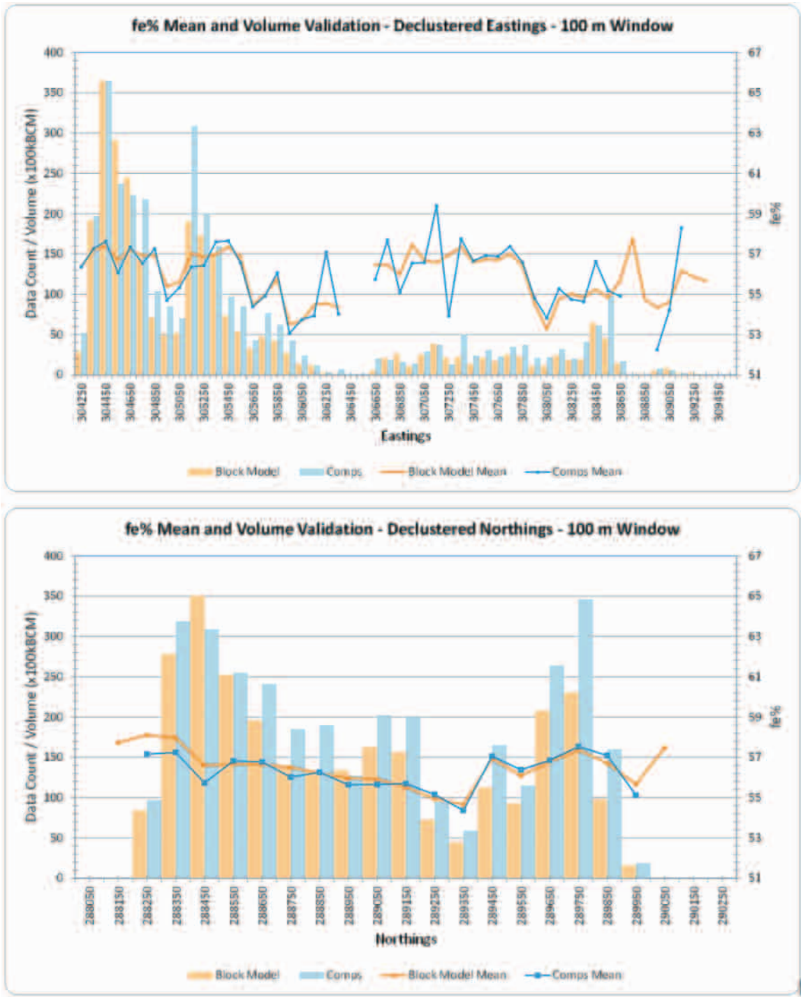
Figure 11-12: Illustration of Typical Swath Plots allowing for a spatial comparison between estimated block and composite mean grades
