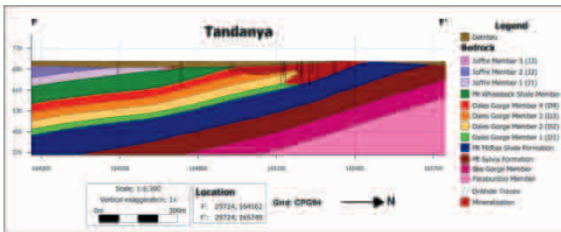
Figure 6-21: Geological Cross-section F-F' through Tandanya (a BKM deposit)
