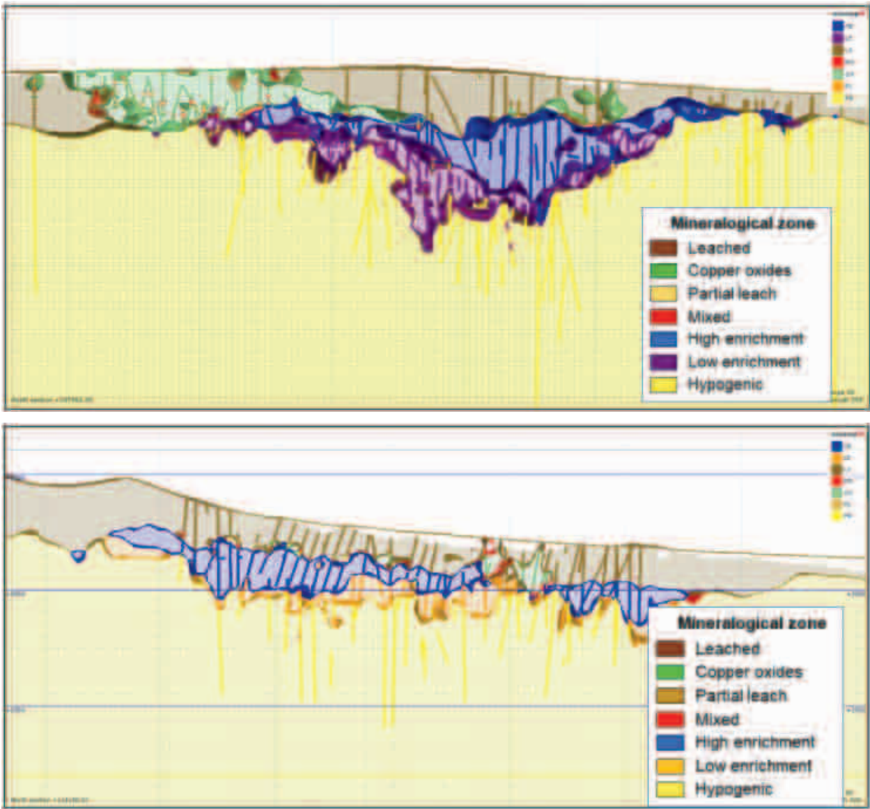
Figure 11-3: Examples of the Mineralogical Zones Cross-Sections for Escondida Section 107,550 (top) an Escondida Norte Section 114,150N (bottom)
