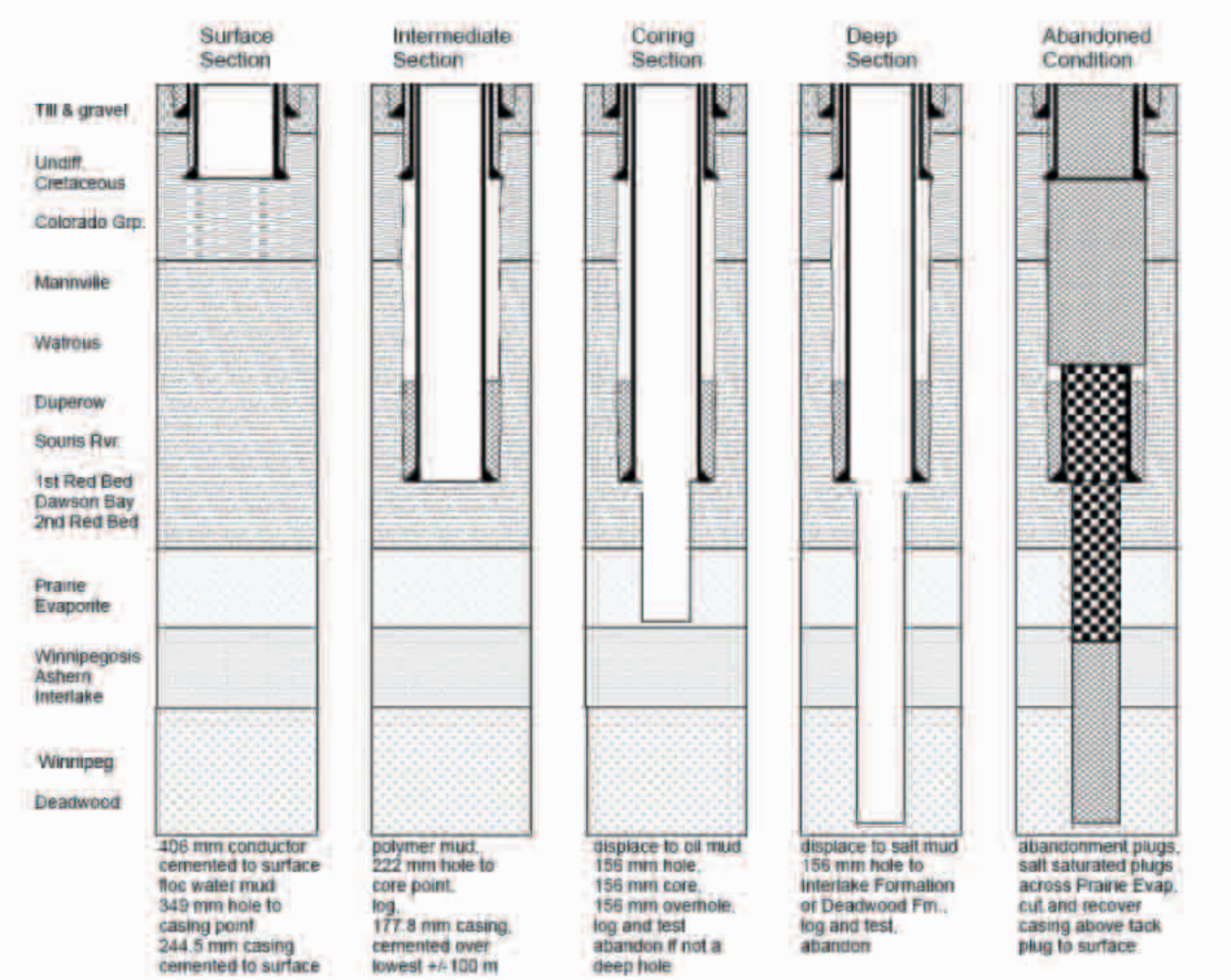
Figure 7-4: The four sections of the exploration drilling program and abandonment procedures.
