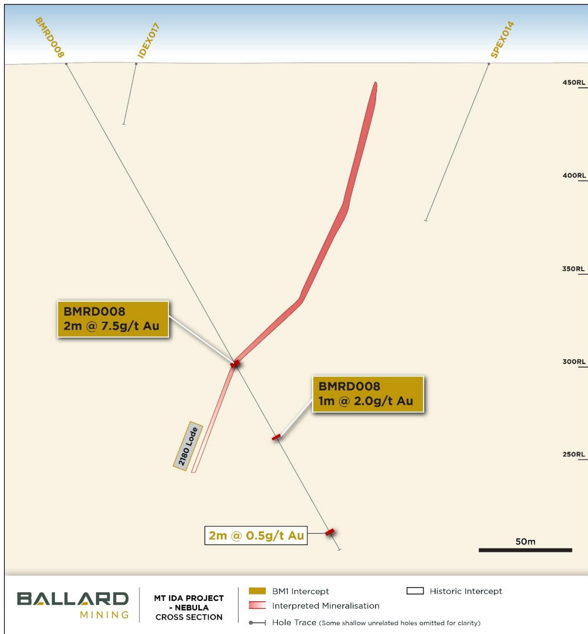
Figure 10 -Cross section 1 showing high grade assays results below the existing Mineral Resource in lode 2180 in the northern part of the Baldock system (Nebula) 200 metres north of cross section 2.
