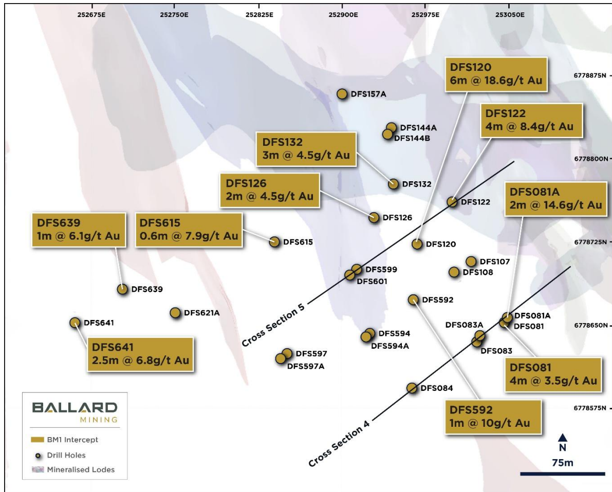
Figure 3 – Selected final infill assay results from Baldock
