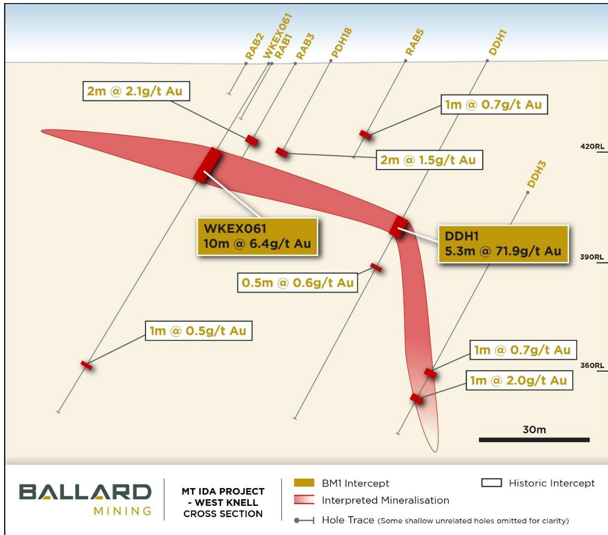
Figure 12 - Cross section through West Knell showing shallow high grade intervals, possibly supergene mineralisation
