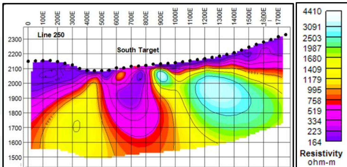
Figure 2: CSAMT L250 resistivity section over the Southern Target
