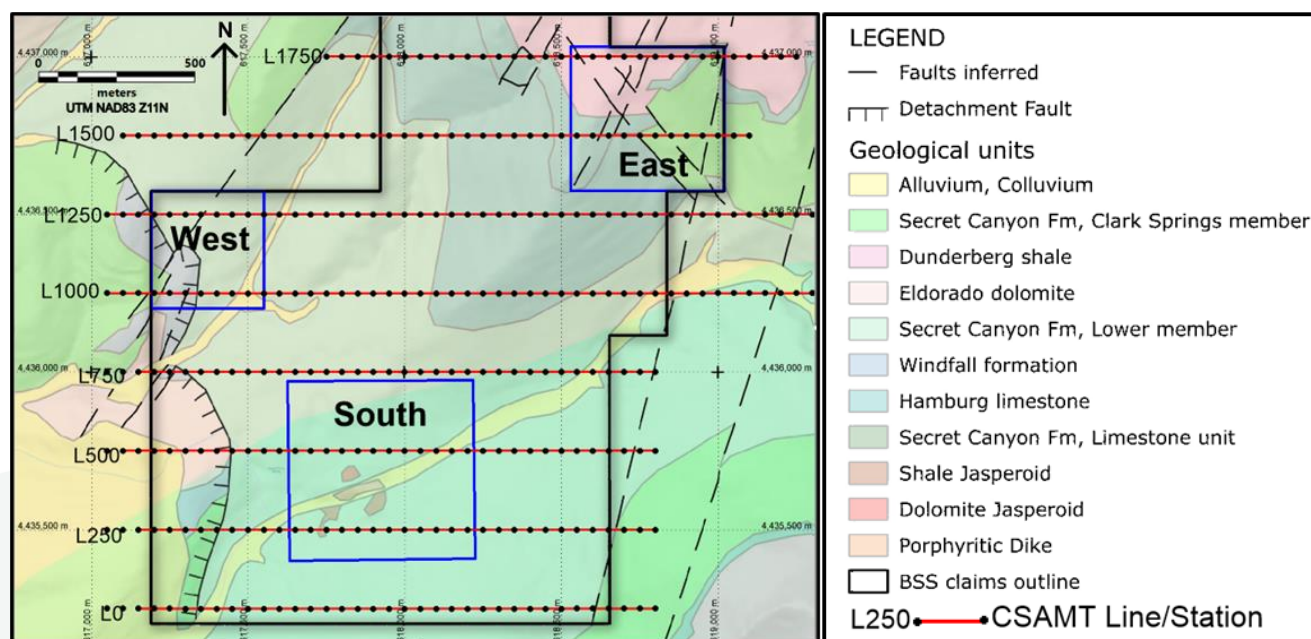
Figure 1: Position of CSAMT survey profile lines and defined target over detail geological map
