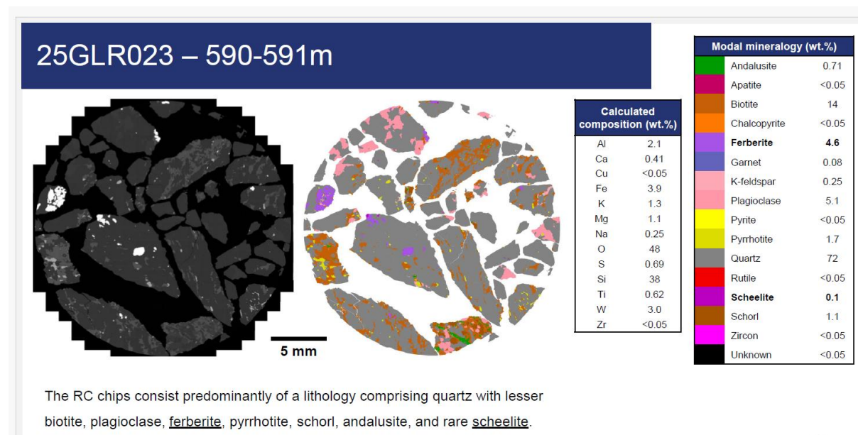
Figure 6 Coarse ferberite confirmed in SEM analysis (iron rich wolframite). RC sample returned 1.25% \text{WO}_3 .
