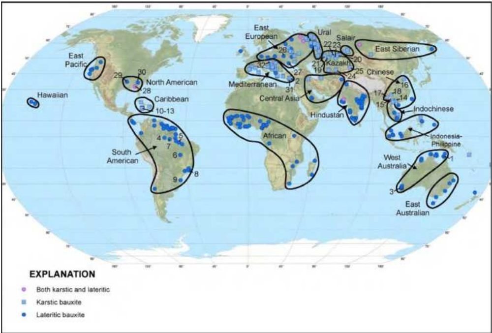
Figure 3-1: Distribution of world bauxite deposits
