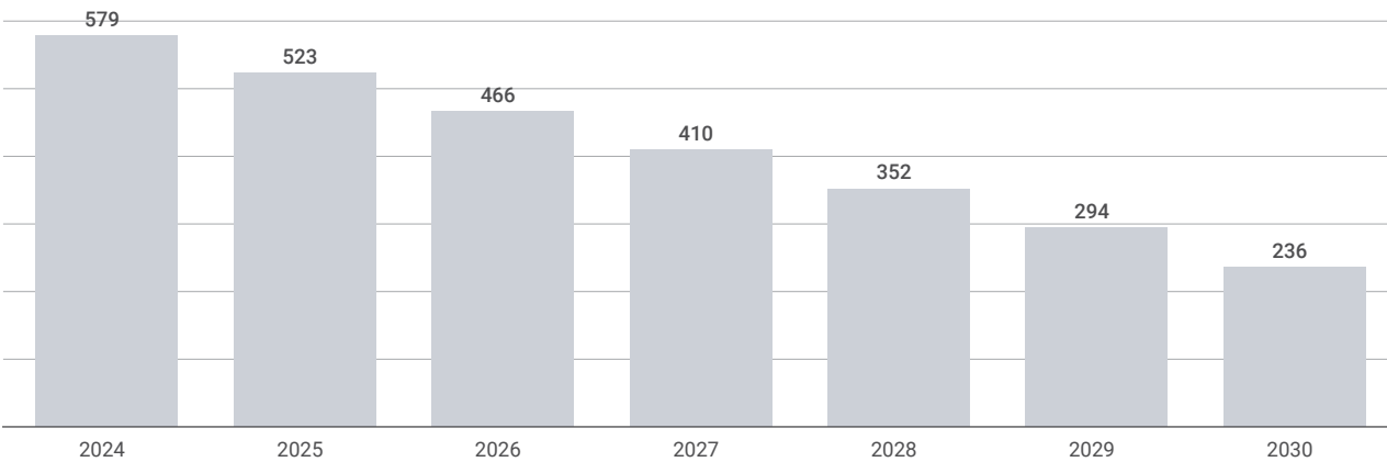
Figure 2: China bauxite reserves – forecast (millions of tonnes) 1
