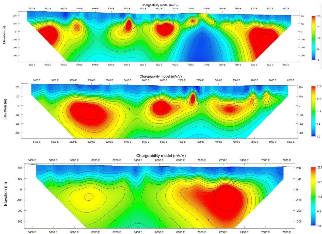
Figure 3. Chargeability sections 12350N, 12850N and 13100N showing 25 mV/V chargeability features.
