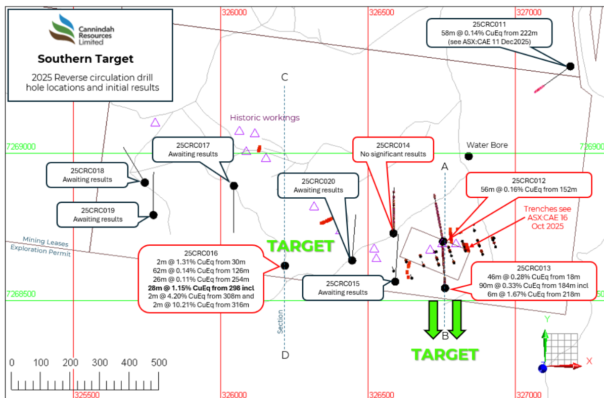
Figure 7: Location of Southern Porphyry Target drill holes and results
