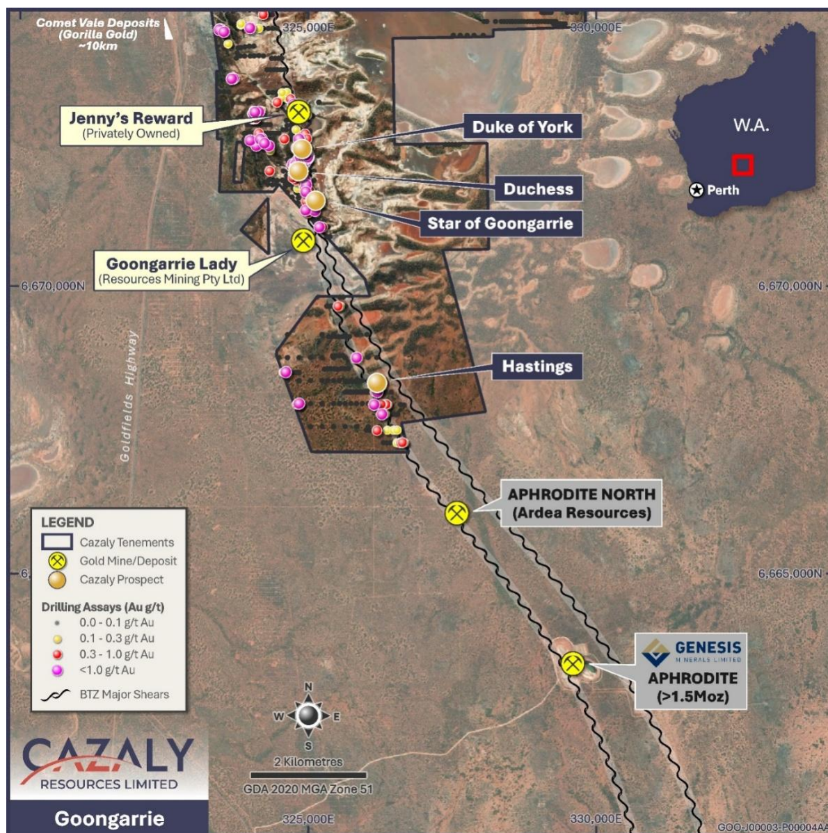
Figure 3. Location of the Hasting gold prospect along the Bardoc Tectonic Zone.
