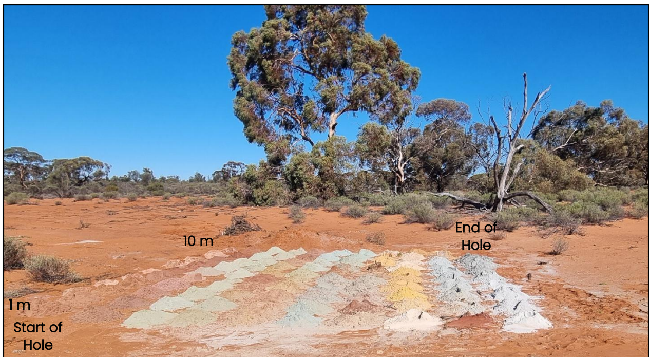
Figure 2. GGAC0356 1m drill spoil laid out in rows of 10 from left front to right back.
