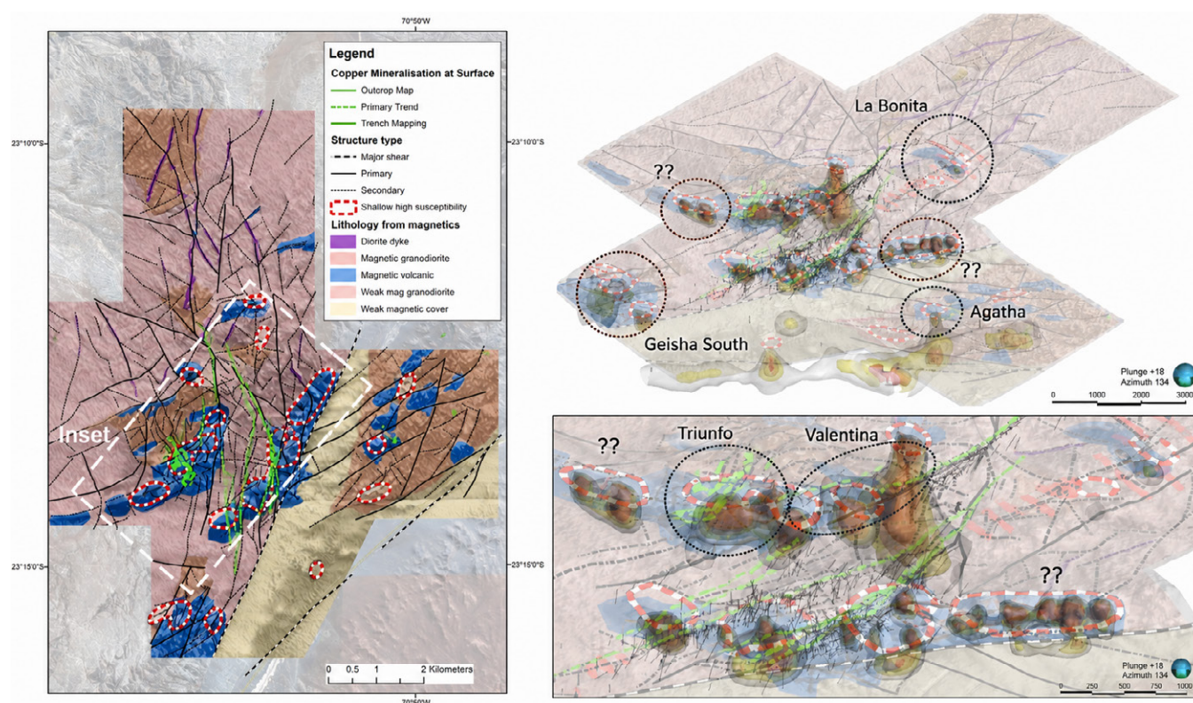
Figure 13 | Drone magnetic interpretation on first vertical derivative magnetic background. Isoshells of high magnetic units are displayed in the 3D images in the right-hand panels. Results highlight both the structural pathways to mineralisation as well as magnetic sources which appear to control higher-grades and provide a key targeting criteria.
