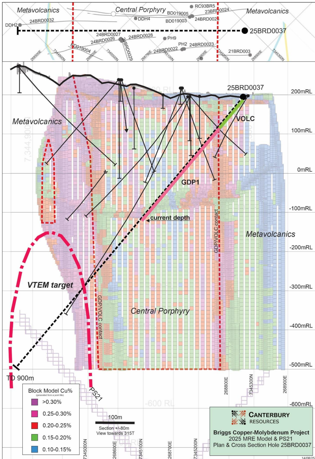
Figure 2 Cross-section view along the trace of hole 25BRD0037 showing block model grade distribution from the 2025 MRE and an outline of the VTEM target.
