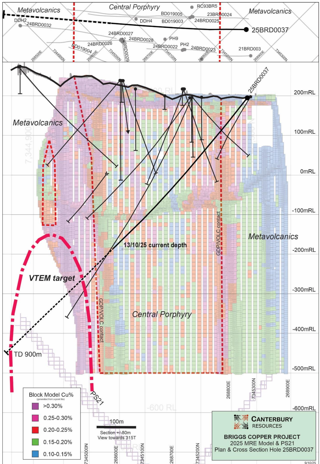
Figure 4 Plan & cross-section of Briggs displaying progress of the 900m deep hole (25BRD0037), historical drilling (projected \pm 80\text{m} ) plus the MRE block model
