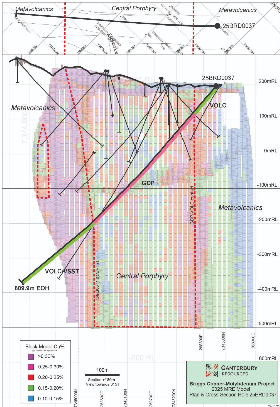
Figure 2 Cross Section showing down-hole geology in 25BRD0037 and the copper grades from the MRE block model estimate.
