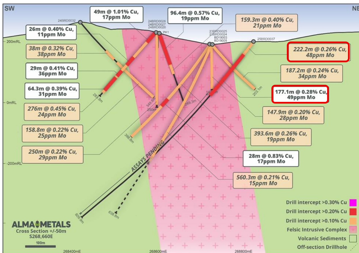
Figure 2 Cross Section showing down-hole geology in 25BRD0037 and the assays for the top 231m of the hole (red label outline). For location refer to Figure 1.
