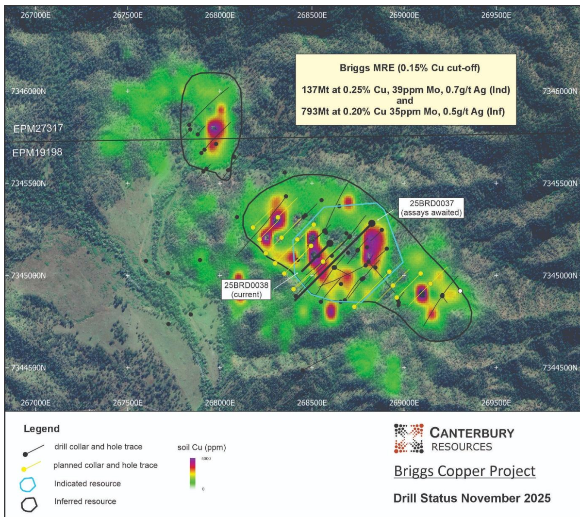
Figure 1 Plan view of the Briggs deposit showing the outline of the MRE, drill collars, the recently completed hole (25BRD0037) and the current hole (25BRD0038) on a background image of copper-in-soil mineralisation.
