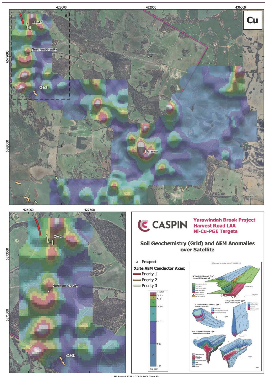
Figure 6. Copper-in-soil geochemistry.
