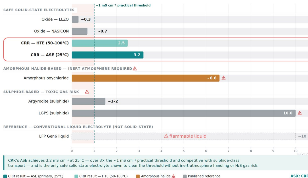
Figure 1 – Ionic conductivity comparison. Initial ASE results exceed the \sim 1 \text{ mS cm}^{-1} practical operation threshold without sulphide chemistry — with further improvement expected through ongoing formulation work. HTE = High Temperature Electrolyte
