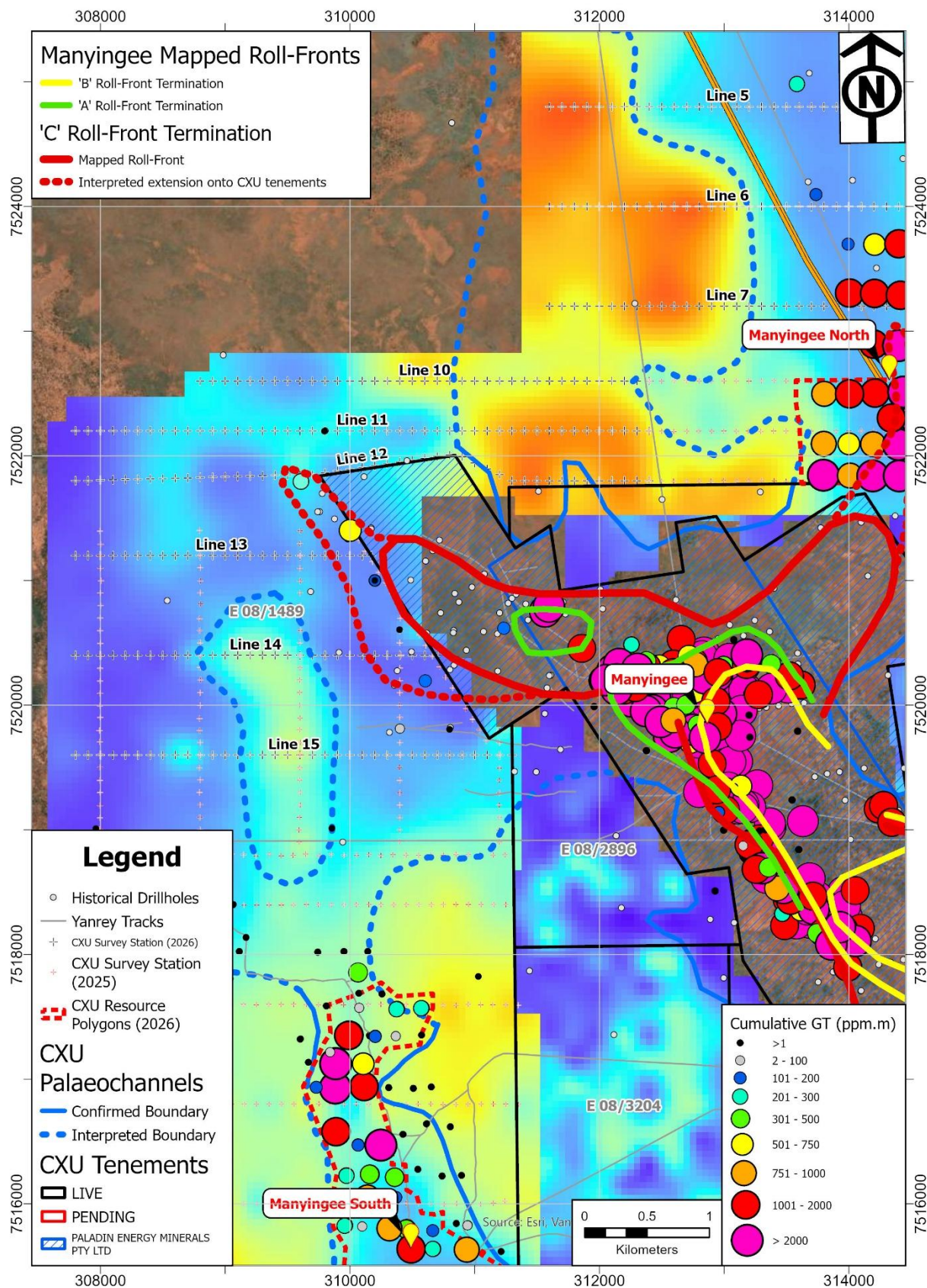
Figure 4. North Manyingee & Manyingee West passive seismic interpreted depth to bedrock. Roll-fronts mapped by Paladin Energy Ltd. Note the extension of the C roll-front onto Cauldron's E08/1489 where passive seismic shows that the channel is deeply incised.
