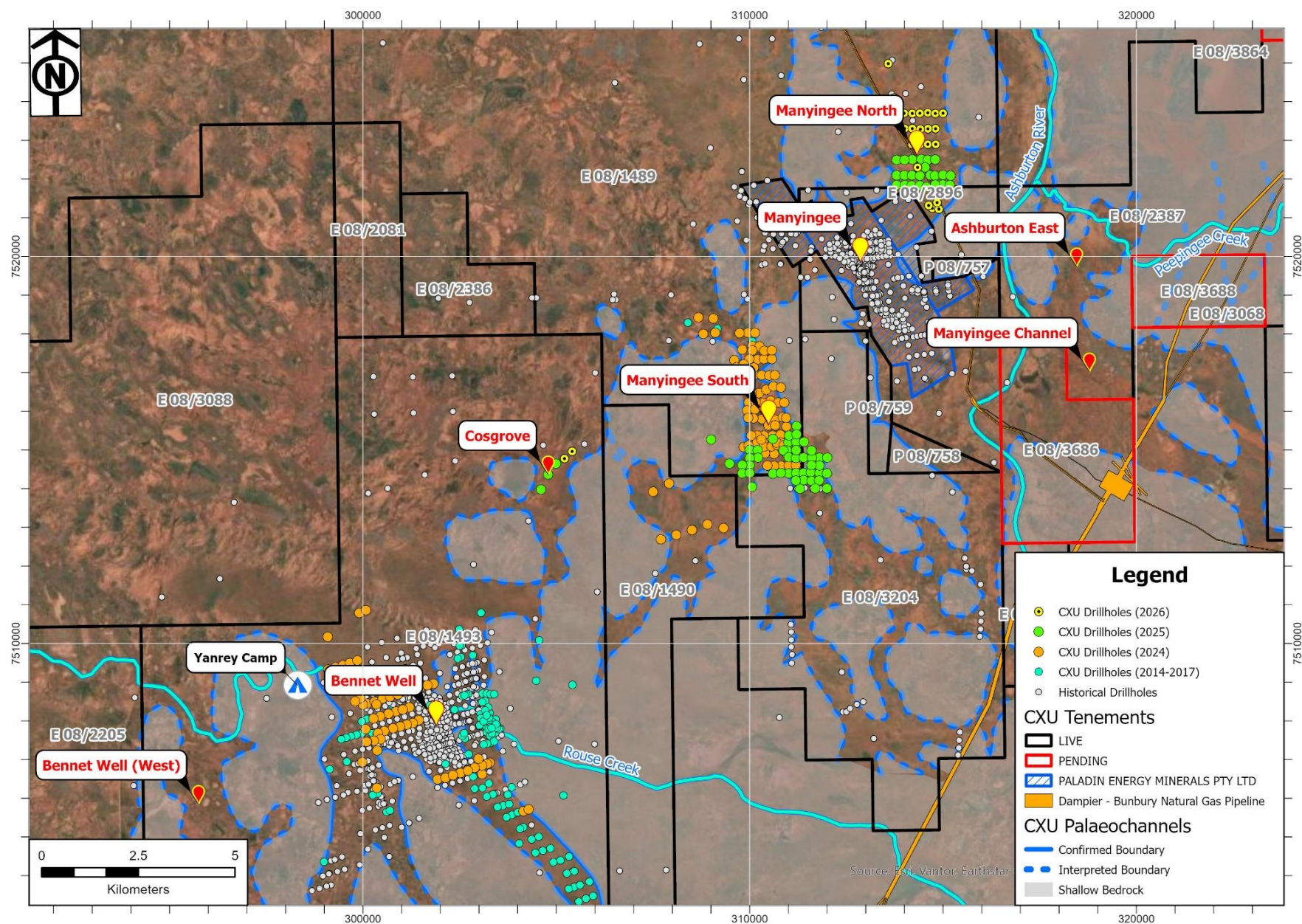
Figure 2. Map of the Yanrey region showing drilling and uranium deposits within the interpreted Early Cretaceous palaeodrainage network.
