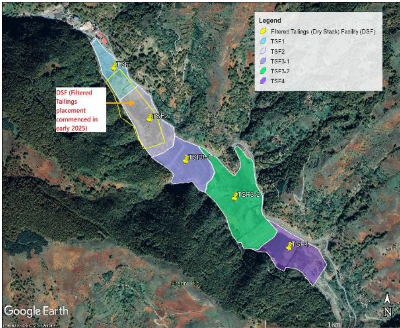
Figure 3.9 Sasa Mine TSF Outline
