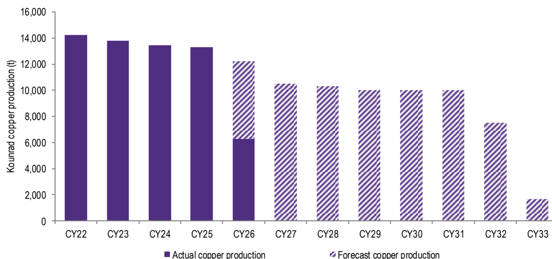
Figure 98 - Kounrad production profile
