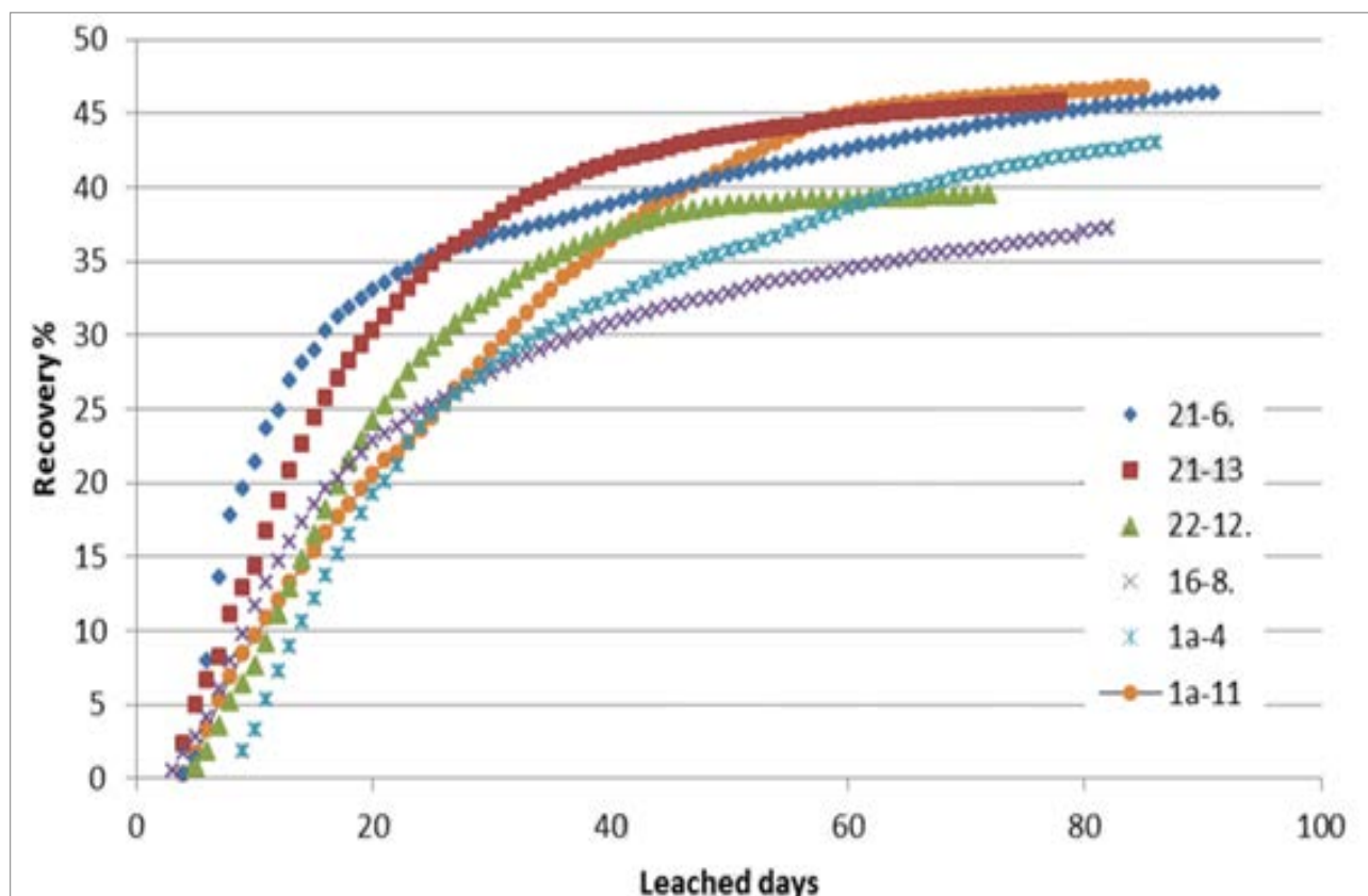
Figure 3.13 Western Dumps Column Test Results
