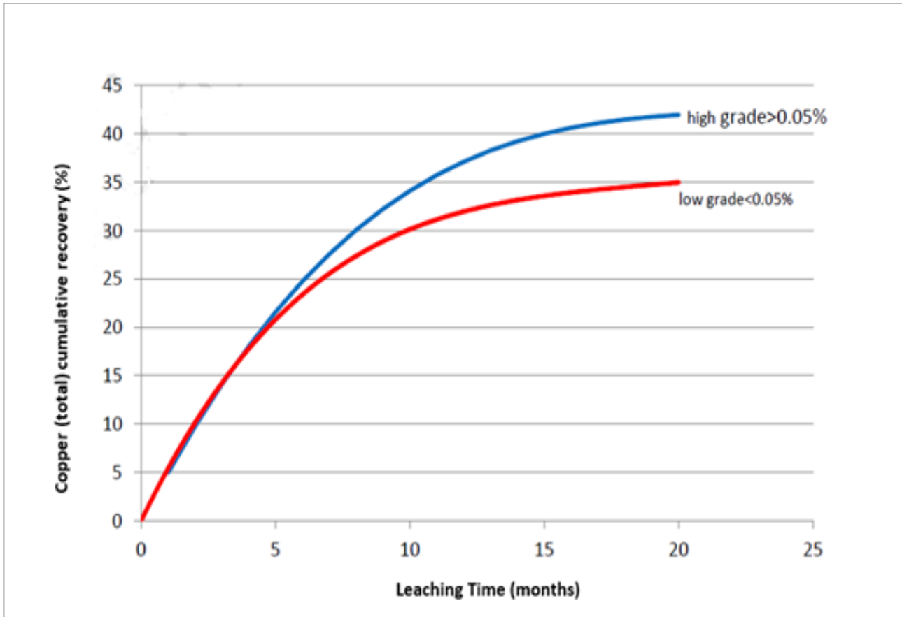
Figure 3.14 Western Dumps Leach Design Recovery Curves
