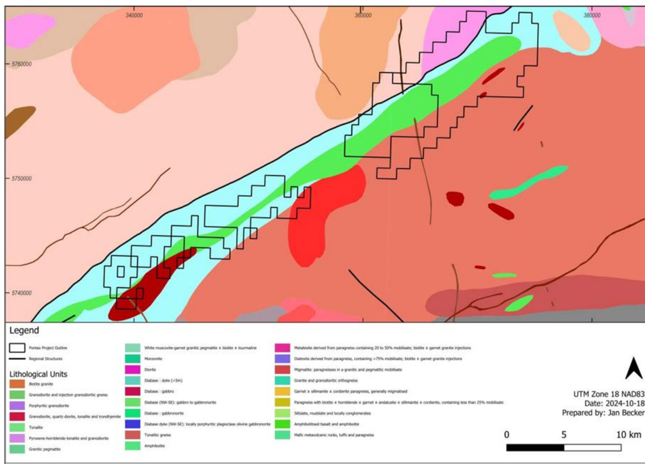
Figure 2.11 Geology plan for Pontax
