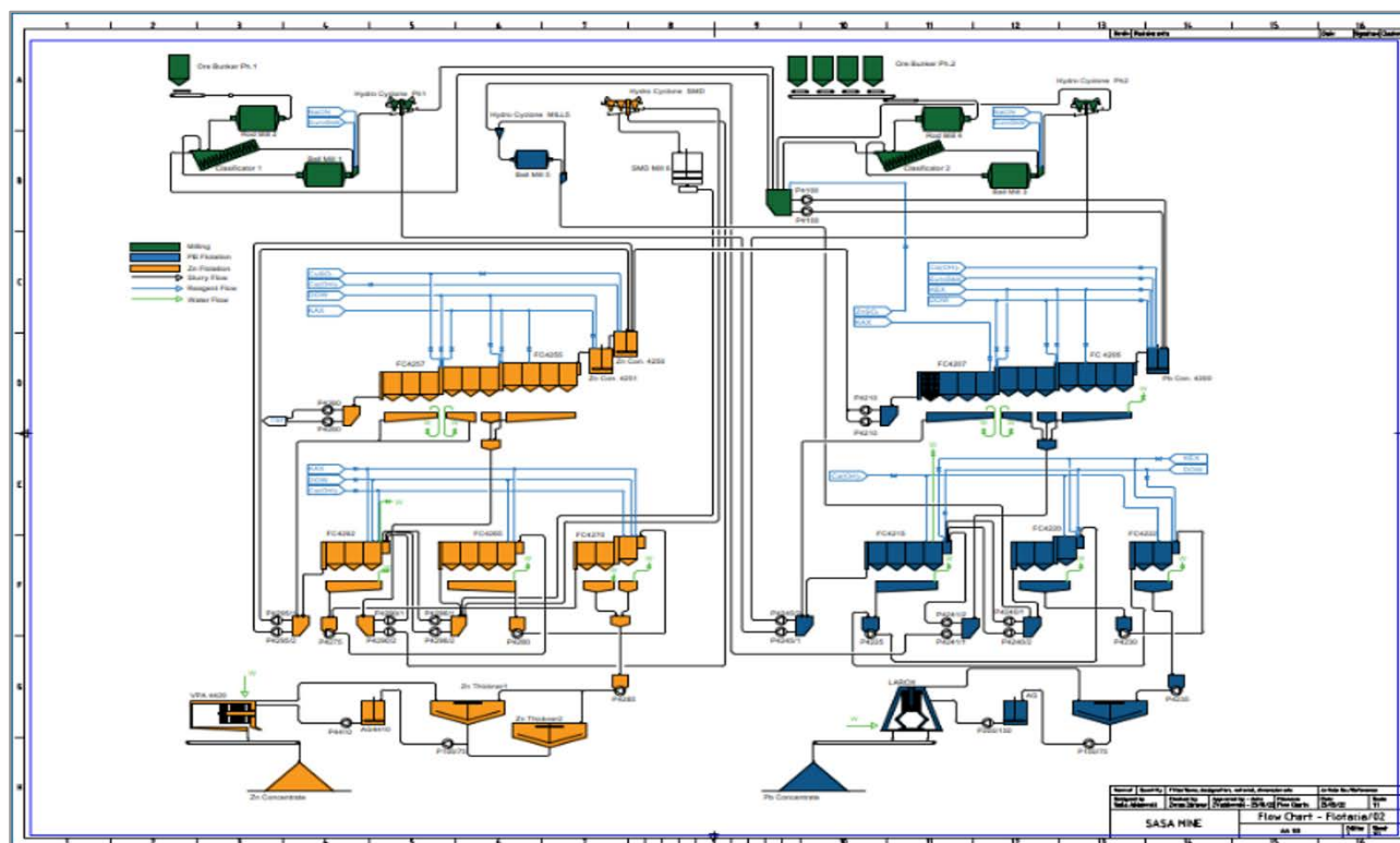
Figure 3.8 Flowsheet for the Sasa Processing Plant
