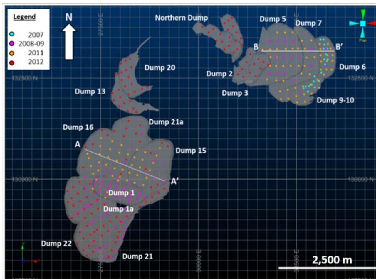
Figure 3.12 Waste dump drillhole locations
