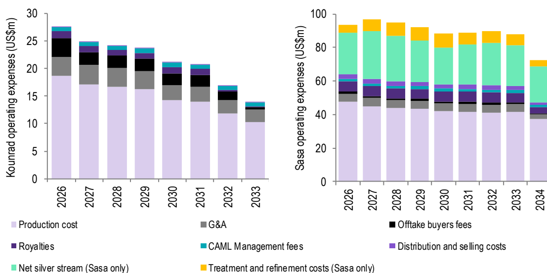
Figure 100 - Operating costs for the Kounrad (LHS) and Sasa (RHS) Projects
