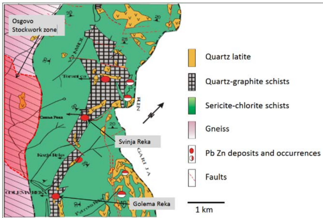
Figure 3.4 Sasa deposit geology
