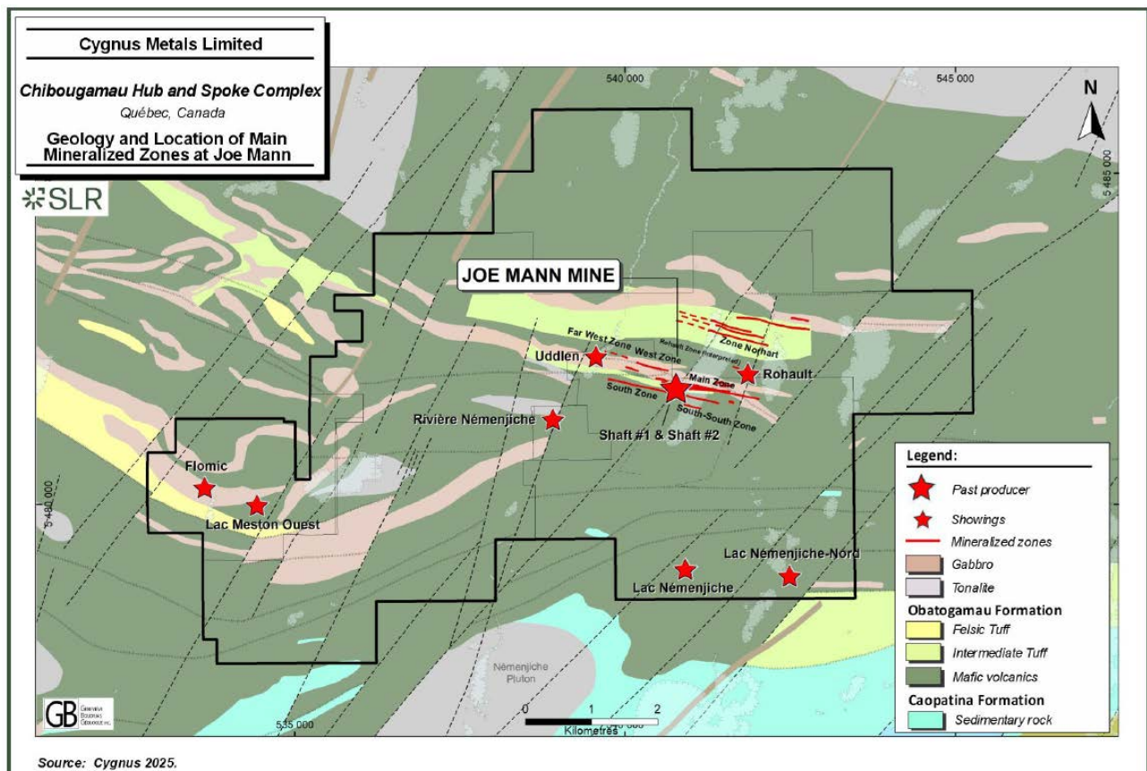
Figure 2.10 Joe Mann and Devlin geology
