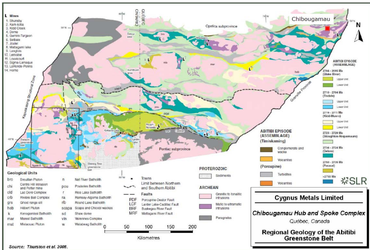
Figure 2.7 AGB geology
