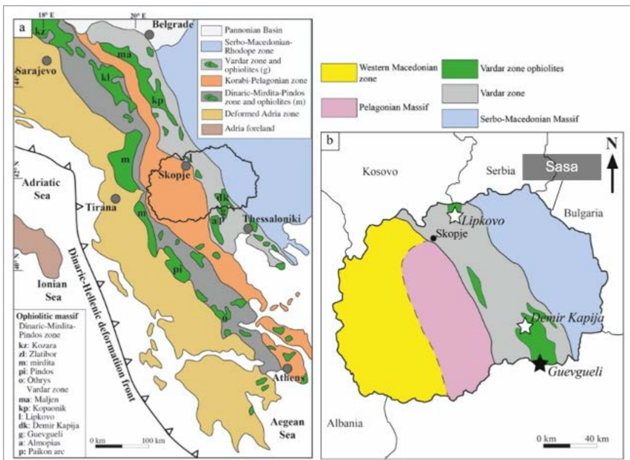
Figure 3.3 Sasa regional geology
