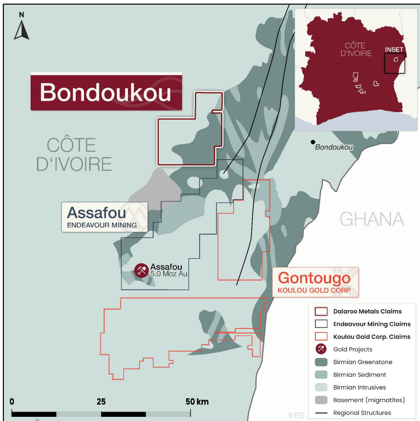
Figure 6. Location of Dalaroo Bondoukou Gold Project with Relevant neighbouring licences. Regional geological map showing Dalaroo's Côte d'Ivoire project portfolio within the Birman Greenstone Belt relative to neighbouring mining projects.
