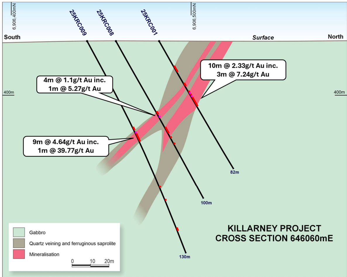
Figure 3: Cross Section 646060E, Killarney Project
