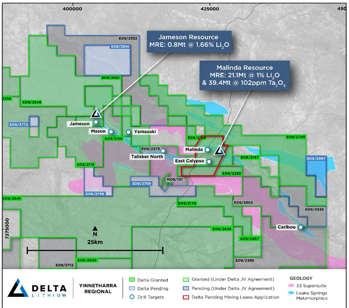
Figure 4: Plan View to Yinnetharra MRE's and drill targets for current exploration programs
