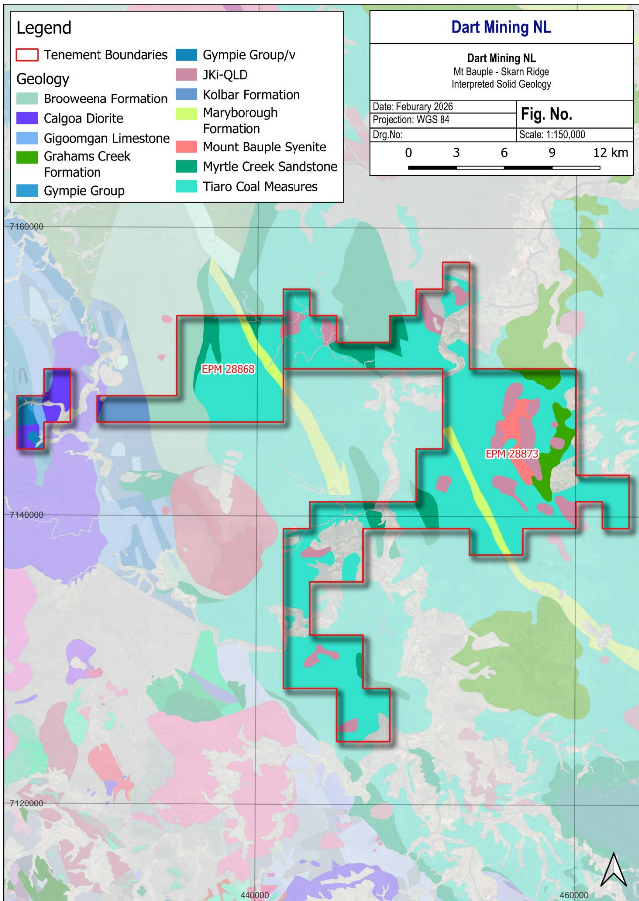
Figure 2 : EPM 28868 and 28873 Interpreted Solid Geology.
