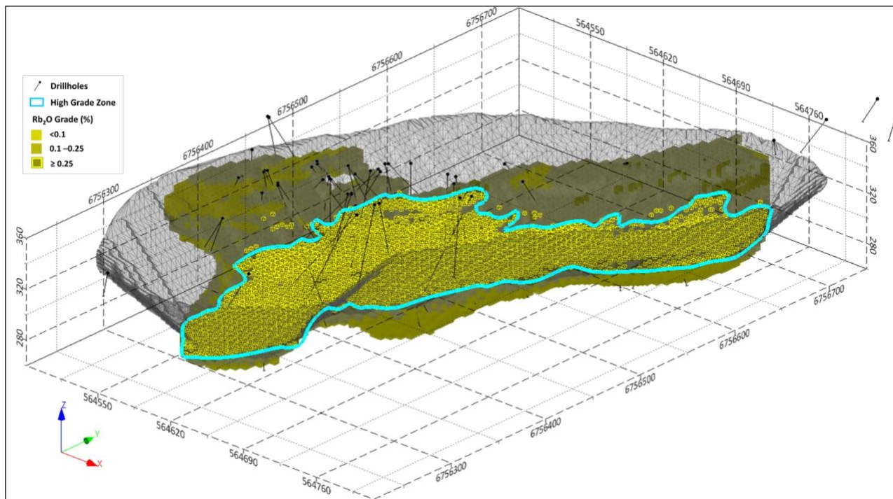
Figure 2: Oblique northwest-looking view of the Mt Edon MRE, highlighting the high-grade subset of the Mineral Resource
