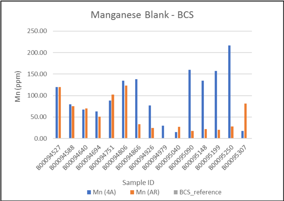
Figure 11-25: Certified Blank – BCS-CRM-531 – Manganese Source: Tetra Tech (2022)
