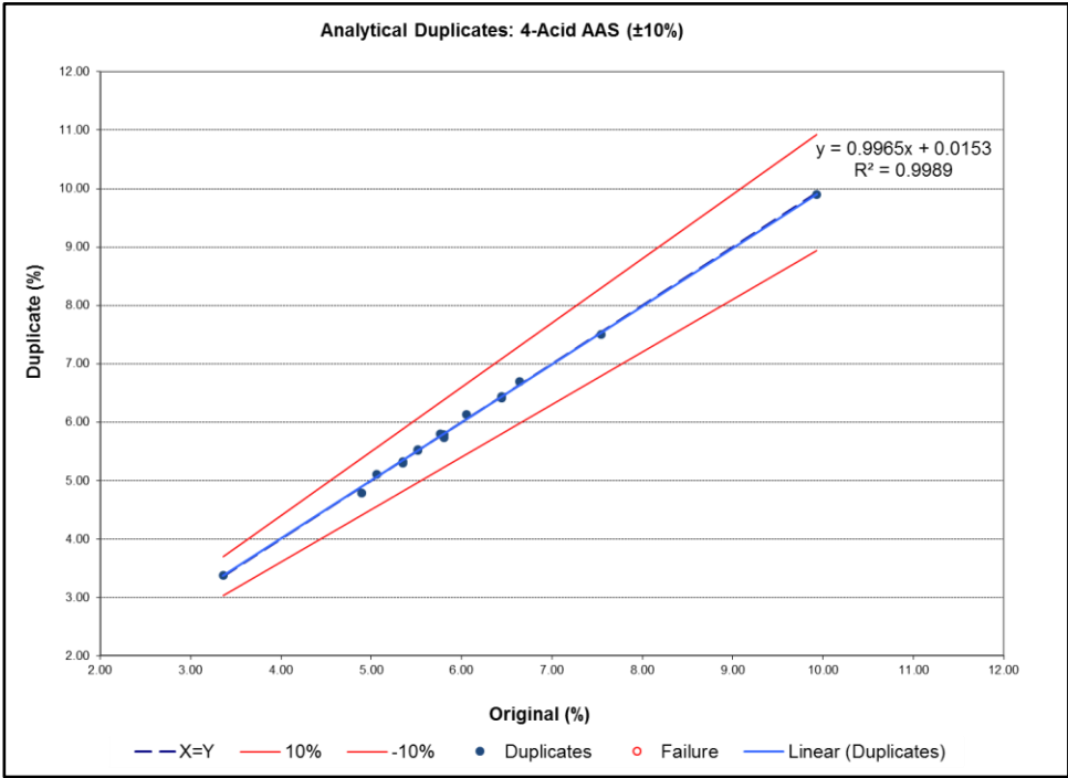
Figure 11-35: Linear Regression of 4-Acid AAS Manganese Analytical Duplicates Source: Tetra Tech (2022)
