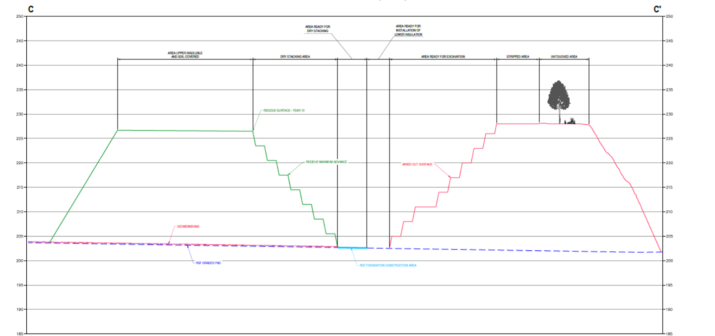
Figure 16-13: Tailings Extraction and Residue Development Section C-C'
