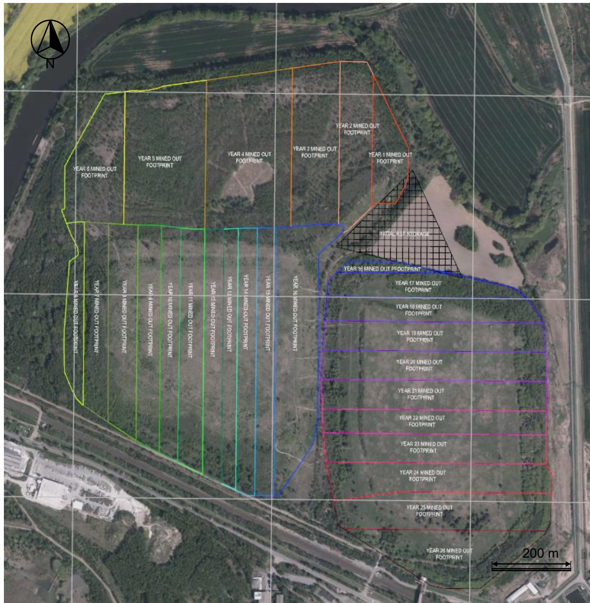
Figure 16-8: Plan View of Annual Mined-Out Footprint
