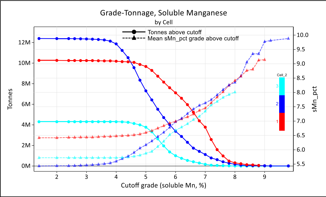
Figure 14-16: Grade-tonnage Curve for the Chvaletice Manganese Project, Soluble Manganese Source: Tetra Tech (2022)
