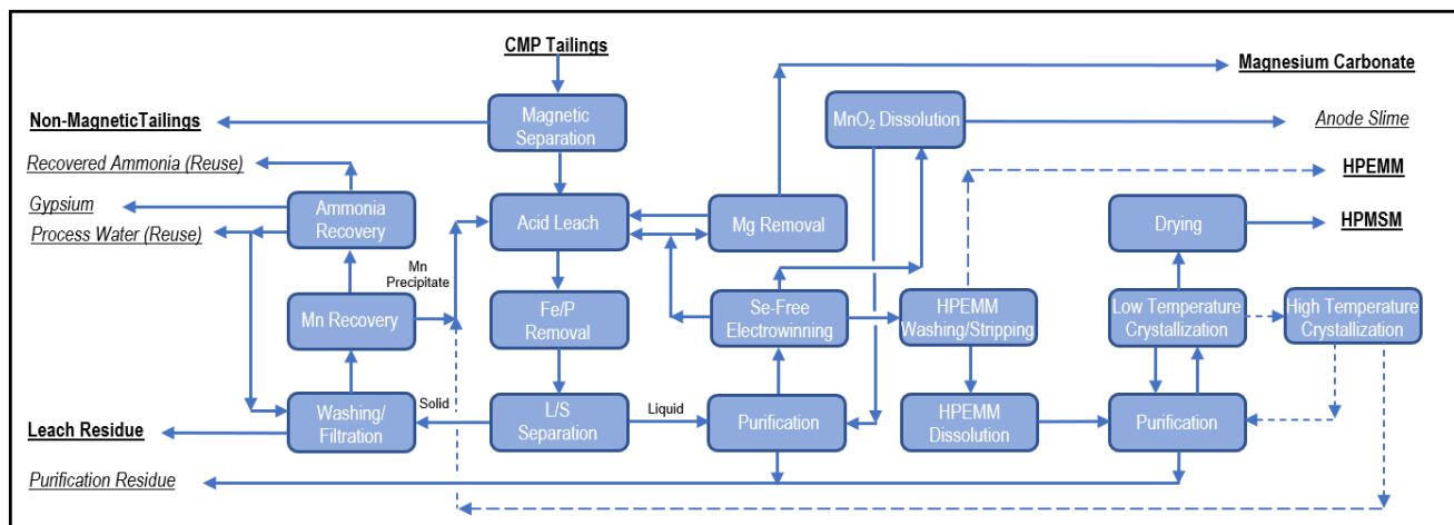
Figure 17-1: Simplified Process Flowsheet
