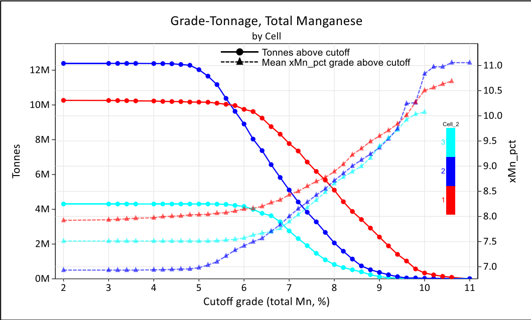
Figure 14-15: Grade-tonnage Curve for the Chvaletice Manganese Project, Total Manganese Source: Tetra Tech (2022)
