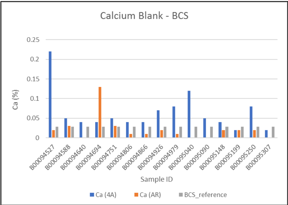
Figure 11-26: Certified Blank – BCS-ST-531 – Calcium Source: Tetra Tech (2022)
