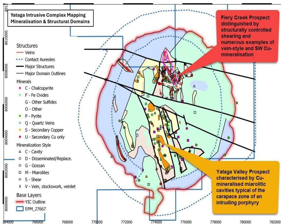
Figure 1 – Yataga Project Showing both Fiery Creek and Yataga Valley Prospects
