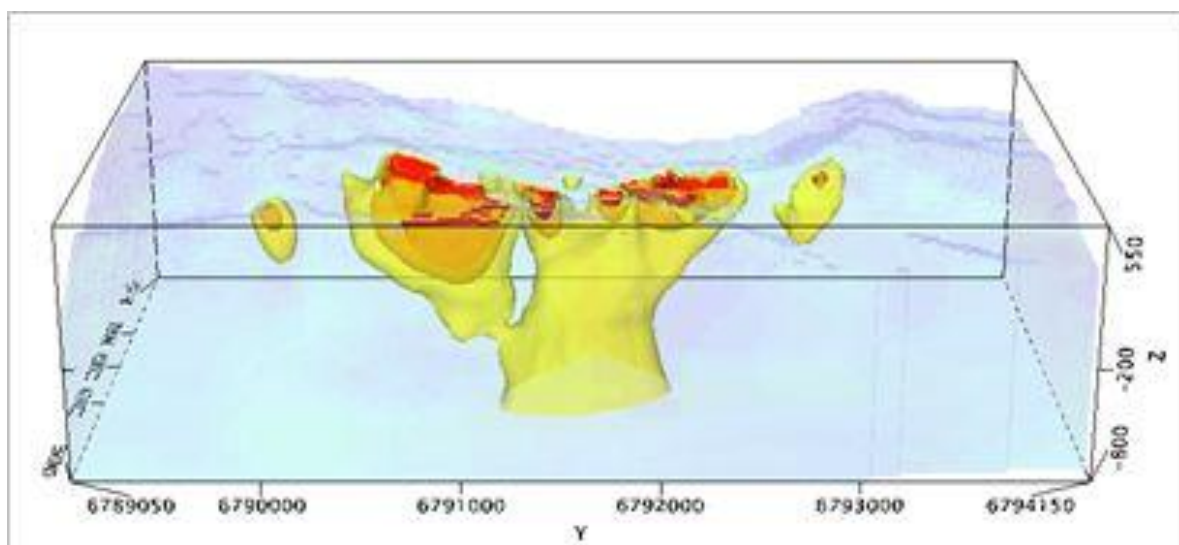
Figure 9: 3D inversion of DIGHEM magnetic data. Isosurfaces: red – 0.15 orange 0.13 yellow 0.11 SI
