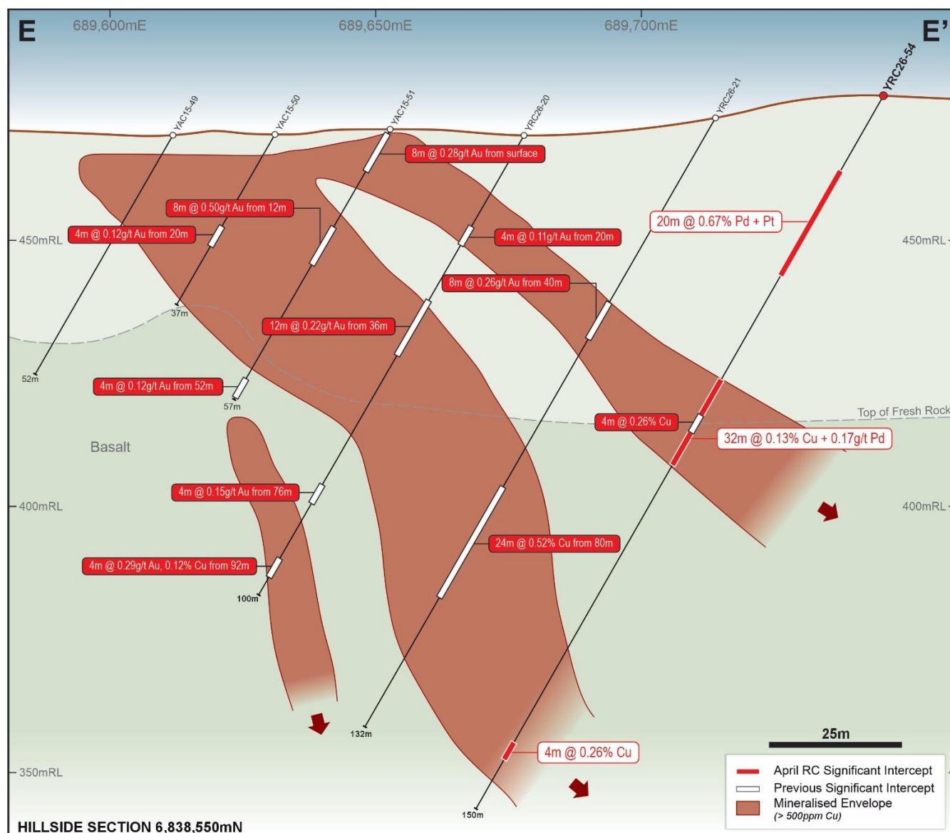
Figure 6. Hillside Cross Section 6,838,550mN
