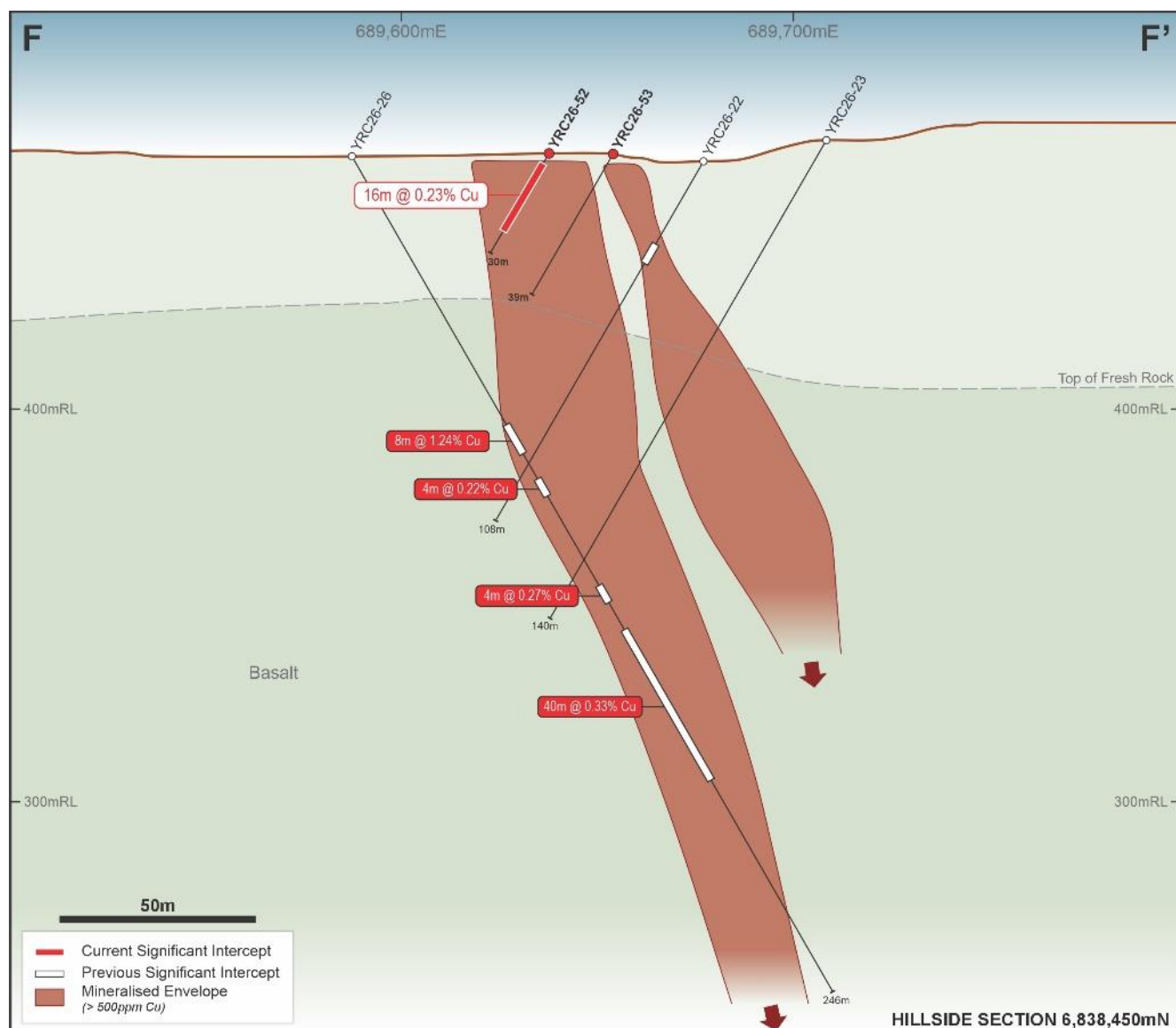
Figure 7. Hillside Cross Section 6,838,450mN
