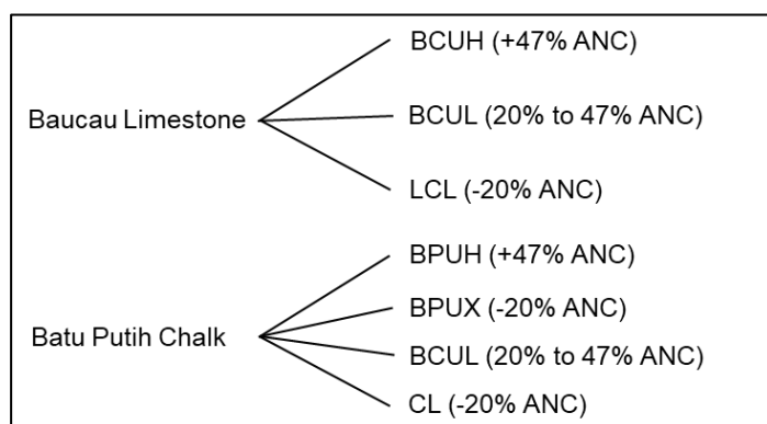
Figure 4.3 – Interpreted Horizons
