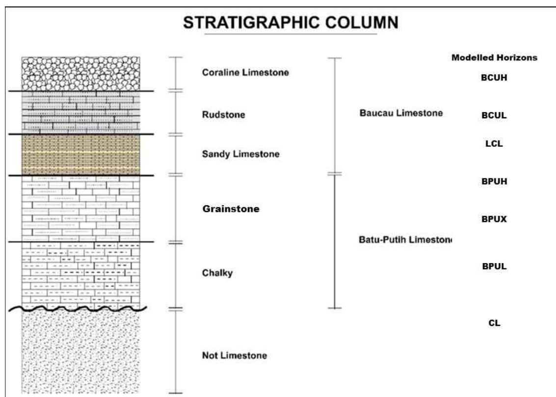
Figure 4.1 – Stratigraphic Column
